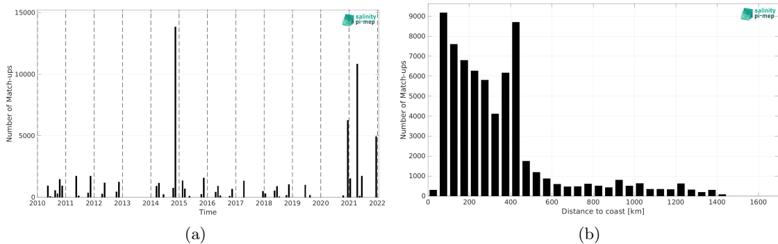
Figure 1: Number of match-ups between TSG (Polarstern) and CCI SSS L4 Merged-OI v4.4 - 30-day running (ESA) SSS as a function of time (a) and as function of the distance to coast (b) over the North Atlantic Ocean Pi-MEP region and for the full satellite product period.
