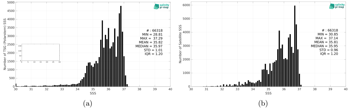
Figure 2: Histograms of SSS from TSG (Polarstern) (a) and CCI SSS L4 Merged-OI v4.4 - 30-day running (ESA) (b) considering all match-up pairs per bins of 0.1 over the North Atlantic Ocean Pi-MEP region and for the full satellite product period.
