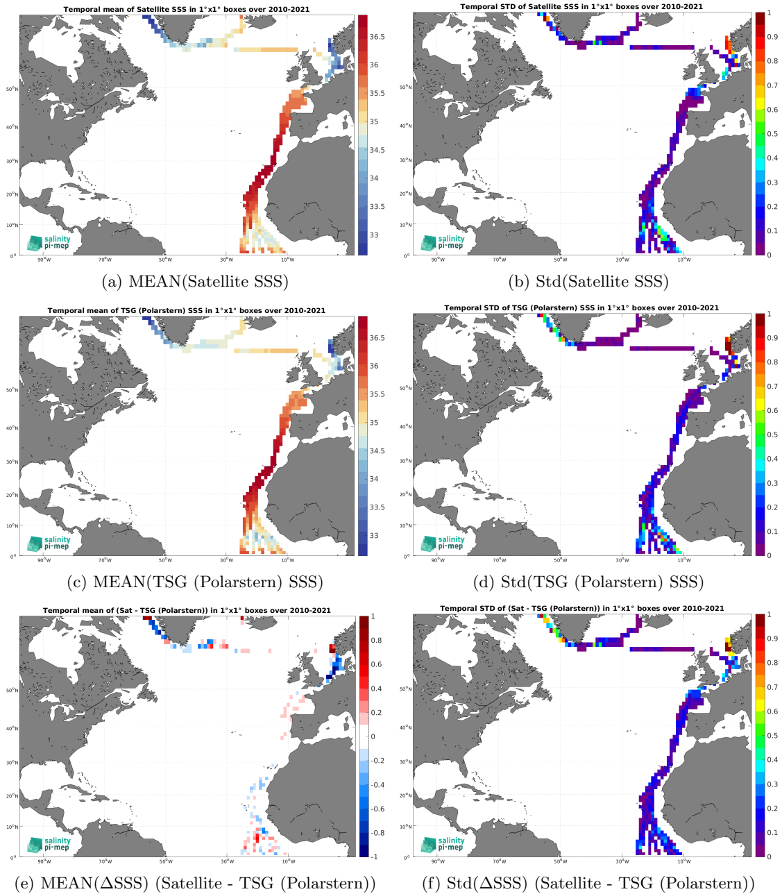
Figure 6: Temporal mean (left) and Std (right) of SSS from CCI SSS L4 Merged-OI v4.4 - 30-day running (ESA) (top), TSG (Polarstern) (middle), and of \Delta SSS (Satellite - TSG (Polarstern)). Only match-up pairs are used to generate these maps.
