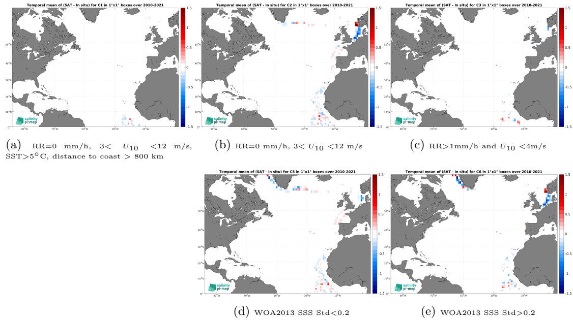
Figure 12: Temporal mean gridded over spatial boxes of size 1^\circ \times 1^\circ of \Delta\text{SSS} (CCI SSS L4 Merged-OI v4.4 - 30-day running (ESA) - TSG (Polarstern)) for 5 different subdatasets corresponding to:RR=0 mm/h, 3 < U_{10} < 12 m/s, SST >5^\circ\text{C} , distance to coast > 800 km (a), RR=0 mm/h, 3 < U_{10} < 12 m/s (b), RR >1 mm/h and U_{10} < 4 m/s (c), WOA2013 SSS Std <0.2 (d), WOA2013 SSS Std >0.2 (e).
