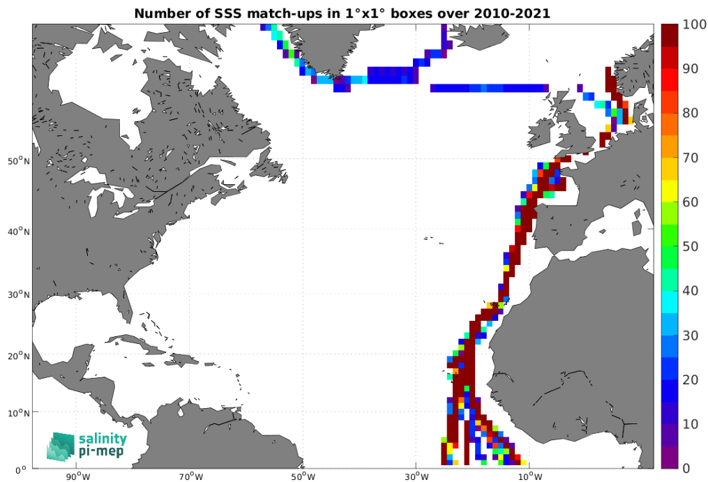
Figure 4: Number of SSS match-ups between TSG (Polarstern) SSS and the CCI SSS L4 Merged-OI v4.4 - 30-day running (ESA) SSS product for the North Atlantic Ocean Pi-MEP region over 1^\circ \times 1^\circ boxes and for the full satellite product period.
