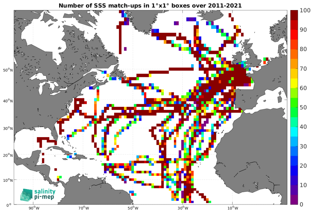
Figure 4: Number of SSS match-ups between TSG (GOSUD-Sailing-ship) SSS and the CCI SSS L4 Merged-OI v4.4 - 30-day running (ESA) SSS product for the North Atlantic Ocean Pi-MEP region over 1^\circ \times 1^\circ boxes and for the full satellite product period.
