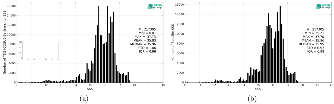
Figure 2: Histograms of SSS from TSG (GOSUD-Sailing-ship) (a) and CCI SSS L4 Merged-OI v4.4 - 30-day running (ESA) (b) considering all match-up pairs per bins of 0.1 over the North Atlantic Ocean Pi-MEP region and for the full satellite product period.
