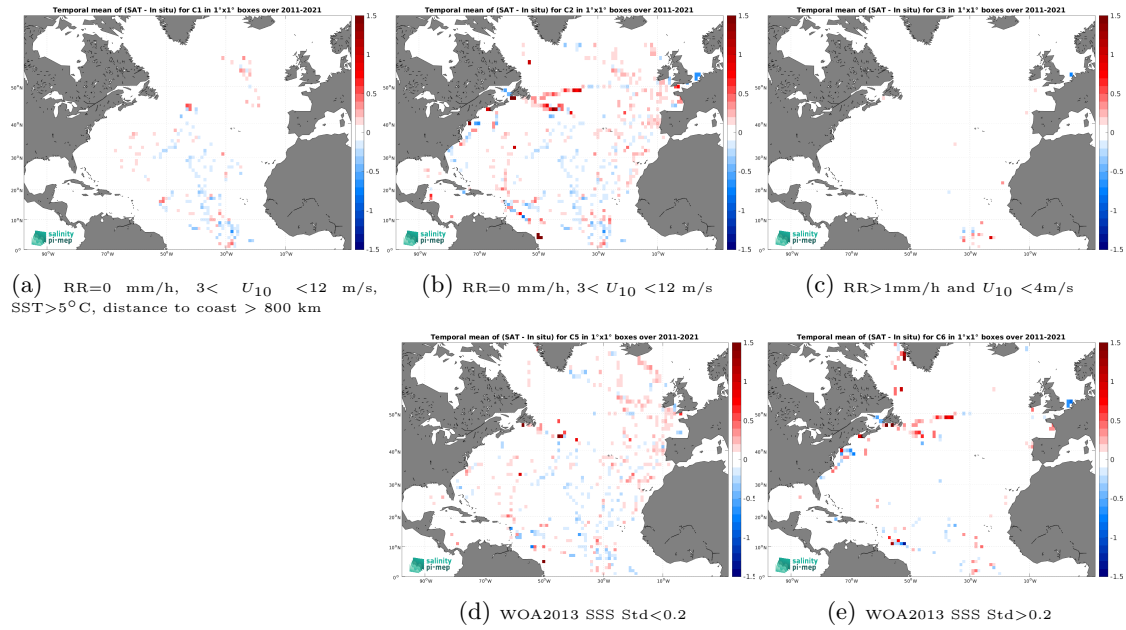
Figure 12: Temporal mean gridded over spatial boxes of size 1^\circ \times 1^\circ of \Delta\text{SSS} (CCI SSS L4 Merged-OI v4.4 - 30-day running (ESA) - TSG (GOSUD-Sailing-ship)) for 5 different subdatasets corresponding to:RR=0 mm/h, 3 < U_{10} < 12 m/s, SST >5^\circ\text{C} , distance to coast > 800 km (a), RR=0 mm/h, 3 < U_{10} < 12 m/s (b), RR >1 mm/h and U_{10} < 4 m/s (c), WOA2013 SSS Std <0.2 (d), WOA2013 SSS Std >0.2 (e).
