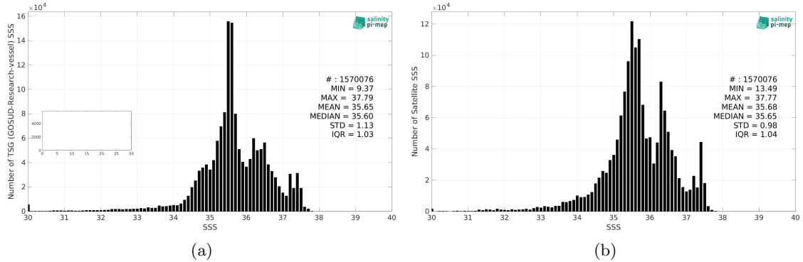
Figure 2: Histograms of SSS from TSG (GOSUD-Research-vessel) (a) and CCI SSS L4 Merged-OI v4.4 - 30-day running (ESA) (b) considering all match-up pairs per bins of 0.1 over the North Atlantic Ocean Pi-MEP region and for the full satellite product period.
