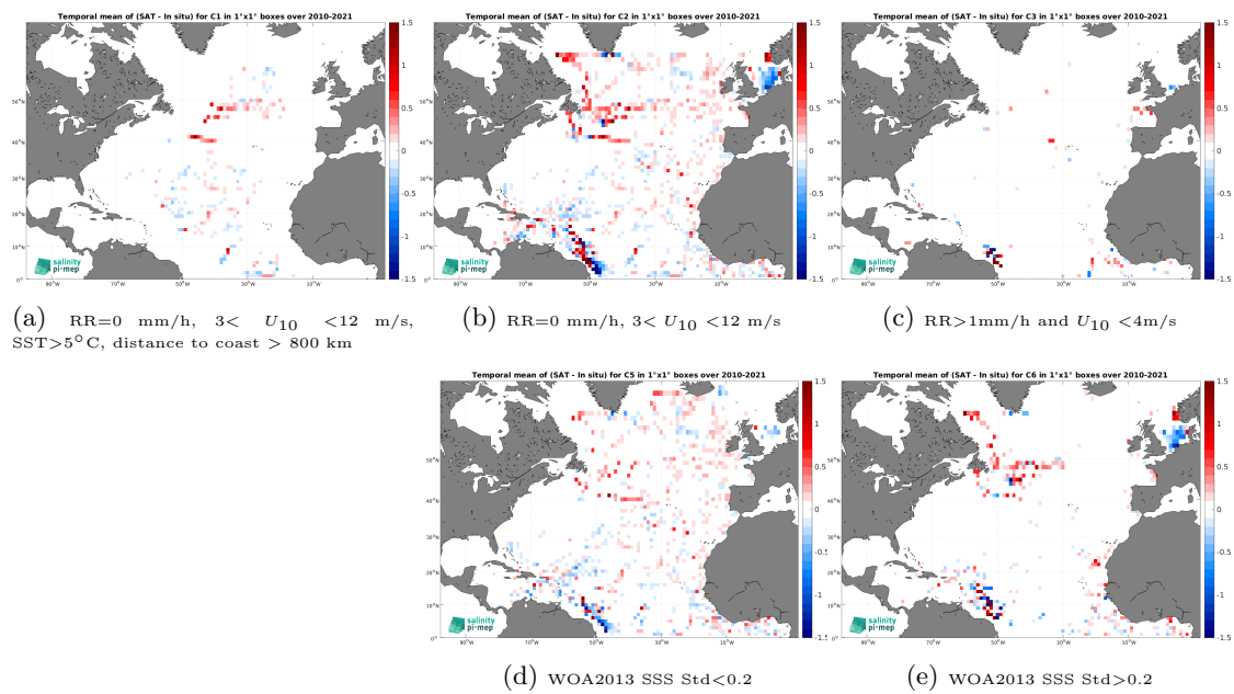
Figure 12: Temporal mean gridded over spatial boxes of size 1^\circ \times 1^\circ of \Delta\text{SSS} (CCI SSS L4 Merged-OI v4.4 - 30-day running (ESA) - TSG (GOSUD-Research-vessel)) for 5 different subdatasets corresponding to:RR=0 mm/h, 3 < U_{10} < 12 m/s, SST >5^\circ\text{C} , distance to coast > 800 km (a), RR=0 mm/h, 3 < U_{10} < 12 m/s (b), RR >1 mm/h and U_{10} < 4 m/s (c), WOA2013 SSS Std <0.2 (d), WOA2013 SSS Std >0.2 (e).
