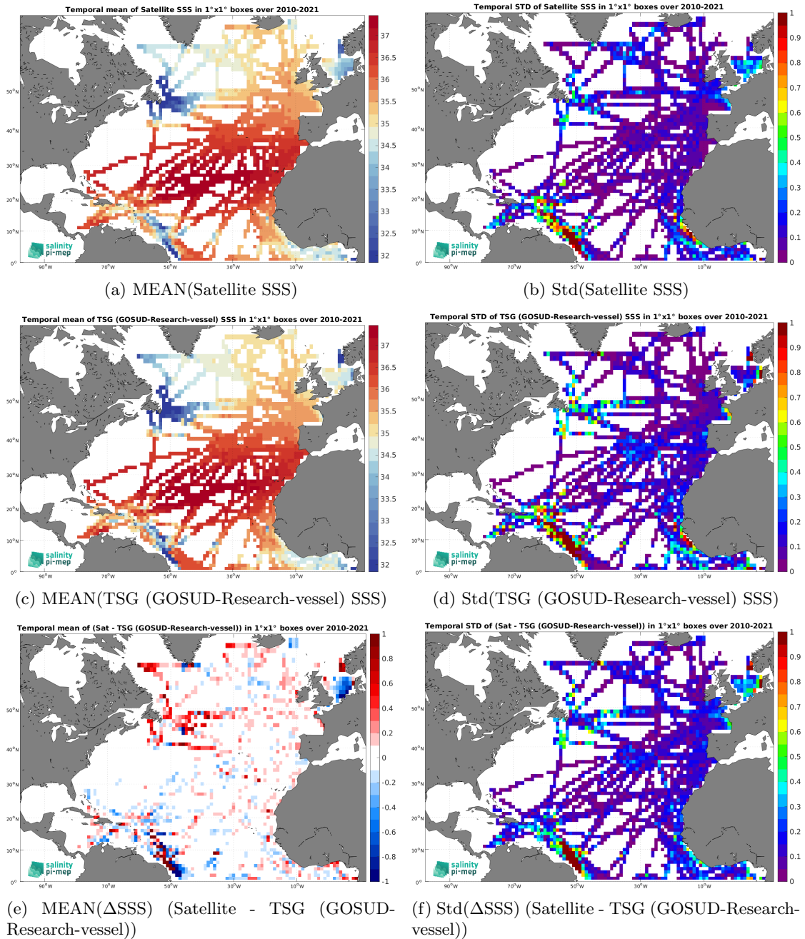
Figure 6: Temporal mean (left) and Std (right) of SSS from CCI SSS L4 Merged-OI v4.4 - 30-day running (ESA) (top), TSG (GOSUD-Research-vessel) (middle), and of \Delta SSS (Satellite - TSG (GOSUD-Research-vessel)). Only match-up pairs are used to generate these maps.
