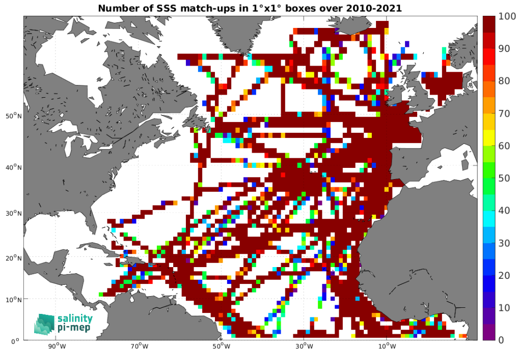
Figure 4: Number of SSS match-ups between TSG (GOSUD-Research-vessel) SSS and the CCI SSS L4 Merged-OI v4.4 - 30-day running (ESA) SSS product for the North Atlantic Ocean Pi-MEP region over 1^\circ \times 1^\circ boxes and for the full satellite product period.
