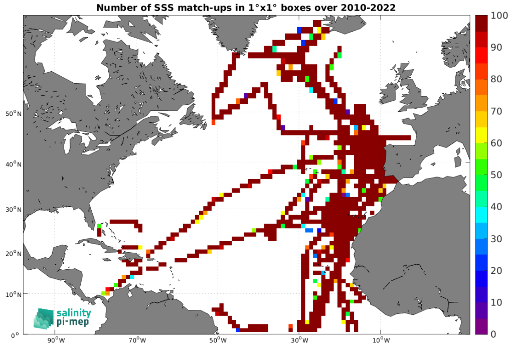
Figure 4: Number of SSS match-ups between TSG (CSIC-UTM) SSS and the CCI SSS L4 Merged-OI v4.4 - 30-day running (ESA) SSS product for the North Atlantic Ocean Pi-MEP region over 1^\circ \times 1^\circ boxes and for the full satellite product period.
