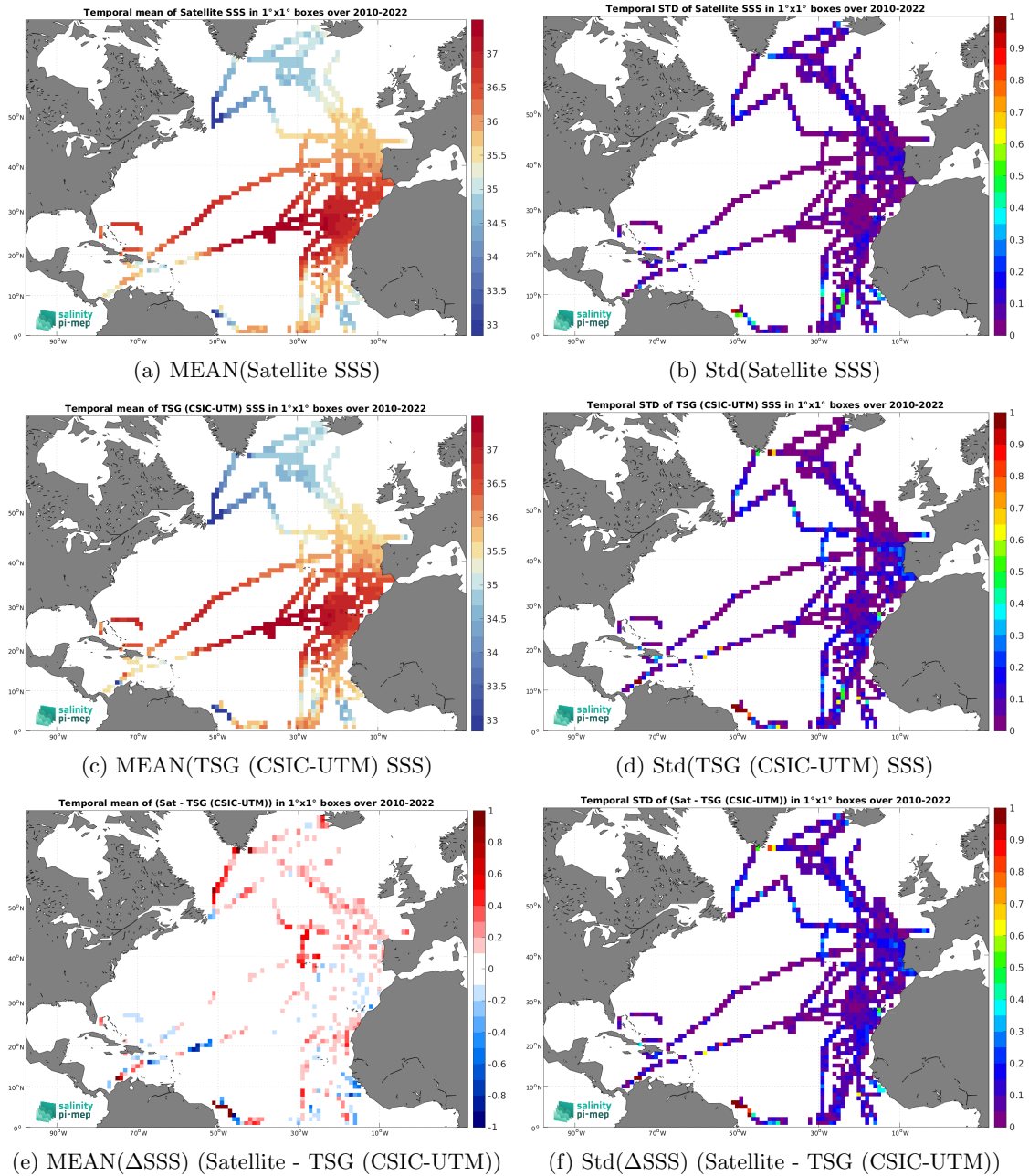
Figure 6: Temporal mean (left) and Std (right) of SSS from CCI SSS L4 Merged-OI v4.4 - 30-day running (ESA) (top), TSG (CSIC-UTM) (middle), and of \Delta SSS (Satellite - TSG (CSIC-UTM)). Only match-up pairs are used to generate these maps.
