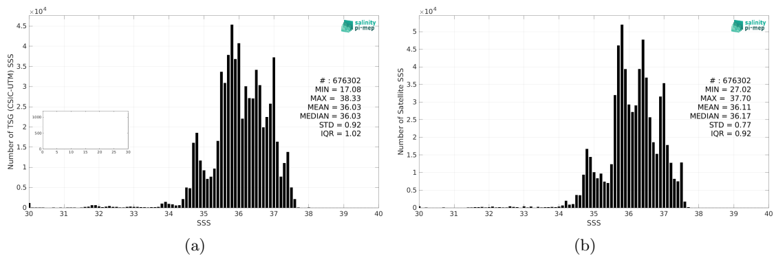
Figure 2: Histograms of SSS from TSG (CSIC-UTM) (a) and CCI SSS L4 Merged-OI v4.4 - 30-day running (ESA) (b) considering all match-up pairs per bins of 0.1 over the North Atlantic Ocean Pi-MEP region and for the full satellite product period.
