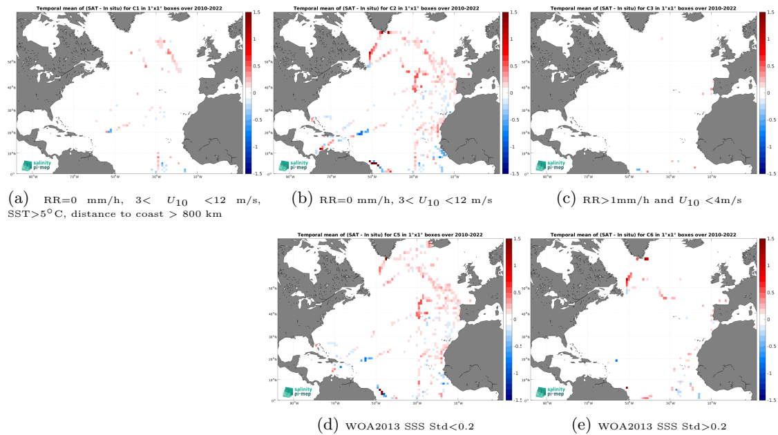
Figure 12: Temporal mean gridded over spatial boxes of size 1^\circ \times 1^\circ of \Delta\text{SSS} (CCI SSS L4 Merged-OI v4.4 - 30-day running (ESA) - TSG (CSIC-UTM)) for 5 different subdatasets corresponding to:RR=0 mm/h, 3 < U_{10} < 12 m/s, SST >5^\circ\text{C} , distance to coast > 800 km (a), RR=0 mm/h, 3 < U_{10} < 12 m/s (b), RR >1 mm/h and U_{10} < 4 m/s (c), WOA2013 SSS Std <0.2 (d), WOA2013 SSS Std >0.2 (e).
