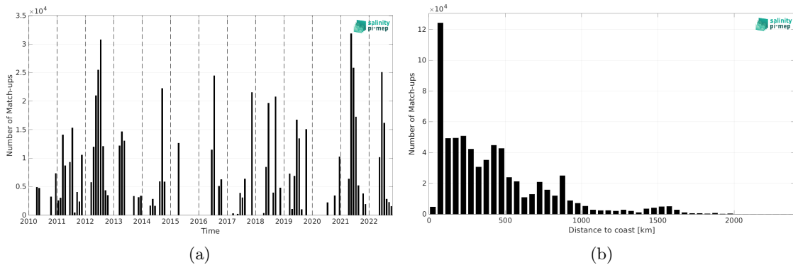
Figure 1: Number of match-ups between TSG (CSIC-UTM) and CCI SSS L4 Merged-OI v4.4 - 30-day running (ESA) SSS as a function of time (a) and as function of the distance to coast (b) over the North Atlantic Ocean Pi-MEP region and for the full satellite product period.
