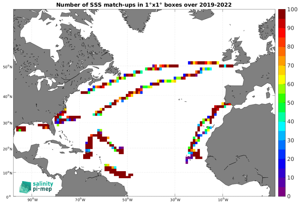
Figure 4: Number of SSS match-ups between Saildrone SSS and the CCI SSS L4 Merged-OI v4.4 - 30-day running (ESA) SSS product for the North Atlantic Ocean Pi-MEP region over 1^\circ \times 1^\circ boxes and for the full satellite product period.
