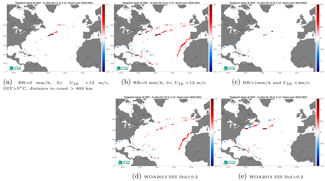
Figure 12: Temporal mean gridded over spatial boxes of size 1^\circ \times 1^\circ of \Delta\text{SSS} (CCI SSS L4 Merged-OI v4.4 - 30-day running (ESA) - Saildrone) for 5 different subdatasets corresponding to:RR=0 mm/h, 3 < U_{10} < 12 m/s, SST >5^\circ\text{C} , distance to coast > 800 km (a), RR=0 mm/h, 3 < U_{10} < 12 m/s (b), RR >1 mm/h and U_{10} < 4 m/s (c), WOA2013 SSS Std <0.2 (d), WOA2013 SSS Std >0.2 (e).
