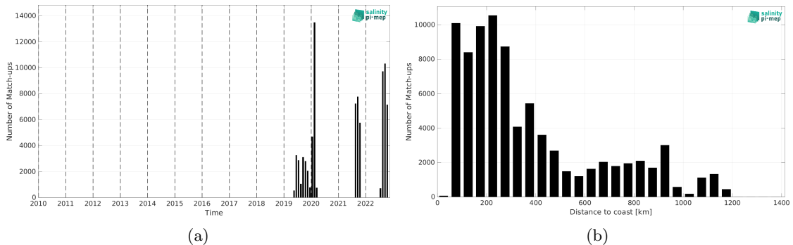
Figure 1: Number of match-ups between Saildrone and CCI SSS L4 Merged-OI v4.4 - 30-day running (ESA) SSS as a function of time (a) and as function of the distance to coast (b) over the North Atlantic Ocean Pi-MEP region and for the full satellite product period.
