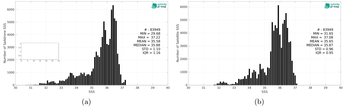
Figure 2: Histograms of SSS from Saildrone (a) and CCI SSS L4 Merged-OI v4.4 - 30-day running (ESA) (b) considering all match-up pairs per bins of 0.1 over the North Atlantic Ocean Pi-MEP region and for the full satellite product period.
