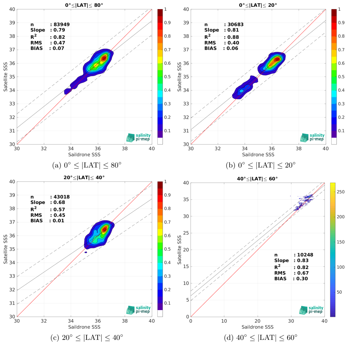
Figure 9: Contour maps of the concentration of CCI SSS L4 Merged-OI v4.4 - 30-day running (ESA) SSS (y-axis) versus Saldrone SSS (x-axis) at match-up pairs for different latitude bands. For each plot, the red line shows x=y . The black thin and dashed lines indicate a linear fit through the data cloud and the \pm 95\% confidence levels, respectively. The number match-up pairs n , the slope and R^2 coefficient of the linear fit, the root mean square (RMS) and the mean bias between satellite and in situ data are indicated for each latitude band in each plots.
