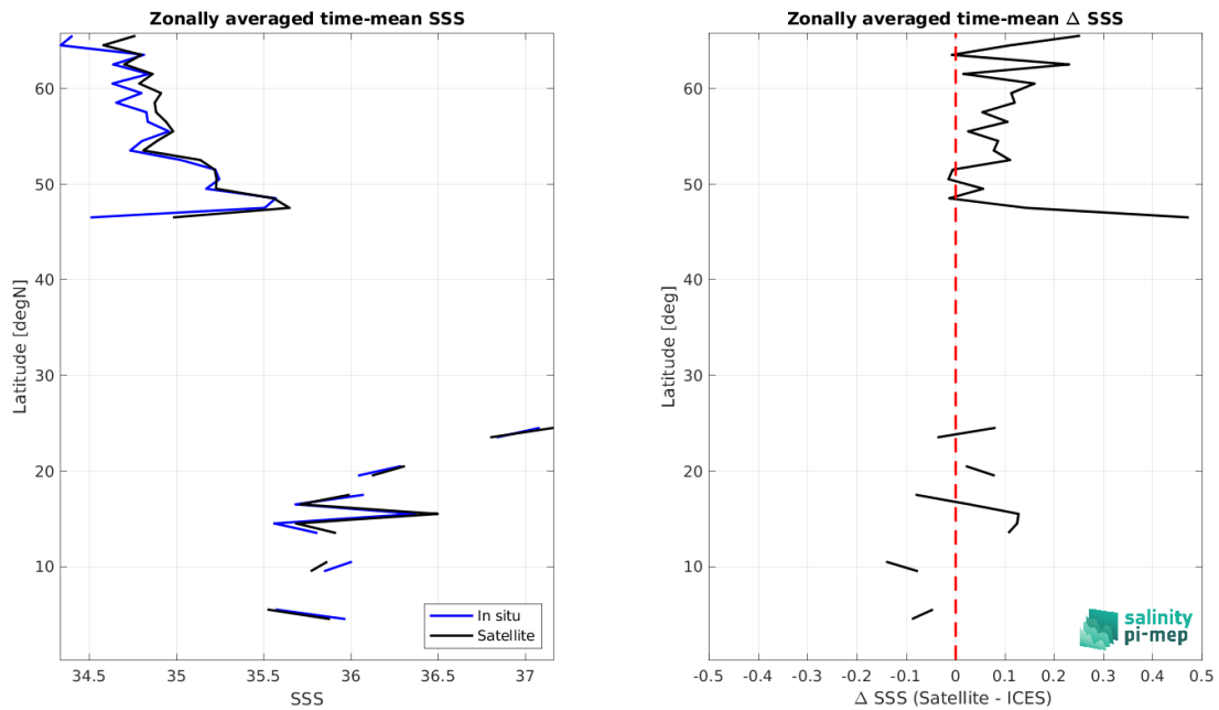
Figure 8: Left panel: Zonal mean SSS from CCI SSS L4 Merged-OI v4.4 - 30-day running (ESA) satellite product (black) and from ICES (blue). Right panel: Zonal mean of \Delta SSS (Satellite - ICES) for all the collected Pi-MEP match-up pairs estimated over the full satellite product period.
