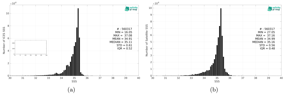
Figure 2: Histograms of SSS from ICES (a) and CCI SSS L4 Merged-OI v4.4 - 30-day running (ESA) (b) considering all match-up pairs per bins of 0.1 over the North Atlantic Ocean Pi-MEP region and for the full satellite product period.
