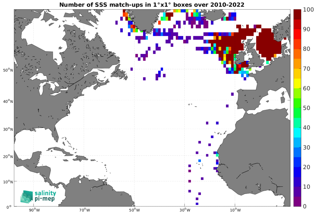
Figure 4: Number of SSS match-ups between ICES SSS and the CCI SSS L4 Merged-OI v4.4 - 30-day running (ESA) SSS product for the North Atlantic Ocean Pi-MEP region over 1^\circ \times 1^\circ boxes and for the full satellite product period.
