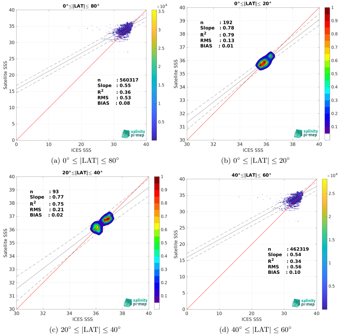
Figure 9: Contour maps of the concentration of CCI SSS L4 Merged-OI v4.4 - 30-day running (ESA) SSS (y-axis) versus ICES SSS (x-axis) at match-up pairs for different latitude bands. For each plot, the red line shows x=y . The black thin and dashed lines indicate a linear fit through the data cloud and the \pm 95\% confidence levels, respectively. The number match-up pairs n , the slope and R^2 coefficient of the linear fit, the root mean square (RMS) and the mean bias between satellite and in situ data are indicated for each latitude band in each plots.
