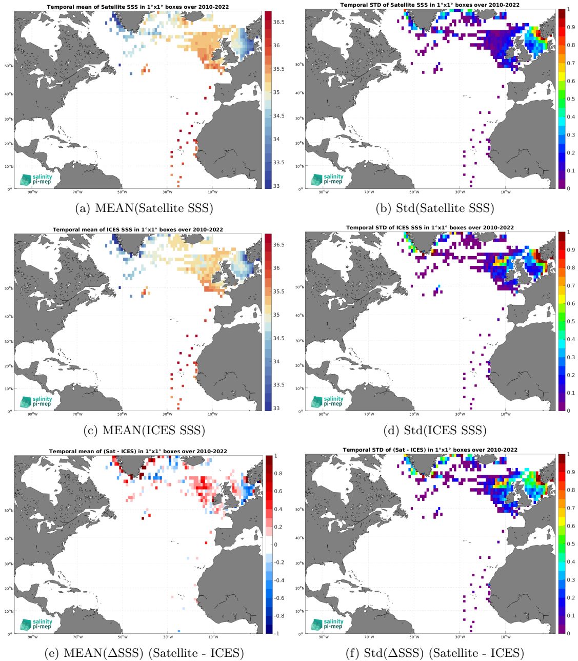
Figure 6: Temporal mean (left) and Std (right) of SSS from CCI SSS L4 Merged-OI v4.4 - 30-day running (ESA) (top), ICES (middle), and of \Delta SSS (Satellite - ICES). Only match-up pairs are used to generate these maps.
