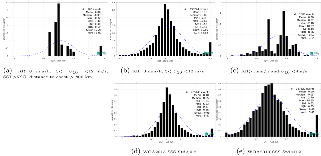
Figure 13: Normalized histogram of \Delta SSS (CCI SSS L4 Merged-OI v4.4 - 30-day running (ESA) - ICES) for 5 different subdatasets corresponding to: RR=0 mm/h, 3 < U_{10} < 12 m/s, SST > 5°C, distance to coast > 800 km (a), RR=0 mm/h, 3 < U_{10} < 12 m/s (b), RR > 1mm/h and U_{10} < 4 m/s (c), WOA2013 SSS Std < 0.2 (d), WOA2013 SSS Std > 0.2 (e).
