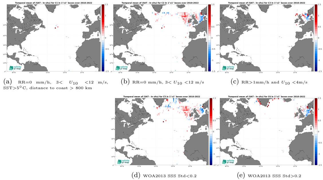
Figure 12: Temporal mean gridded over spatial boxes of size 1^\circ \times 1^\circ of \Delta\text{SSS} (CCI SSS L4 Merged-OI v4.4 - 30-day running (ESA) - ICES) for 5 different subdatasets corresponding to:RR=0 mm/h, 3 < U_{10} < 12 m/s, SST >5^\circ\text{C} , distance to coast > 800 km (a), RR=0 mm/h, 3 < U_{10} < 12 m/s (b), RR >1 mm/h and U_{10} < 4 m/s (c), WOA2013 SSS Std <0.2 (d), WOA2013 SSS Std >0.2 (e).
