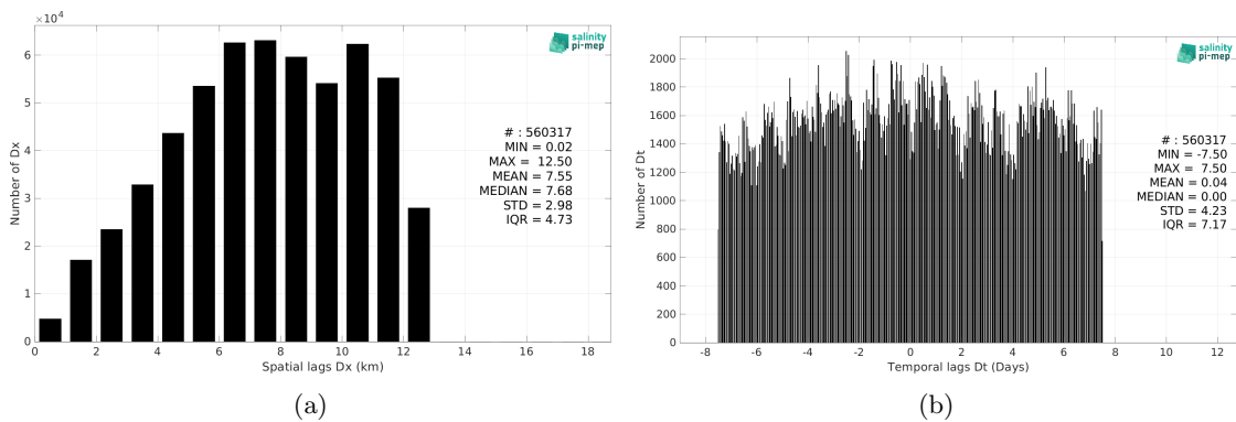
Figure 5: Histograms of the spatial (a) and temporal (b) lags between the location/time of the ICES measurement and the date of the corresponding CCI SSS L4 Merged-OI v4.4 - 30-day running (ESA) SSS pixel.
