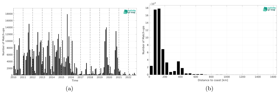
Figure 1: Number of match-ups between ICES and CCI SSS L4 Merged-OI v4.4 - 30-day running (ESA) SSS as a function of time (a) and as function of the distance to coast (b) over the North Atlantic Ocean Pi-MEP region and for the full satellite product period.
