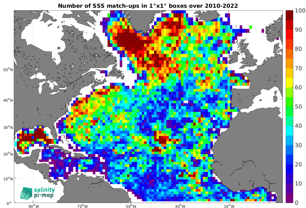
Figure 4: Number of SSS match-ups between Argo SSS and the CCI SSS L4 Merged-OI v4.4 - 30-day running (ESA) SSS product for the North Atlantic Ocean Pi-MEP region over 1^\circ \times 1^\circ boxes and for the full satellite product period.
