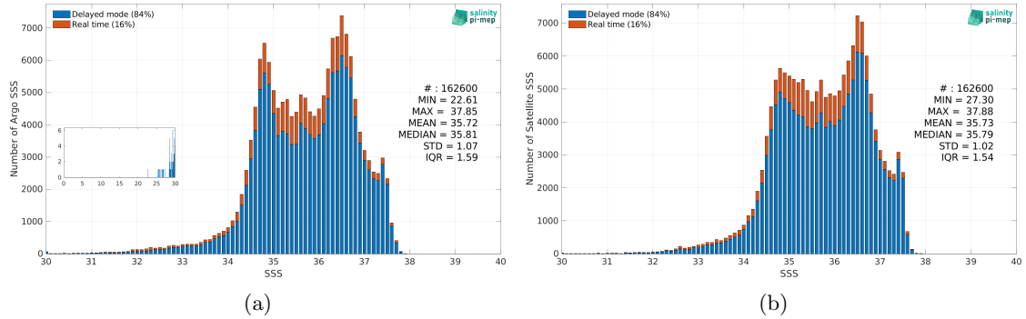
Figure 2: Histograms of SSS from Argo (a) and CCI SSS L4 Merged-OI v4.4 - 30-day running (ESA) (b) considering all match-up pairs per bins of 0.1 over the North Atlantic Ocean Pi-MEP region and for the full satellite product period.
