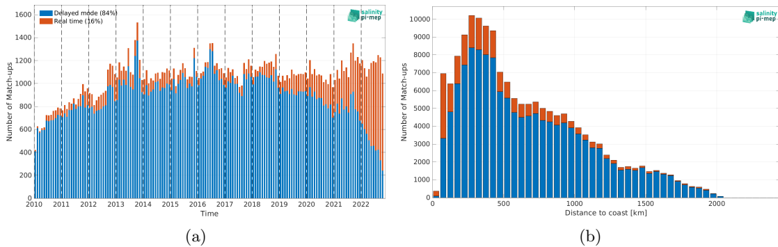
Figure 1: Number of match-ups between Argo and CCI SSS L4 Merged-OI v4.4 - 30-day running (ESA) SSS as a function of time (a) and as function of the distance to coast (b) over the North Atlantic Ocean Pi-MEP region and for the full satellite product period.
