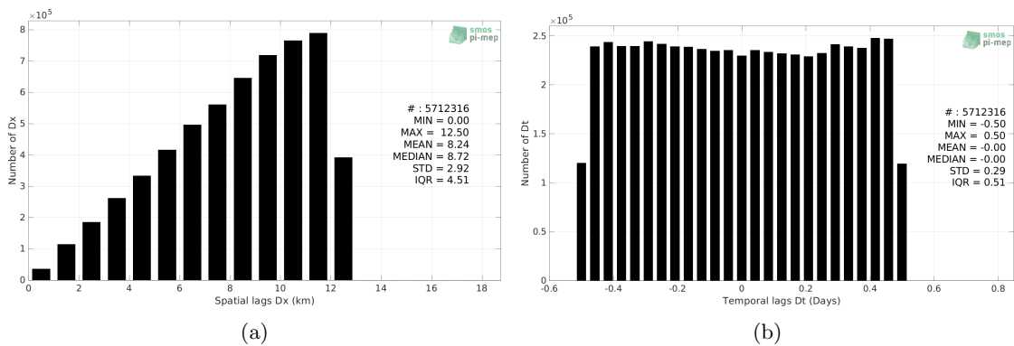
Figure 5: Histograms of the spatial (a) and temporal (b) lags between the location/time of the TSG (SAMOS) measurement and the date of the corresponding CCI SSS L4 Merged-OI v3.2 - 7-day running (ESA) SSS pixel.
