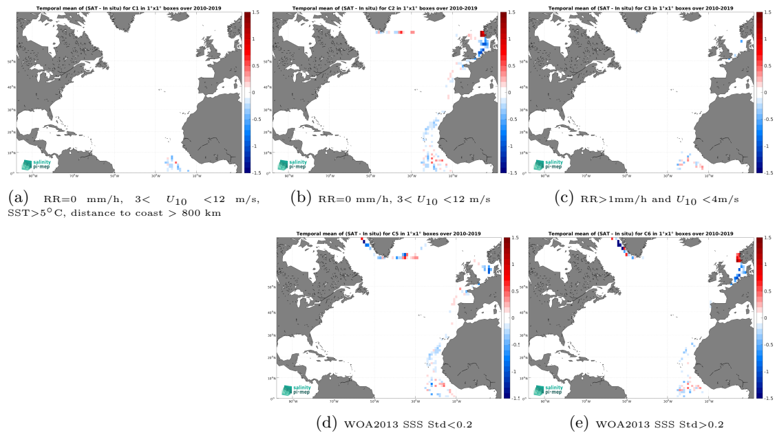
Figure 12: Temporal mean gridded over spatial boxes of size 1^\circ \times 1^\circ of \Delta\text{SSS} (CCI SSS L4 Merged-OI v3.2 - 7-day running (ESA) - TSG (Polarstern)) for 5 different subdatasets corresponding to:RR=0 mm/h, 3 < U_{10} < 12 m/s, SST >5^\circ\text{C} , distance to coast > 800 km (a), RR=0 mm/h, 3 < U_{10} < 12 m/s (b), RR >1 mm/h and U_{10} < 4 m/s (c), WOA2013 SSS Std <0.2 (d), WOA2013 SSS Std >0.2 (e).
