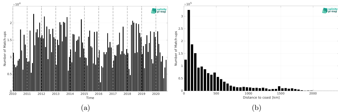
Figure 1: Number of match-ups between TSG (LEGOS-DM) and CCI SSS L4 Merged-OI v3.2 - 7-day running (ESA) SSS as a function of time (a) and as function of the distance to coast (b) over the North Atlantic Ocean Pi-MEP region and for the full satellite product period.
