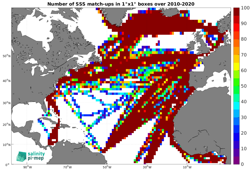
Figure 4: Number of SSS match-ups between TSG (LEGOS-DM) SSS and the CCI SSS L4 Merged-OI v3.2 - 7-day running (ESA) SSS product for the North Atlantic Ocean Pi-MEP region over 1^\circ \times 1^\circ boxes and for the full satellite product period.
