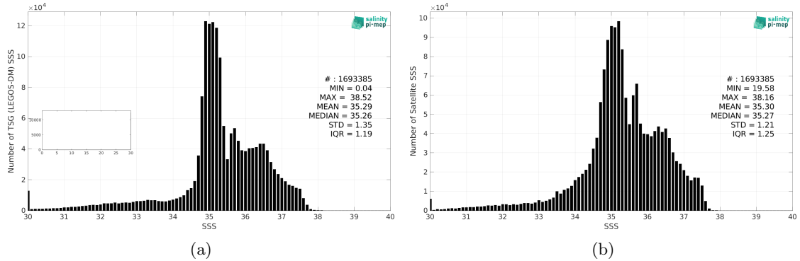
Figure 2: Histograms of SSS from TSG (LEGOS-DM) (a) and CCI SSS L4 Merged-OI v3.2 - 7-day running (ESA) (b) considering all match-up pairs per bins of 0.1 over the North Atlantic Ocean Pi-MEP region and for the full satellite product period.
