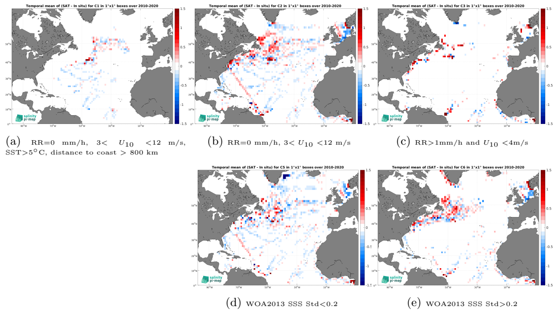
Figure 12: Temporal mean gridded over spatial boxes of size 1^\circ \times 1^\circ of \Delta\text{SSS} (CCI SSS L4 Merged-OI v3.2 - 7-day running (ESA) - TSG (LEGOS-DM)) for 5 different subdatasets corresponding to: RR=0 mm/h, 3 < U_{10} < 12 m/s, SST > 5^\circ\text{C} , distance to coast > 800 km (a), RR=0 mm/h, 3 < U_{10} < 12 m/s (b), RR > 1 mm/h and U_{10} < 4 m/s (c), WOA2013 SSS Std < 0.2 (d), WOA2013 SSS Std > 0.2 (e).
