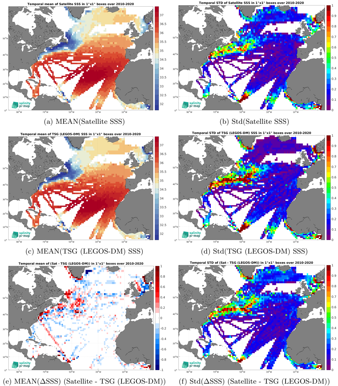
Figure 6: Temporal mean (left) and Std (right) of SSS from CCI SSS L4 Merged-OI v3.2 - 7-day running (ESA) (top), TSG (LEGOS-DM) (middle), and of \Delta SSS (Satellite - TSG (LEGOS-DM)). Only match-up pairs are used to generate these maps.
