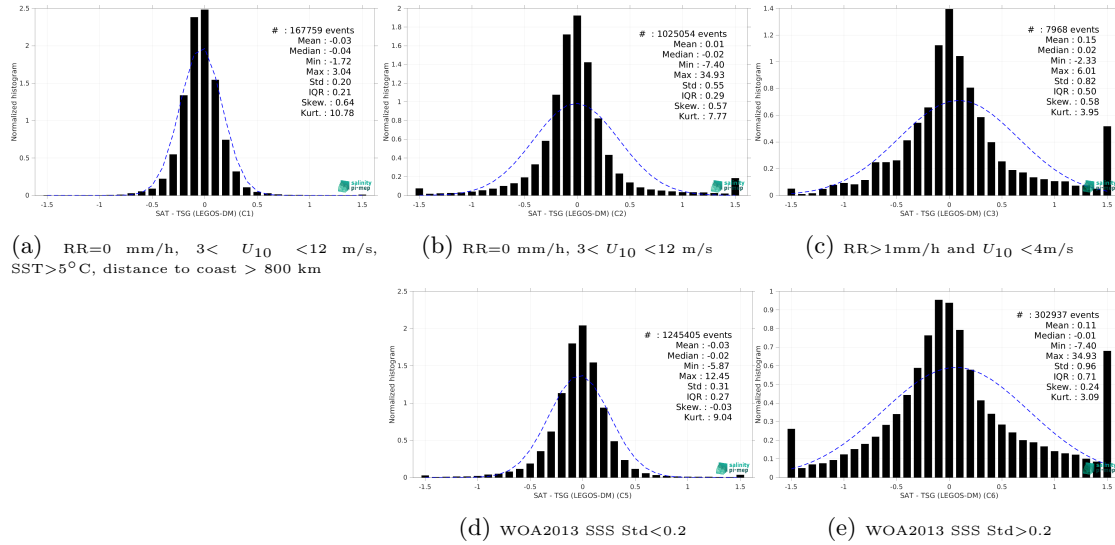
Figure 13: Normalized histogram of \Delta\text{SSS} (CCI SSS L4 Merged-OI v3.2 - 7-day running (ESA) - TSG (LEGOS-DM)) for 5 different subdatasets corresponding to: RR=0 mm/h, 3 < U_{10} < 12 m/s, SST>5°C, distance to coast > 800 km (a), RR=0 mm/h, 3 < U_{10} < 12 m/s (b), RR>1mm/h and U_{10} < 4 m/s (c), WOA2013 SSS Std<0.2 (d), WOA2013 SSS Std>0.2 (e).
