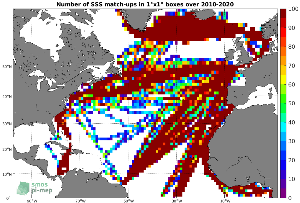
Figure 4: Number of SSS match-ups between TSG (LEGOS-DM) SSS and the CCI SSS L4 Merged-OI v3.2 - 7-day running (ESA) SSS product for the North Atlantic Ocean Pi-MEP region over 1°x1° boxes and for the full satellite product period.
