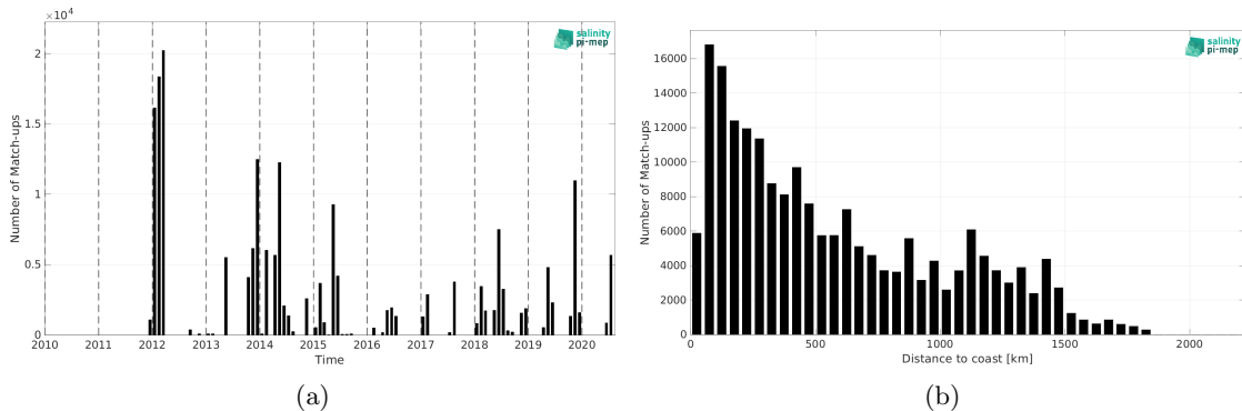
Figure 1: Number of match-ups between TSG (GOSUD-Sailing-ship) and CCI SSS L4 Merged-OI v3.2 - 7-day running (ESA) SSS as a function of time (a) and as function of the distance to coast (b) over the North Atlantic Ocean Pi-MEP region and for the full satellite product period.
