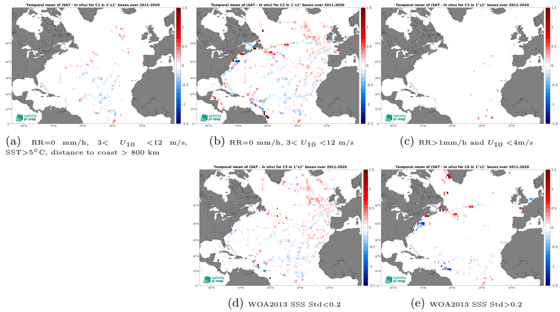
Figure 12: Temporal mean gridded over spatial boxes of size 1^\circ \times 1^\circ of \Delta\text{SSS} (CCI SSS L4 Merged-OI v3.2 - 7-day running (ESA) - TSG (GOSUD-Sailing-ship)) for 5 different subdatasets corresponding to:RR=0 mm/h, 3 < U_{10} < 12 m/s, SST >5^\circ\text{C} , distance to coast > 800 km (a), RR=0 mm/h, 3 < U_{10} < 12 m/s (b), RR >1 mm/h and U_{10} < 4 m/s (c), WOA2013 SSS Std <0.2 (d), WOA2013 SSS Std >0.2 (e).
