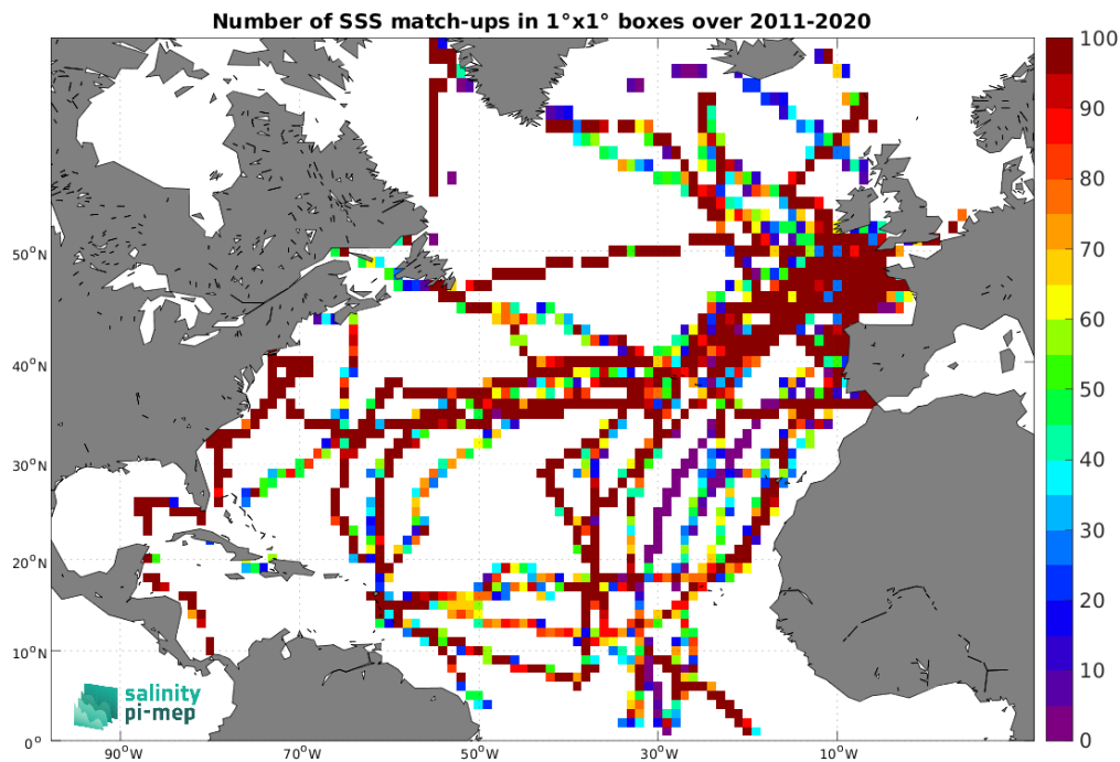
Figure 4: Number of SSS match-ups between TSG (GOSUD-Sailing-ship) SSS and the CCI SSS L4 Merged-OI v3.2 - 7-day running (ESA) SSS product for the North Atlantic Ocean Pi-MEP region over 1^\circ \times 1^\circ boxes and for the full satellite product period.
