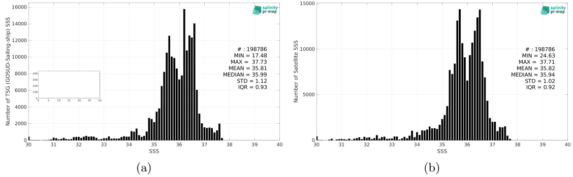
Figure 2: Histograms of SSS from TSG (GOSUD-Sailing-ship) (a) and CCI SSS L4 Merged-OI v3.2 - 7-day running (ESA) (b) considering all match-up pairs per bins of 0.1 over the North Atlantic Ocean Pi-MEP region and for the full satellite product period.
