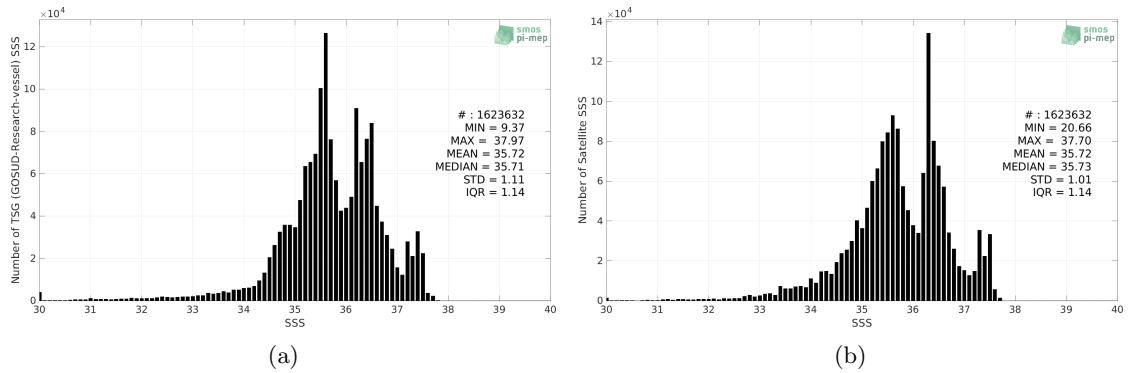
Figure 2: Histograms of SSS from TSG (GOSUD-Research-vessel) (a) and CCI SSS L4 Merged-OI v3.2 - 7-day running (ESA) (b) considering all match-up pairs per bins of 0.1 over the North Atlantic Ocean Pi-MEP region and for the full satellite product period.
