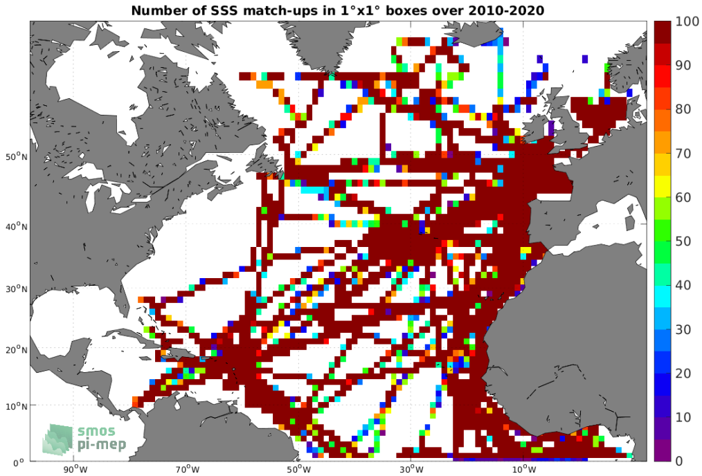
Figure 4: Number of SSS match-ups between TSG (GOSUD-Research-vessel) SSS and the CCI SSS L4 Merged-OI v3.2 - 7-day running (ESA) SSS product for the North Atlantic Ocean Pi-MEP region over 1^\circ \times 1^\circ boxes and for the full satellite product period.
