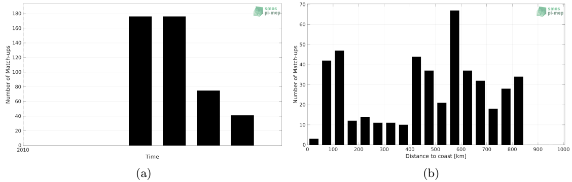
Figure 1: Number of match-ups between Marine mammals and CCI SSS L4 Merged-OI v3.2 - 7-day running (ESA) SSS as a function of time (a) and as function of the distance to coast (b) over the North Atlantic Ocean Pi-MEP region and for the full satellite product period.
