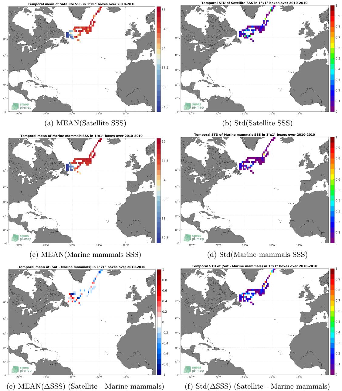
Figure 6: Temporal mean (left) and Std (right) of SSS from CCI SSS L4 Merged-OI v3.2 - 7-day running (ESA) (top), Marine mammals (middle), and of \Delta SSS (Satellite - Marine mammals). Only match-up pairs are used to generate these maps.
