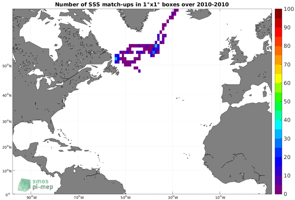
Figure 4: Number of SSS match-ups between Marine mammals SSS and the CCI SSS L4 Merged-OI v3.2 - 7-day running (ESA) SSS product for the North Atlantic Ocean Pi-MEP region over 1^\circ \times 1^\circ boxes and for the full satellite product period.
