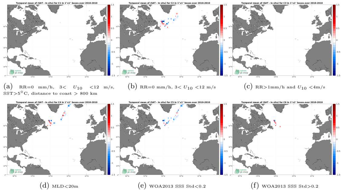
Figure 12: Temporal mean gridded over spatial boxes of size 1^{\circ}\times 1^{\circ} of \Delta\text{SSS} (CCI SSS L4 Merged-OI v3.2 - 7-day running (ESA) - Marine mammals) for 6 different subdatasets corresponding to:RR=0 mm/h, 3 < U_{10} < 12 m/s, SST >5^{\circ}\text{C} , distance to coast > 800 km (a), RR=0 mm/h, 3 < U_{10} < 12 m/s (b), RR >1\text{mm/h} and U_{10} < 4\text{m/s} (c),MLD <20\text{m} (d),WOA2013 SSS Std <0.2 (e),WOA2013 SSS Std >0.2 (f).
