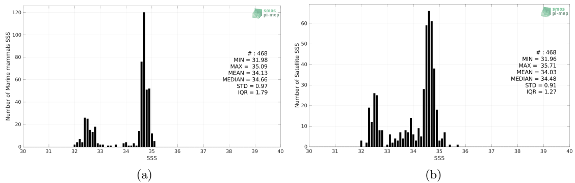
Figure 2: Histograms of SSS from Marine mammals (a) and CCI SSS L4 Merged-OI v3.2 - 7-day running (ESA) (b) considering all match-up pairs per bins of 0.1 over the North Atlantic Ocean Pi-MEP region and for the full satellite product period.
