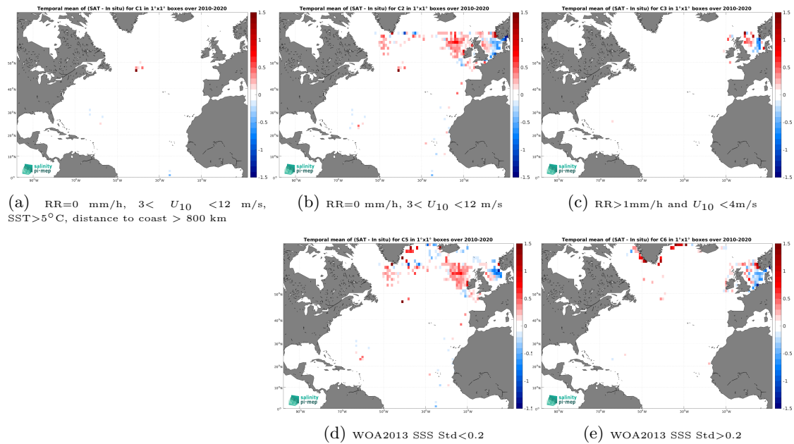
Figure 12: Temporal mean gridded over spatial boxes of size 1^\circ \times 1^\circ of \Delta\text{SSS} (CCI SSS L4 Merged-OI v3.2 - 7-day running (ESA) - ICES) for 5 different subdatasets corresponding to:RR=0 mm/h, 3 < U_{10} < 12 m/s, SST >5^\circ\text{C} , distance to coast > 800 km (a), RR=0 mm/h, 3 < U_{10} < 12 m/s (b), RR >1 mm/h and U_{10} < 4 m/s (c), WOA2013 SSS Std <0.2 (d), WOA2013 SSS Std >0.2 (e).
