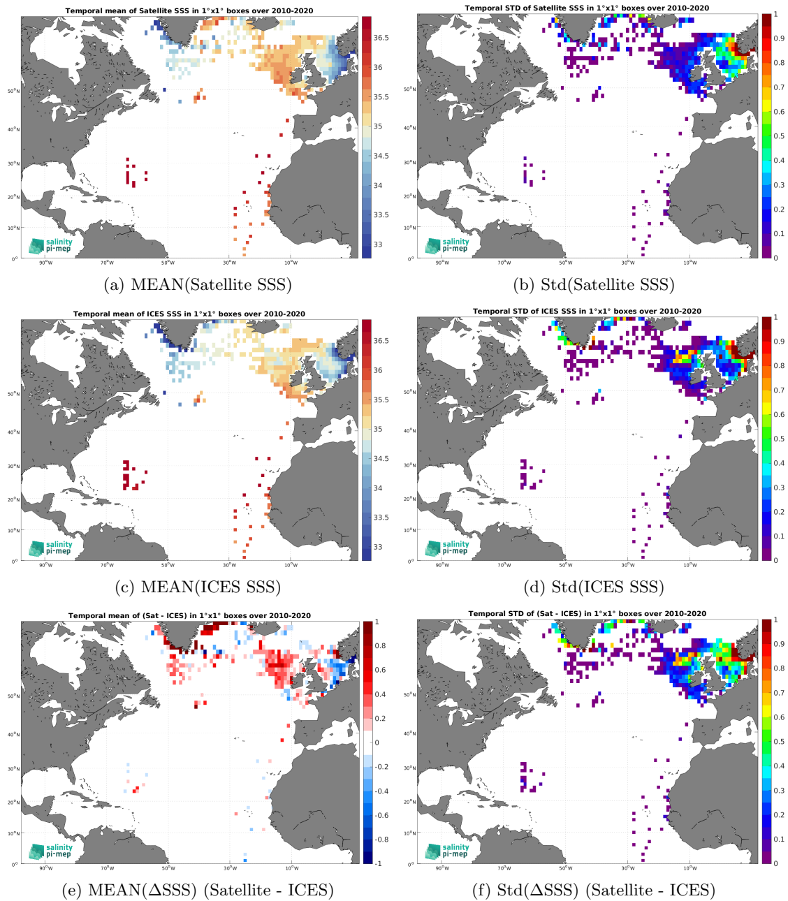
Figure 6: Temporal mean (left) and Std (right) of SSS from CCI SSS L4 Merged-OI v3.2 - 7-day running (ESA) (top), ICES (middle), and of \Delta SSS (Satellite - ICES). Only match-up pairs are used to generate these maps.
