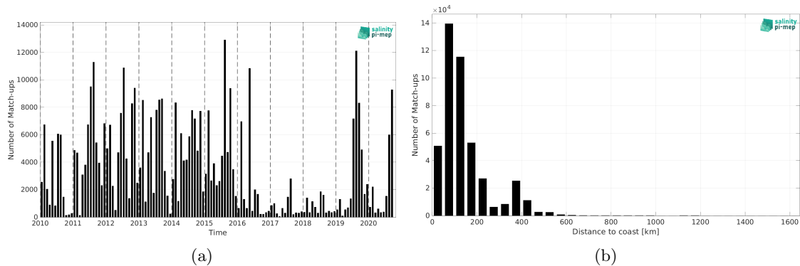
Figure 1: Number of match-ups between ICES and CCI SSS L4 Merged-OI v3.2 - 7-day running (ESA) SSS as a function of time (a) and as function of the distance to coast (b) over the North Atlantic Ocean Pi-MEP region and for the full satellite product period.
