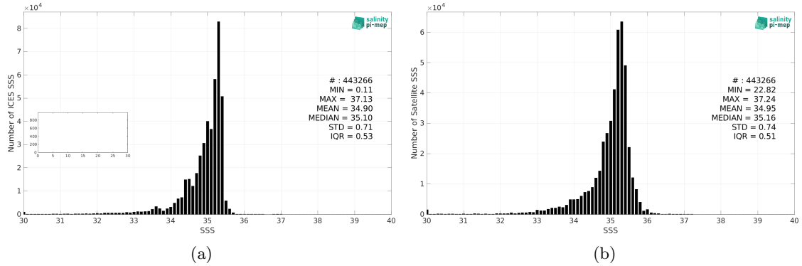
Figure 2: Histograms of SSS from ICES (a) and CCI SSS L4 Merged-OI v3.2 - 7-day running (ESA) (b) considering all match-up pairs per bins of 0.1 over the North Atlantic Ocean Pi-MEP region and for the full satellite product period.
