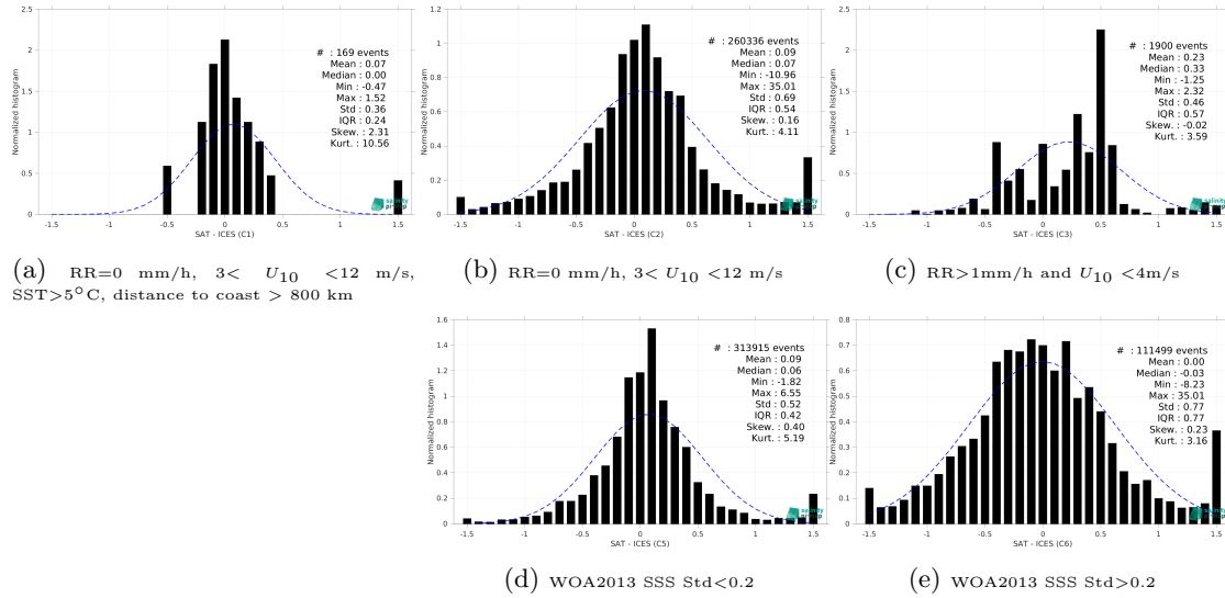
Figure 13: Normalized histogram of \Delta SSS (CCI SSS L4 Merged-OI v3.2 - 7-day running (ESA) - ICES) for 5 different subdatasets corresponding to: RR=0 mm/h, 3 < U_{10} < 12 m/s, SST>5°C, distance to coast > 800 km (a), RR=0 mm/h, 3 < U_{10} < 12 m/s (b), RR>1mm/h and U_{10} < 4 m/s (c), WOA2013 SSS Std<0.2 (d), WOA2013 SSS Std>0.2 (e).
