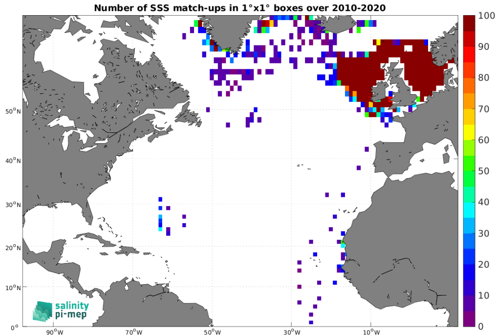
Figure 4: Number of SSS match-ups between ICES SSS and the CCI SSS L4 Merged-OI v3.2 - 7-day running (ESA) SSS product for the North Atlantic Ocean Pi-MEP region over 1^\circ \times 1^\circ boxes and for the full satellite product period.
