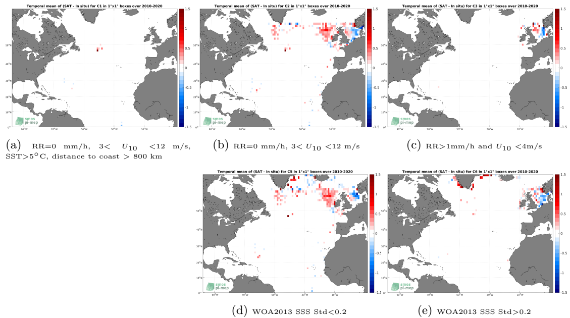
Figure 12: Temporal mean gridded over spatial boxes of size 1^\circ \times 1^\circ of \Delta SSS (CCI SSS L4 Merged-OI v3.2 - 7-day running (ESA) - ICES) for 5 different subdatasets corresponding to:RR=0 mm/h, 3 < U_{10} < 12 m/s, SST >5^\circ\text{C} , distance to coast > 800 km (a), RR=0 mm/h, 3 < U_{10} < 12 m/s (b), RR >1 mm/h and U_{10} < 4 m/s (c), WOA2013 SSS Std <0.2 (d), WOA2013 SSS Std >0.2 (e).
