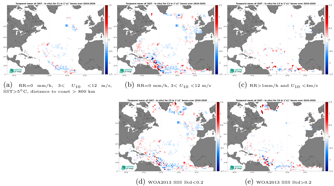
Figure 11: Temporal mean gridded over spatial boxes of size 1^\circ \times 1^\circ of \Delta\text{SSS} (CCI SSS L4 Merged-OI v3.2 - 7-day running (ESA) - Surface drifters) for 5 different subdatasets corresponding to:RR=0 mm/h, 3 < U_{10} < 12 m/s, SST >5^\circ\text{C} , distance to coast > 800 km (a), RR=0 mm/h, 3 < U_{10} < 12 m/s (b), RR >1 mm/h and U_{10} < 4 m/s (c), WOA2013 SSS Std <0.2 (d), WOA2013 SSS Std >0.2 (e).
