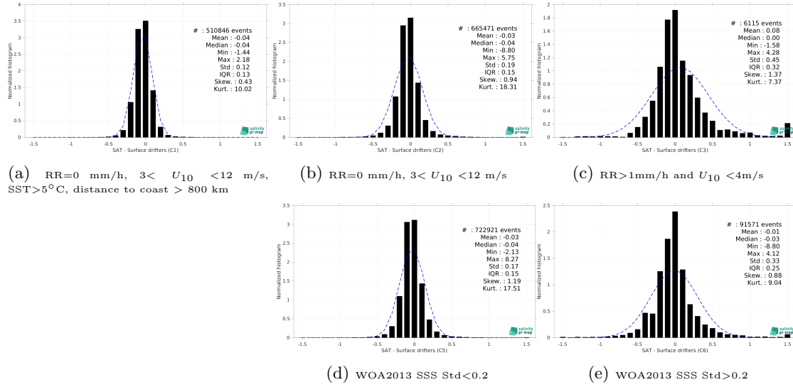
Figure 12: Normalized histogram of \Delta\text{SSS} (CCI SSS L4 Merged-OI v3.2 - 7-day running (ESA) - Surface drifters) for 5 different subdatasets corresponding to: RR=0 mm/h, 3 < U_{10} < 12 m/s, SST>5°C, distance to coast > 800 km (a), RR=0 mm/h, 3 < U_{10} < 12 m/s (b), RR>1mm/h and U_{10} < 4 m/s (c), WOA2013 SSS Std<0.2 (d), WOA2013 SSS Std>0.2 (e).
