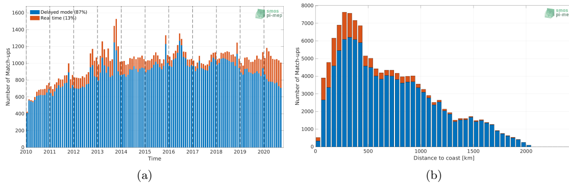
Figure 1: Number of match-ups between Argo and CCI SSS L4 Merged-OI v3.2 - 7-day running (ESA) SSS as a function of time (a) and as function of the distance to coast (b) over the North Atlantic Ocean Pi-MEP region and for the full satellite product period.
