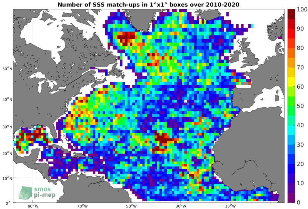
Figure 4: Number of SSS match-ups between Argo SSS and the CCI SSS L4 Merged-OI v3.2 - 7-day running (ESA) SSS product for the North Atlantic Ocean Pi-MEP region over 1^\circ \times 1^\circ boxes and for the full satellite product period.
