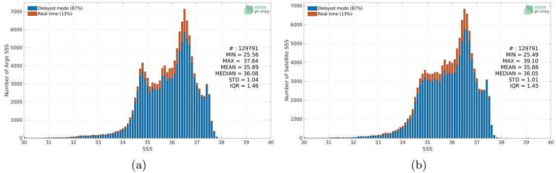
Figure 2: Histograms of SSS from Argo (a) and CCI SSS L4 Merged-OI v3.2 - 7-day running (ESA) (b) considering all match-up pairs per bins of 0.1 over the North Atlantic Ocean Pi-MEP region and for the full satellite product period.
