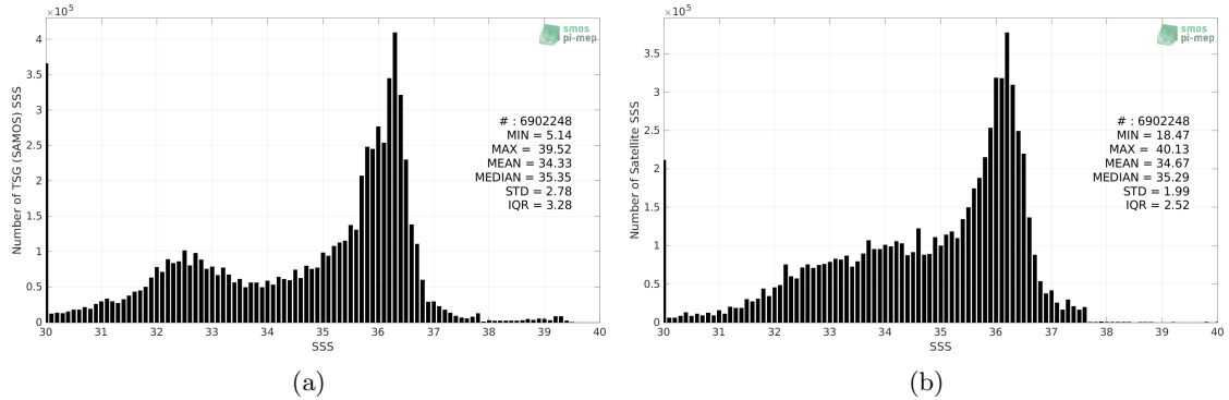
Figure 2: Histograms of SSS from TSG (SAMOS) (a) and CCI SSS L4 Merged-OI v3.2 - 30-day running (ESA) (b) considering all match-up pairs per bins of 0.1 over the North Atlantic Ocean Pi-MEP region and for the full satellite product period.
