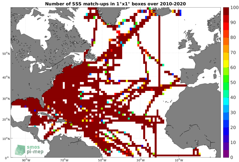
Figure 4: Number of SSS match-ups between TSG (SAMOS) SSS and the CCI SSS L4 Merged-OI v3.2 - 30-day running (ESA) SSS product for the North Atlantic Ocean Pi-MEP region over 1^\circ \times 1^\circ boxes and for the full satellite product period.
