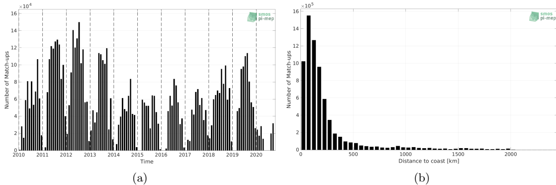
Figure 1: Number of match-ups between TSG (SAMOS) and CCI SSS L4 Merged-OI v3.2 - 30-day running (ESA) SSS as a function of time (a) and as function of the distance to coast (b) over the North Atlantic Ocean Pi-MEP region and for the full satellite product period.
