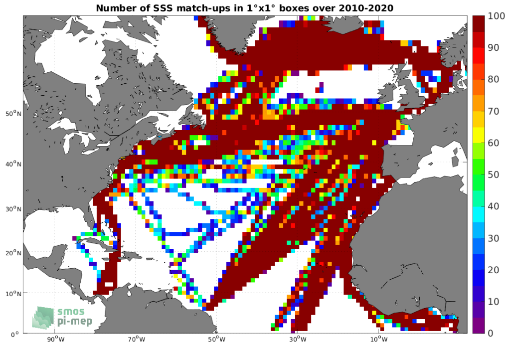
Figure 4: Number of SSS match-ups between TSG (LEGOS-DM) SSS and the CCI SSS L4 Merged-OI v3.2 - 30-day running (ESA) SSS product for the North Atlantic Ocean Pi-MEP region over 1^\circ \times 1^\circ boxes and for the full satellite product period.
