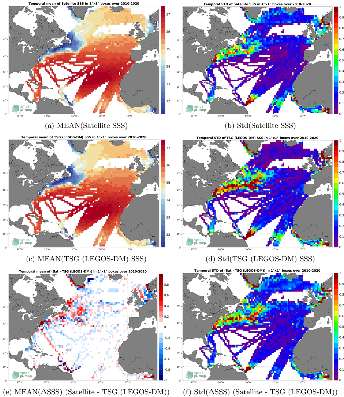
Figure 6: Temporal mean (left) and Std (right) of SSS from CCI SSS L4 Merged-OI v3.2 - 30-day running (ESA) (top), TSG (LEGOS-DM) (middle), and of \Delta SSS (Satellite - TSG (LEGOS-DM)). Only match-up pairs are used to generate these maps.
