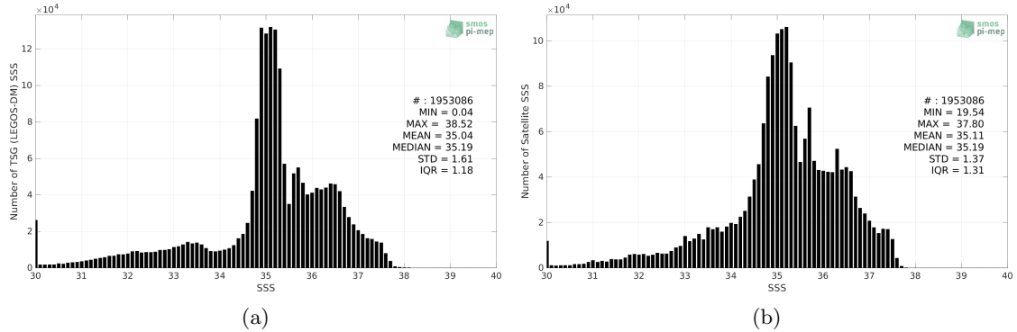
Figure 2: Histograms of SSS from TSG (LEGOS-DM) (a) and CCI SSS L4 Merged-OI v3.2 - 30-day running (ESA) (b) considering all match-up pairs per bins of 0.1 over the North Atlantic Ocean Pi-MEP region and for the full satellite product period.
