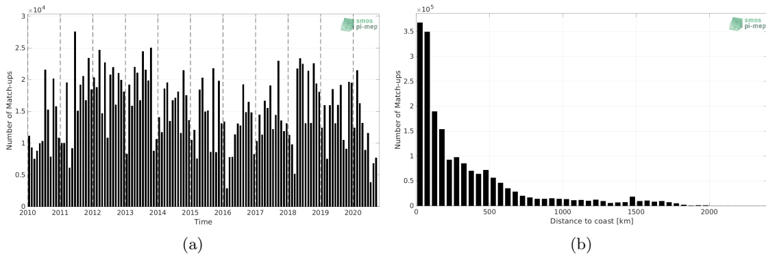
Figure 1: Number of match-ups between TSG (LEGOS-DM) and CCI SSS L4 Merged-OI v3.2 - 30-day running (ESA) SSS as a function of time (a) and as function of the distance to coast (b) over the North Atlantic Ocean Pi-MEP region and for the full satellite product period.
