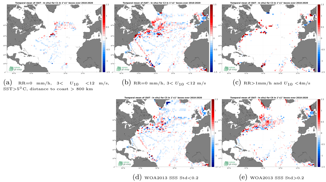
Figure 12: Temporal mean gridded over spatial boxes of size 1^\circ \times 1^\circ of \Delta\text{SSS} (CCI SSS L4 Merged-OI v3.2 - 30-day running (ESA) - TSG (LEGOS-DM)) for 5 different subdatasets corresponding to:RR=0 mm/h, 3 < U_{10} < 12 m/s, SST >5^\circ\text{C} , distance to coast > 800 km (a), RR=0 mm/h, 3 < U_{10} < 12 m/s (b), RR >1 mm/h and U_{10} < 4 m/s (c), WOA2013 SSS Std <0.2 (d), WOA2013 SSS Std >0.2 (e).
