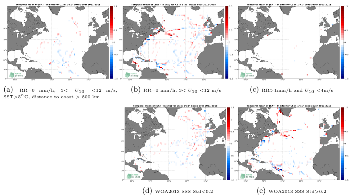
Figure 12: Temporal mean gridded over spatial boxes of size 1^\circ \times 1^\circ of \Delta SSS (CCI SSS L4 Merged-OI v3.2 - 30-day running (ESA) - TSG (GOSUD-Sailing-ship)) for 5 different subdatasets corresponding to: RR=0 mm/h, 3 < U_{10} < 12 m/s, SST > 5°C, distance to coast > 800 km (a), RR=0 mm/h, 3 < U_{10} < 12 m/s (b), RR > 1mm/h and U_{10} < 4 m/s (c), WOA2013 SSS Std < 0.2 (d), WOA2013 SSS Std > 0.2 (e).
