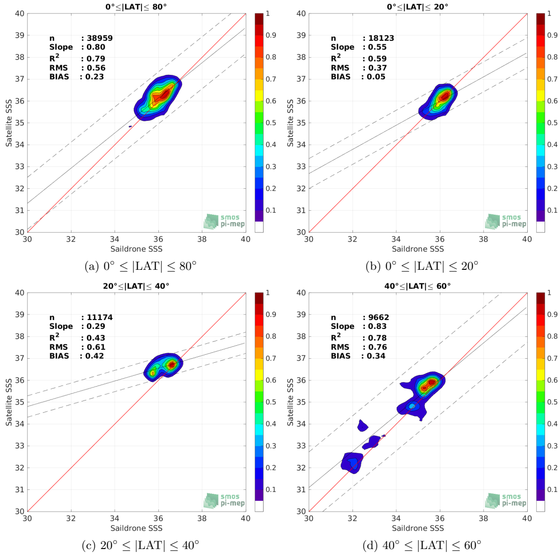
Figure 9: Contour maps of the concentration of CCI SSS L4 Merged-OI v3.2 - 30-day running (ESA) SSS (y-axis) versus Saldrone SSS (x-axis) at match-up pairs for different latitude bands. For each plot, the red line shows x=y . The black thin and dashed lines indicate a linear fit through the data cloud and the \pm 95\% confidence levels, respectively. The number match-up pairs n , the slope and R^2 coefficient of the linear fit, the root mean square (RMS) and the mean bias between satellite and in situ data are indicated for each latitude band in each plots.
