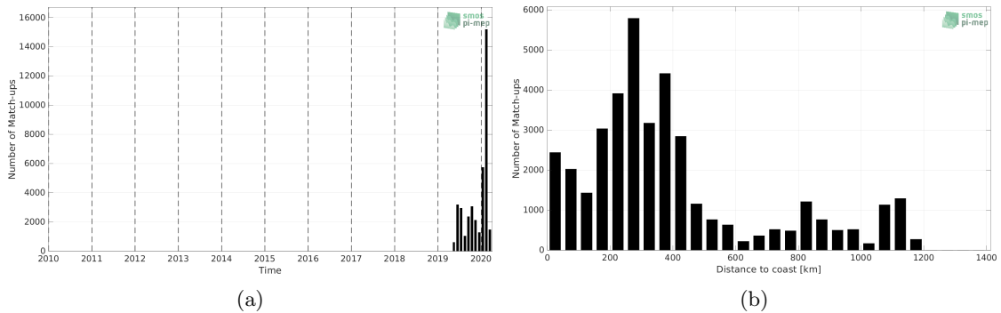
Figure 1: Number of match-ups between Saildrone and CCI SSS L4 Merged-OI v3.2 - 30-day running (ESA) SSS as a function of time (a) and as function of the distance to coast (b) over the North Atlantic Ocean Pi-MEP region and for the full satellite product period.
