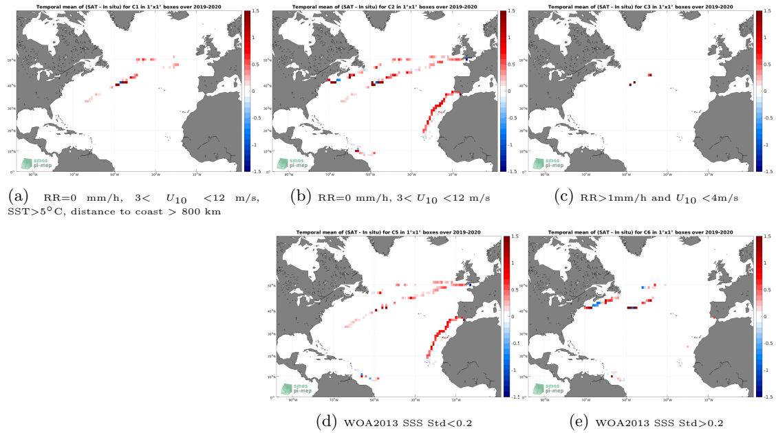
Figure 12: Temporal mean gridded over spatial boxes of size 1^\circ \times 1^\circ of \Delta\text{SSS} (CCI SSS L4 Merged-OI v3.2 - 30-day running (ESA) - Saildrone) for 5 different subdatasets corresponding to:RR=0 mm/h, 3 < U_{10} < 12 m/s, SST >5^\circ\text{C} , distance to coast > 800 km (a), RR=0 mm/h, 3 < U_{10} < 12 m/s (b), RR >1 mm/h and U_{10} < 4 m/s (c), WOA2013 SSS Std <0.2 (d), WOA2013 SSS Std >0.2 (e).
