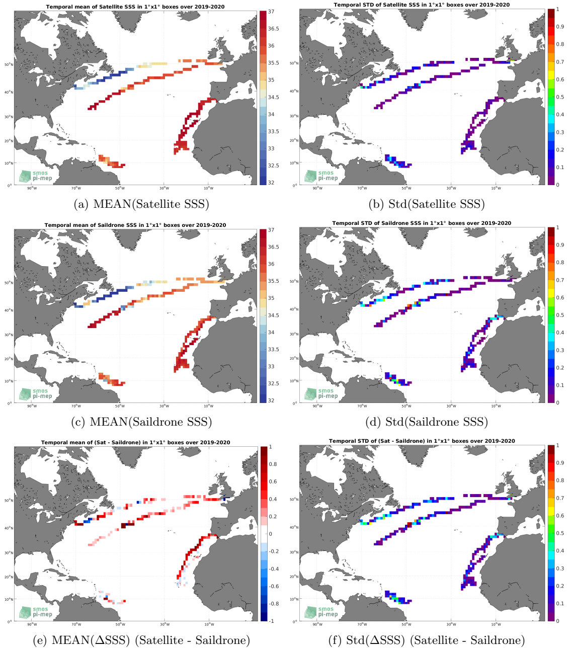
Figure 6: Temporal mean (left) and Std (right) of SSS from CCI SSS L4 Merged-OI v3.2 - 30-day running (ESA) (top), Saildrone (middle), and of \Delta SSS (Satellite - Saildrone). Only match-up pairs are used to generate these maps.
