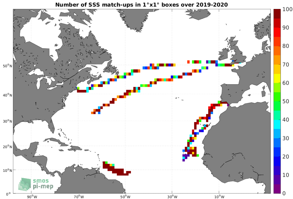
Figure 4: Number of SSS match-ups between Saildrone SSS and the CCI SSS L4 Merged-OI v3.2 - 30-day running (ESA) SSS product for the North Atlantic Ocean Pi-MEP region over 1^\circ \times 1^\circ boxes and for the full satellite product period.
