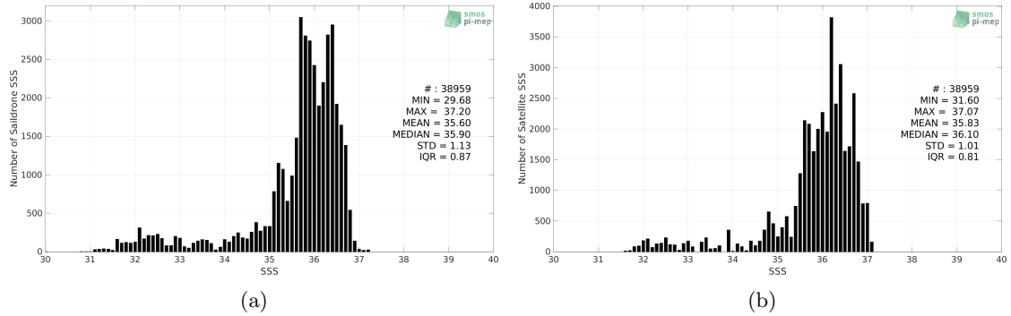
Figure 2: Histograms of SSS from Saildrone (a) and CCI SSS L4 Merged-OI v3.2 - 30-day running (ESA) (b) considering all match-up pairs per bins of 0.1 over the North Atlantic Ocean Pi-MEP region and for the full satellite product period.
