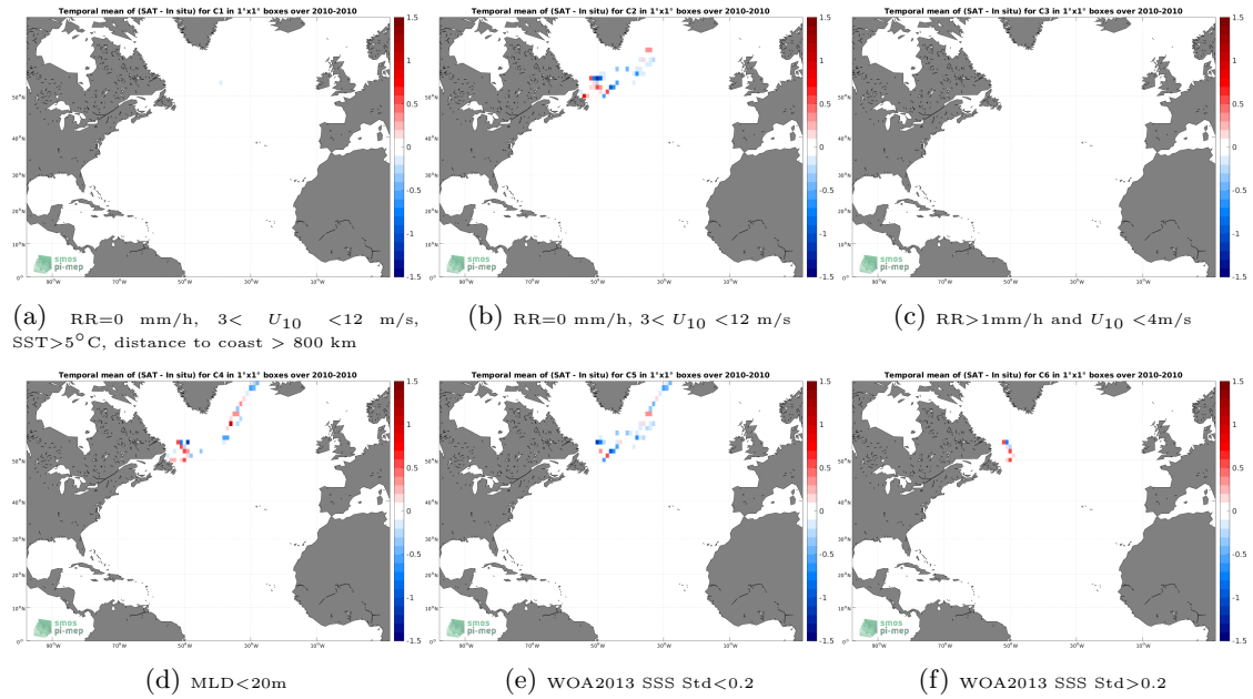
Figure 12: Temporal mean gridded over spatial boxes of size 1^{\circ}\times 1^{\circ} of \Delta\text{SSS} (CCI SSS L4 Merged-OI v3.2 - 30-day running (ESA) - Marine mammals) for 6 different subdatasets corresponding to:RR=0 mm/h, 3 < U_{10} < 12 m/s, SST >5^{\circ}\text{C} , distance to coast > 800 km (a), RR=0 mm/h, 3 < U_{10} < 12 m/s (b), RR >1\text{mm/h} and U_{10} < 4\text{m/s} (c),MLD <20\text{m} (d),WOA2013 SSS Std <0.2 (e),WOA2013 SSS Std >0.2 (f).
