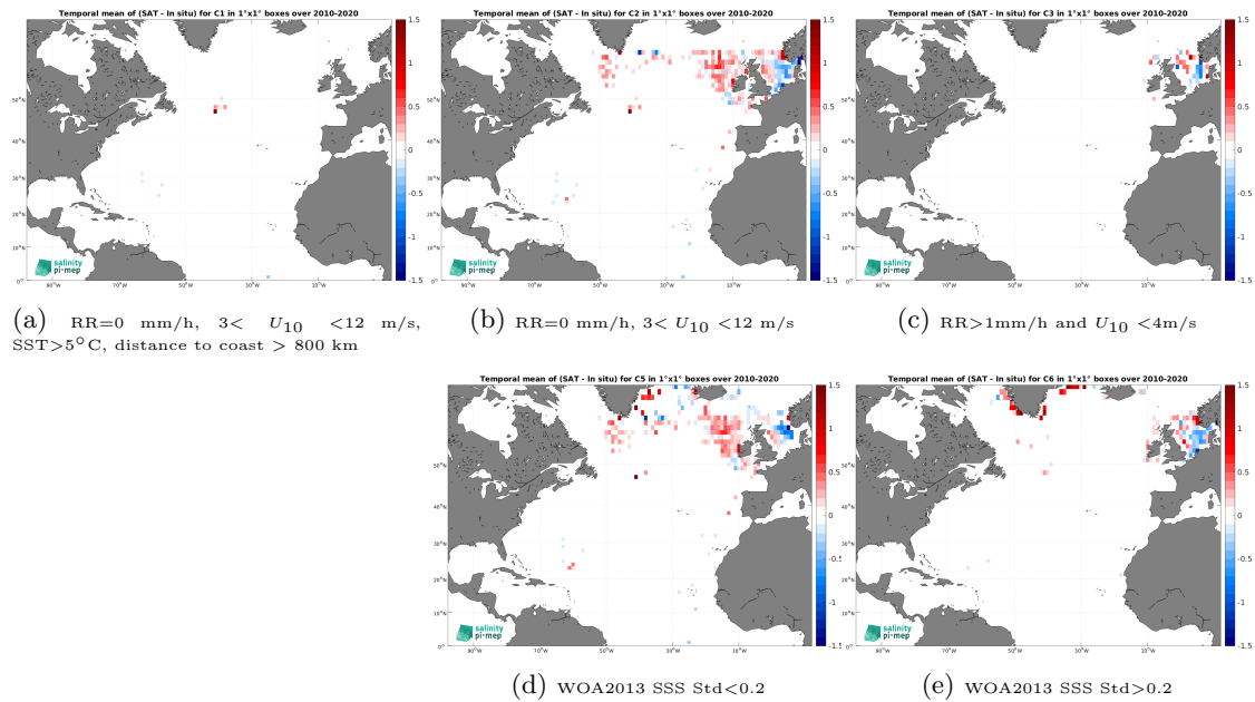
Figure 12: Temporal mean gridded over spatial boxes of size 1^\circ \times 1^\circ of \Delta\text{SSS} (CCI SSS L4 Merged-OI v3.2 - 30-day running (ESA) - ICES) for 5 different subdatasets corresponding to:RR=0 mm/h, 3 < U_{10} < 12 m/s, SST >5^\circ\text{C} , distance to coast > 800 km (a), RR=0 mm/h, 3 < U_{10} < 12 m/s (b), RR >1 mm/h and U_{10} < 4 m/s (c), WOA2013 SSS Std <0.2 (d), WOA2013 SSS Std >0.2 (e).
