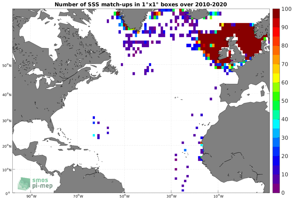
Figure 4: Number of SSS match-ups between ICES SSS and the CCI SSS L4 Merged-OI v3.2 - 30-day running (ESA) SSS product for the North Atlantic Ocean Pi-MEP region over 1^\circ \times 1^\circ boxes and for the full satellite product period.
