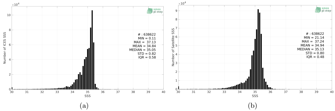
Figure 2: Histograms of SSS from ICES (a) and CCI SSS L4 Merged-OI v3.2 - 30-day running (ESA) (b) considering all match-up pairs per bins of 0.1 over the North Atlantic Ocean Pi-MEP region and for the full satellite product period.
