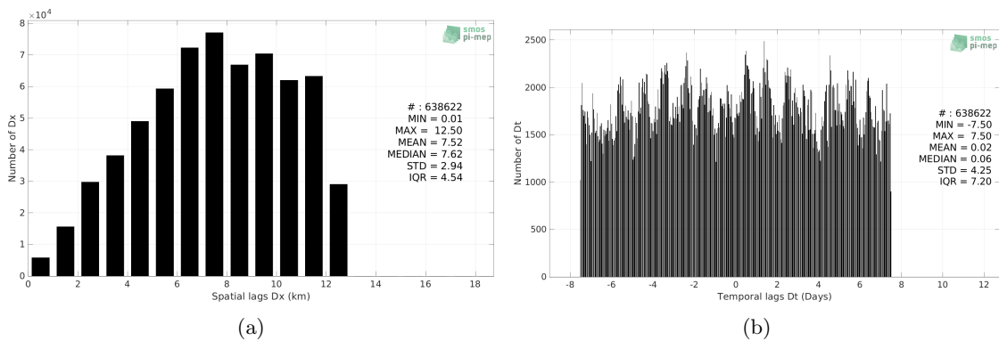
Figure 5: Histograms of the spatial (a) and temporal (b) lags between the location/time of the ICES measurement and the date of the corresponding CCI SSS L4 Merged-OI v3.2 - 30-day running (ESA) SSS pixel.
