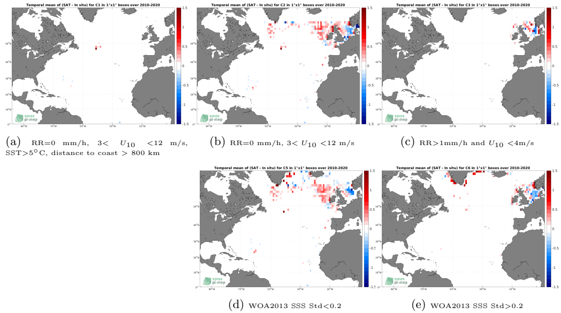
Figure 12: Temporal mean gridded over spatial boxes of size 1^\circ \times 1^\circ of \Delta SSS (CCI SSS L4 Merged-OI v3.2 - 30-day running (ESA) - ICES) for 5 different subdatasets corresponding to:RR=0 mm/h, 3 < U_{10} < 12 m/s, SST >5^\circ C, distance to coast > 800 km (a), RR=0 mm/h, 3 < U_{10} < 12 m/s (b), RR >1 mm/h and U_{10} < 4 m/s (c), WOA2013 SSS Std <0.2 (d), WOA2013 SSS Std >0.2 (e).
