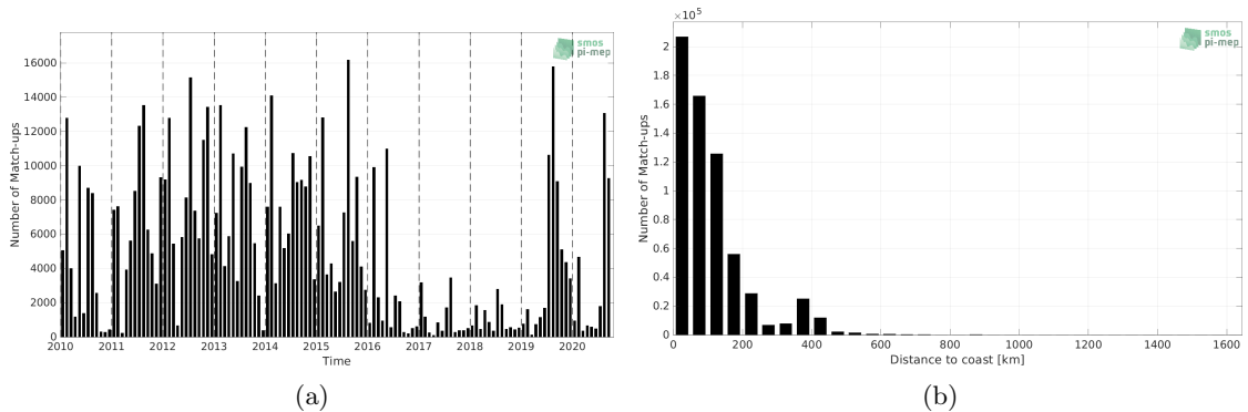
Figure 1: Number of match-ups between ICES and CCI SSS L4 Merged-OI v3.2 - 30-day running (ESA) SSS as a function of time (a) and as function of the distance to coast (b) over the North Atlantic Ocean Pi-MEP region and for the full satellite product period.
