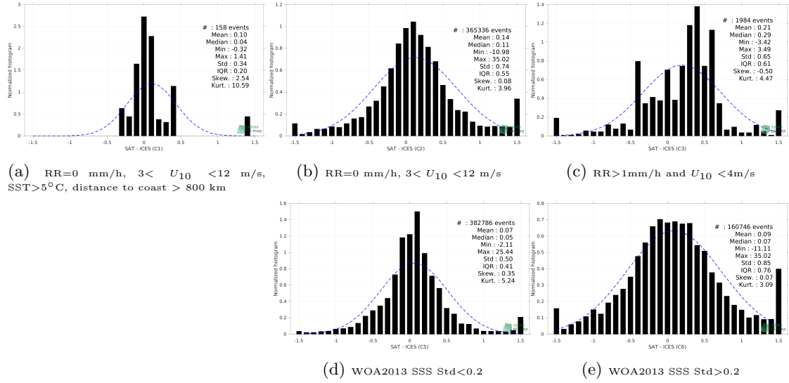
Figure 13: Normalized histogram of \Delta SSS (CCI SSS L4 Merged-OI v3.2 - 30-day running (ESA) - ICES) for 5 different subdatasets corresponding to: RR=0 mm/h, 3 < U_{10} < 12 m/s, SST > 5°C, distance to coast > 800 km (a), RR=0 mm/h, 3 < U_{10} < 12 m/s (b), RR > 1mm/h and U_{10} < 4 m/s (c), WOA2013 SSS Std < 0.2 (d), WOA2013 SSS Std > 0.2 (e).
