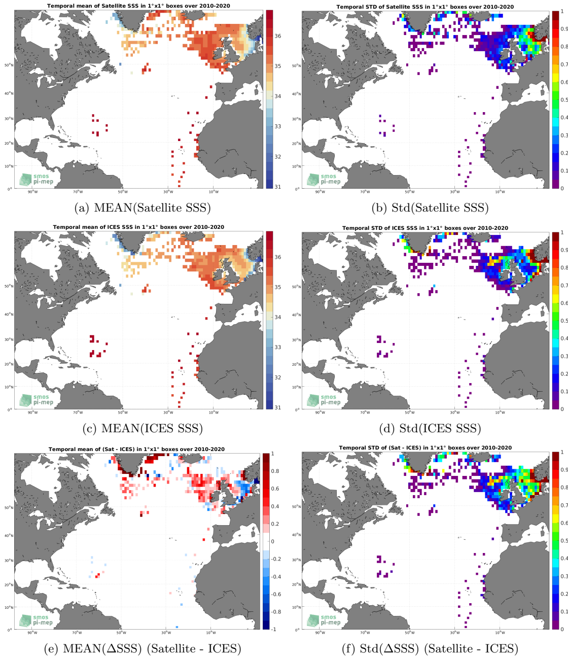
Figure 6: Temporal mean (left) and Std (right) of SSS from CCI SSS L4 Merged-OI v3.2 - 30-day running (ESA) (top), ICES (middle), and of \Delta SSS (Satellite - ICES). Only match-up pairs are used to generate these maps.
