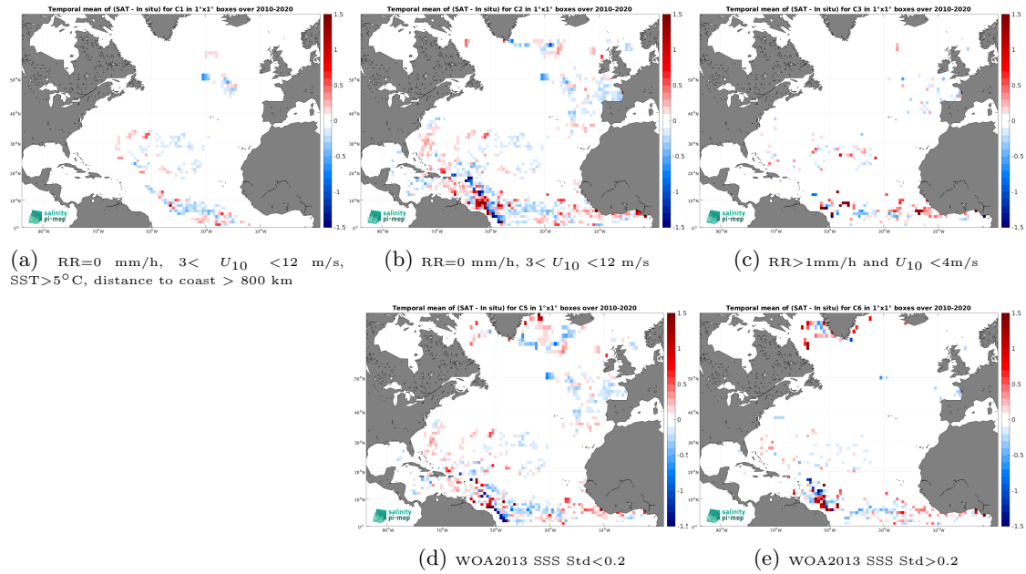
Figure 11: Temporal mean gridded over spatial boxes of size 1^\circ \times 1^\circ of \Delta\text{SSS} (CCI SSS L4 Merged-OI v3.2 - 30-day running (ESA) - Surface drifters) for 5 different subdatasets corresponding to:RR=0 mm/h, 3 < U_{10} < 12 m/s, SST >5^\circ\text{C} , distance to coast > 800 km (a), RR=0 mm/h, 3 < U_{10} < 12 m/s (b), RR >1 mm/h and U_{10} < 4 m/s (c), WOA2013 SSS Std <0.2 (d), WOA2013 SSS Std >0.2 (e).
