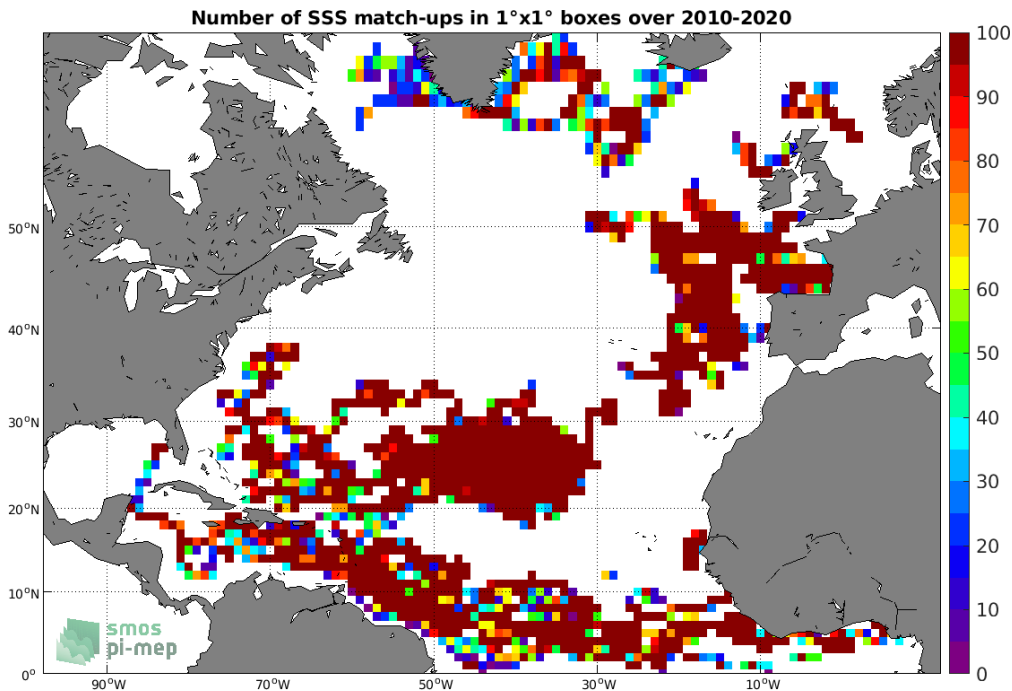
Figure 3: Number of SSS match-ups between Surface drifters SSS and the CCI SSS L4 Merged-OI v3.2 - 30-day running (ESA) SSS product for the North Atlantic Ocean Pi-MEP region over 1^\circ \times 1^\circ boxes and for the full satellite product period.
