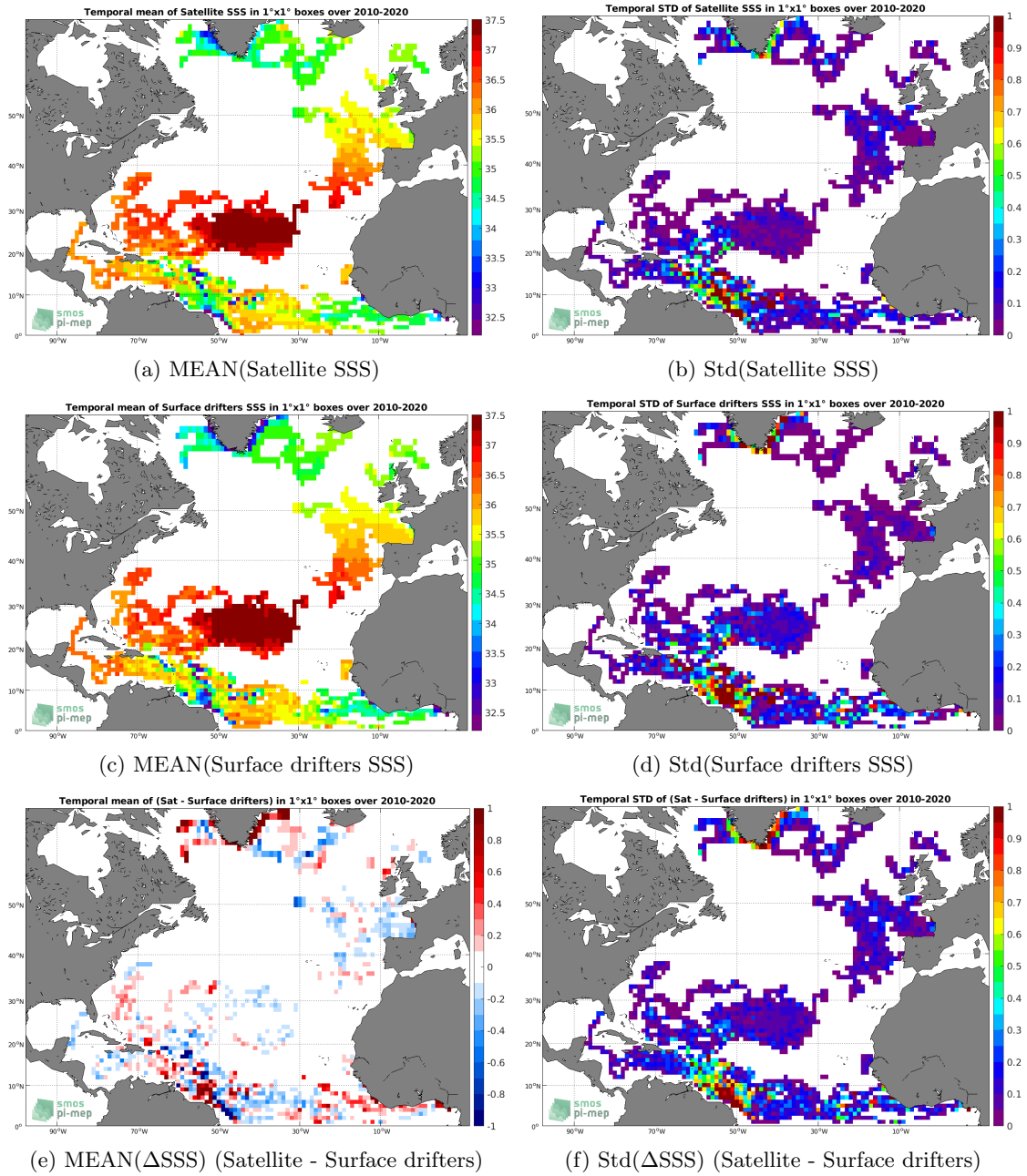
Figure 5: Temporal mean (left) and Std (right) of SSS from CCI SSS L4 Merged-OI v3.2 - 30-day running (ESA) (top), Surface drifters (middle), and of \Delta SSS (Satellite - Surface drifters). Only match-up pairs are used to generate these maps.
