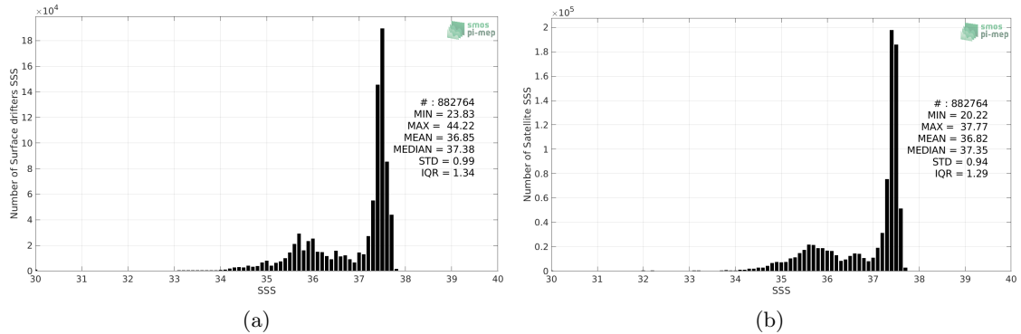
Figure 2: Histograms of SSS from Surface drifters (a) and CCI SSS L4 Merged-OI v3.2 - 30-day running (ESA) (b) considering all match-up pairs per bins of 0.1 over the North Atlantic Ocean Pi-MEP region and for the full satellite product period.
