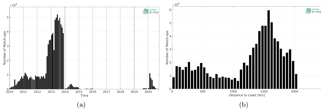
Figure 1: Number of match-ups between Surface drifters and CCI SSS L4 Merged-OI v3.2 - 30-day running (ESA) SSS as a function of time (a) and as function of the distance to coast (b) over the North Atlantic Ocean Pi-MEP region and for the full satellite product period.
