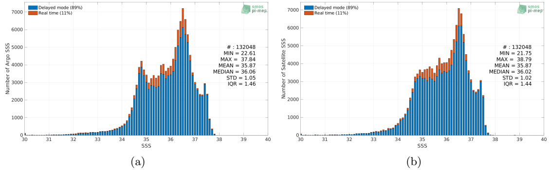
Figure 2: Histograms of SSS from Argo (a) and CCI SSS L4 Merged-OI v3.2 - 30-day running (ESA) (b) considering all match-up pairs per bins of 0.1 over the North Atlantic Ocean Pi-MEP region and for the full satellite product period.
