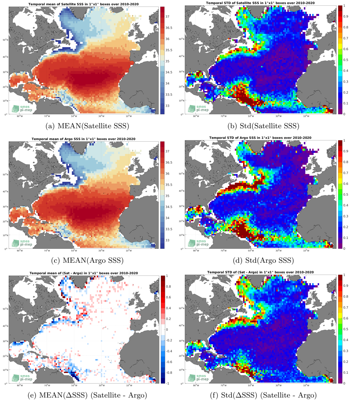
Figure 6: Temporal mean (left) and Std (right) of SSS from CCI SSS L4 Merged-OI v3.2 - 30-day running (ESA) (top), Argo (middle), and of \Delta SSS (Satellite - Argo). Only match-up pairs are used to generate these maps.
