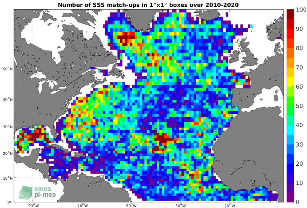
Figure 4: Number of SSS match-ups between Argo SSS and the CCI SSS L4 Merged-OI v3.2 - 30-day running (ESA) SSS product for the North Atlantic Ocean Pi-MEP region over 1^\circ \times 1^\circ boxes and for the full satellite product period.
