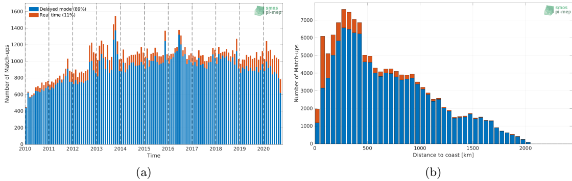
Figure 1: Number of match-ups between Argo and CCI SSS L4 Merged-OI v3.2 - 30-day running (ESA) SSS as a function of time (a) and as function of the distance to coast (b) over the North Atlantic Ocean Pi-MEP region and for the full satellite product period.
