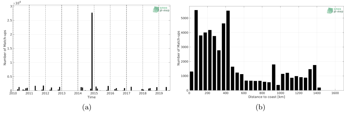
Figure 1: Number of match-ups between TSG (Polarstern) and CCI SSS L4 Merged-OI v2.31 - 7-day running (ESA) SSS as a function of time (a) and as function of the distance to coast (b) over the North Atlantic Ocean Pi-MEP region and for the full satellite product period.
