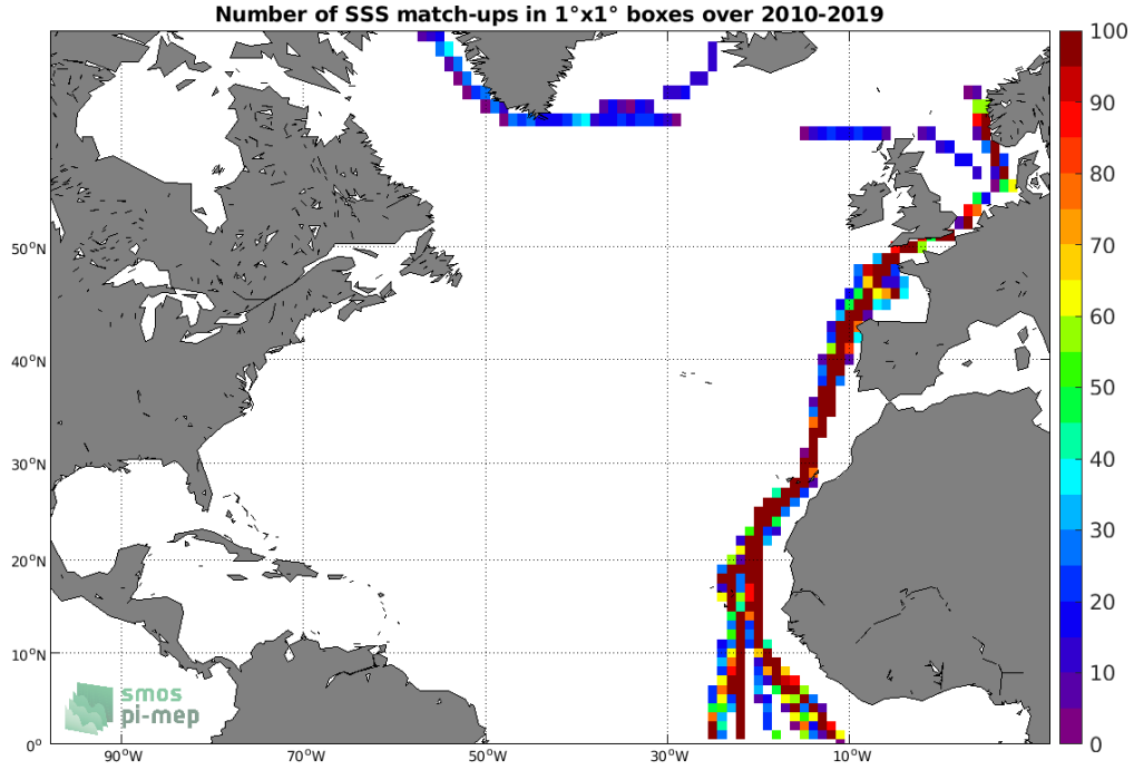
Figure 4: Number of SSS match-ups between TSG (Polarstern) SSS and the CCI SSS L4 Merged-OI v2.31 - 7-day running (ESA) SSS product for the North Atlantic Ocean Pi-MEP region over 1^\circ \times 1^\circ boxes and for the full satellite product period.
