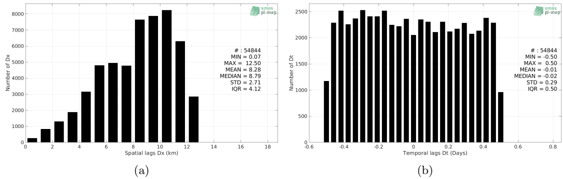
Figure 5: Histograms of the spatial (a) and temporal (b) lags between the location/time of the TSG (Polarstern) measurement and the date of the corresponding CCI SSS L4 Merged-OI v2.31 - 7-day running (ESA) SSS pixel.
