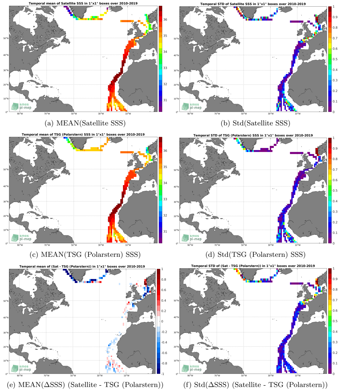
Figure 6: Temporal mean (left) and Std (right) of SSS from CCI SSS L4 Merged-OI v2.31 - 7-day running (ESA) (top), TSG (Polarstern) (middle), and of \Delta SSS (Satellite - TSG (Polarstern)). Only match-up pairs are used to generate these maps.
