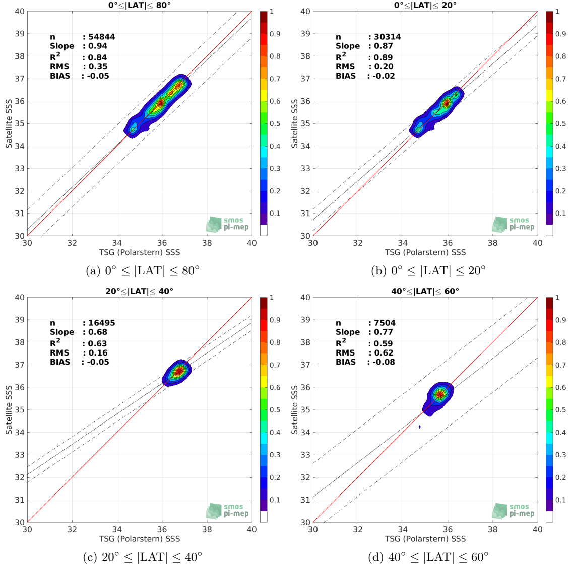
Figure 9: Contour maps of the concentration of CCI SSS L4 Merged-OI v2.31 - 7-day running (ESA) SSS (y-axis) versus TSG (Polarstern) SSS (x-axis) at match-up pairs for different latitude bands. For each plot, the red line shows x=y . The black thin and dashed lines indicate a linear fit through the data cloud and the \pm 95\% confidence levels, respectively. The number match-up pairs n , the slope and R^2 coefficient of the linear fit, the root mean square (RMS) and the mean bias between satellite and in situ data are indicated for each latitude band in each plots.
