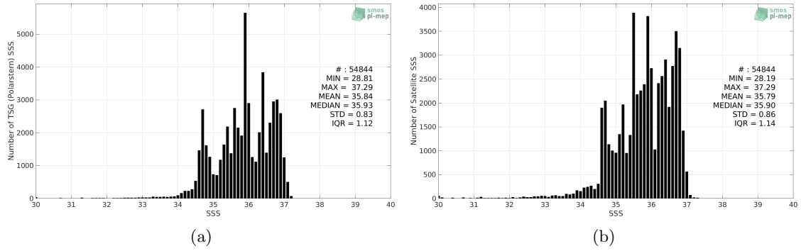
Figure 2: Histograms of SSS from TSG (Polarstern) (a) and CCI SSS L4 Merged-OI v2.31 - 7-day running (ESA) (b) considering all match-up pairs per bins of 0.1 over the North Atlantic Ocean Pi-MEP region and for the full satellite product period.
