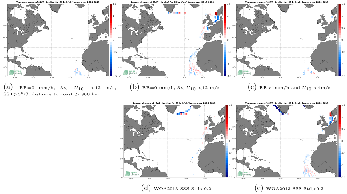
Figure 12: Temporal mean gridded over spatial boxes of size 1^\circ \times 1^\circ of \Delta SSS (CCI SSS L4 Merged-OI v2.31 - 7-day running (ESA) - TSG (Polarstern)) for 5 different subdatasets corresponding to: RR=0 mm/h, 3 < U_{10} < 12 m/s, SST > 5^\circ\text{C} , distance to coast > 800 km (a), RR=0 mm/h, 3 < U_{10} < 12 m/s (b), RR > 1\text{mm/h} and U_{10} < 4\text{m/s} (c), WOA2013 SSS Std < 0.2 (d), WOA2013 SSS Std > 0.2 (e).
