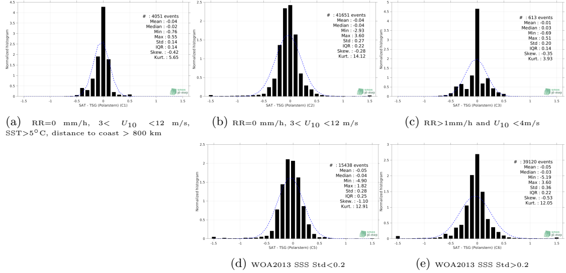
Figure 13: Normalized histogram of \Delta\text{SSS} (CCI SSS L4 Merged-OI v2.31 - 7-day running (ESA) - TSG (Polarstern)) for 5 different subdatasets corresponding to: RR=0 mm/h, 3 < U_{10} < 12 m/s, SST > 5^\circ\text{C} , distance to coast > 800 km (a), RR=0 mm/h, 3 < U_{10} < 12 m/s (b), RR > 1\text{mm/h} and U_{10} < 4\text{m/s} (c), WOA2013 SSS Std <0.2 (d), WOA2013 SSS Std >0.2 (e).
