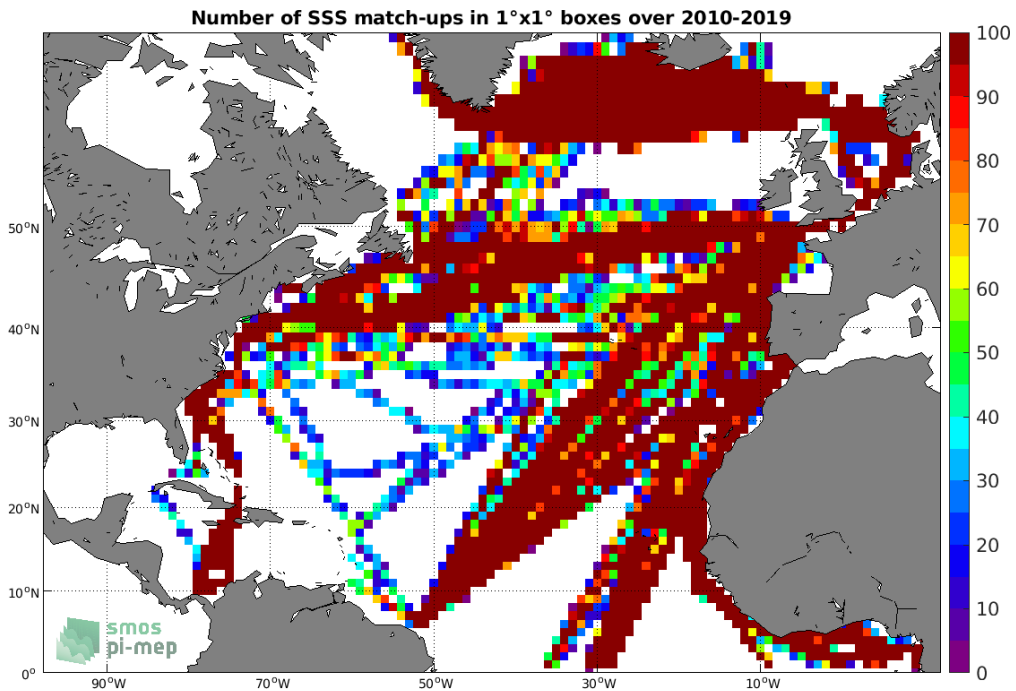
Figure 4: Number of SSS match-ups between TSG (LEGOS-DM) SSS and the CCI SSS L4 Merged-OI v2.31 - 7-day running (ESA) SSS product for the North Atlantic Ocean Pi-MEP region over 1°x1° boxes and for the full satellite product period.
