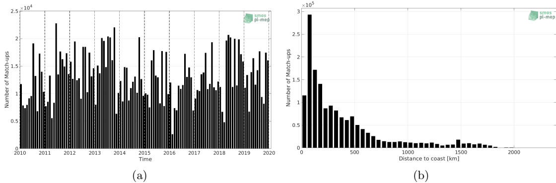
Figure 1: Number of match-ups between TSG (LEGOS-DM) and CCI SSS L4 Merged-OI v2.31 - 7-day running (ESA) SSS as a function of time (a) and as function of the distance to coast (b) over the North Atlantic Ocean Pi-MEP region and for the full satellite product period.
