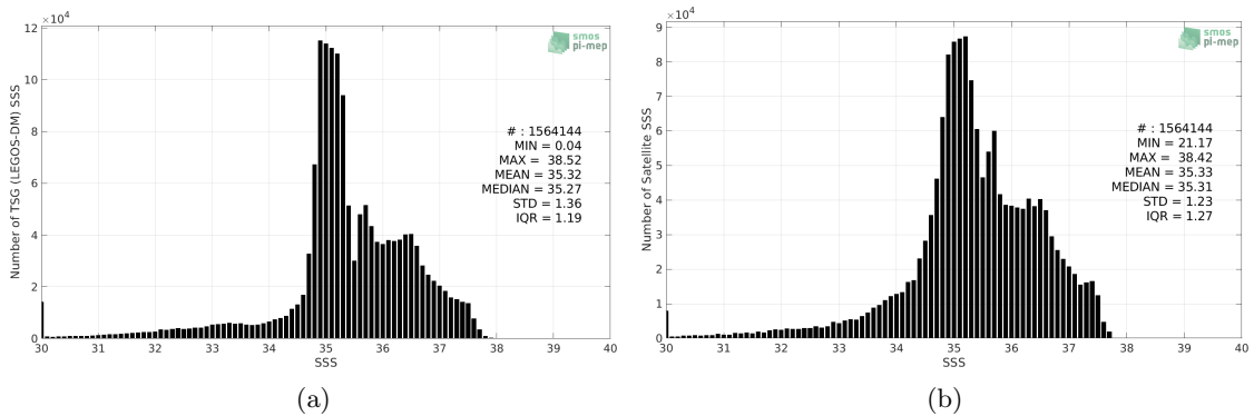
Figure 2: Histograms of SSS from TSG (LEGOS-DM) (a) and CCI SSS L4 Merged-OI v2.31 - 7-day running (ESA) (b) considering all match-up pairs per bins of 0.1 over the North Atlantic Ocean Pi-MEP region and for the full satellite product period.
