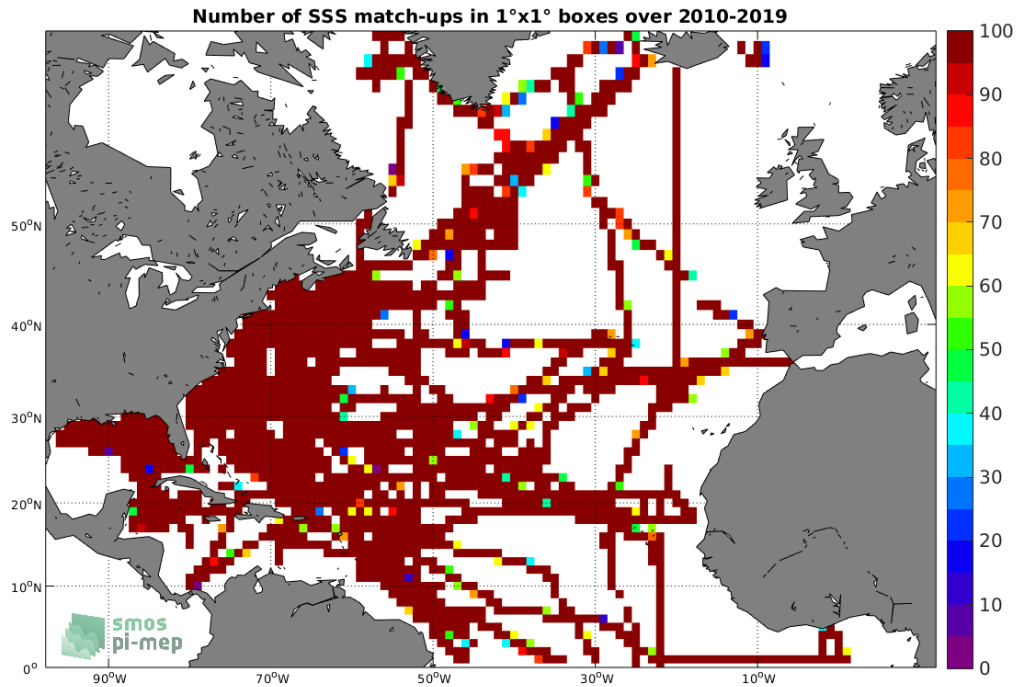
Figure 4: Number of SSS match-ups between TSG (SAMOS) SSS and the CCI SSS L4 Merged-OI v2.31 - 30-day running (ESA) SSS product for the North Atlantic Ocean Pi-MEP region over 1^\circ \times 1^\circ boxes and for the full satellite product period.
