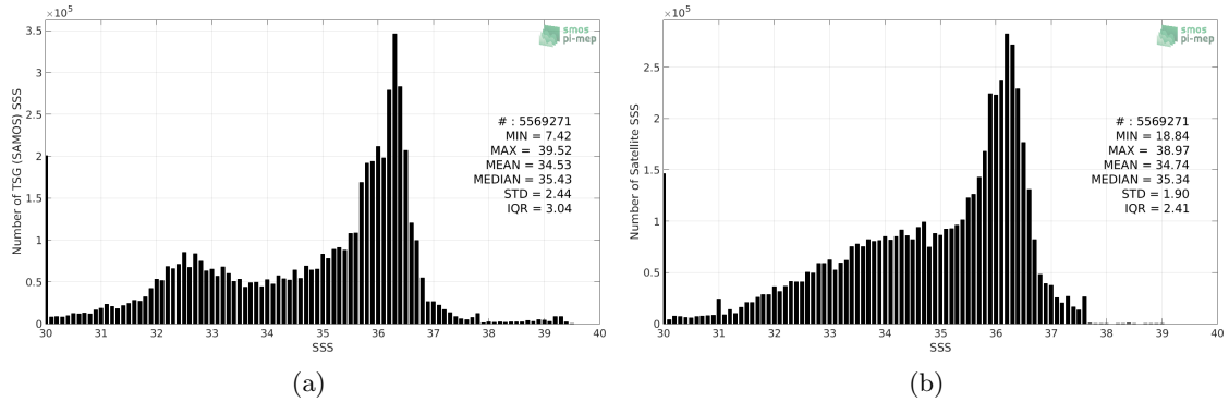
Figure 2: Histograms of SSS from TSG (SAMOS) (a) and CCI L4 Merged-OI v2.31 - 30-day running (ESA) (b) considering all match-up pairs per bins of 0.1 over the North Atlantic Ocean Pi-MEP region and for the full satellite product period.
