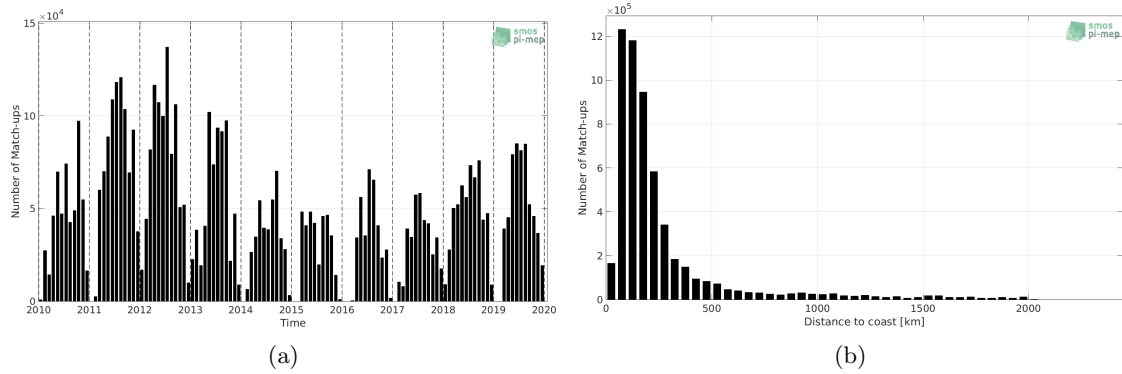
Figure 1: Number of match-ups between TSG (SAMOS) and CCI L4 Merged-OI v2.31 - 30-day running (ESA) SSS as a function of time (a) and as function of the distance to coast (b) over the North Atlantic Ocean Pi-MEP region and for the full satellite product period.
