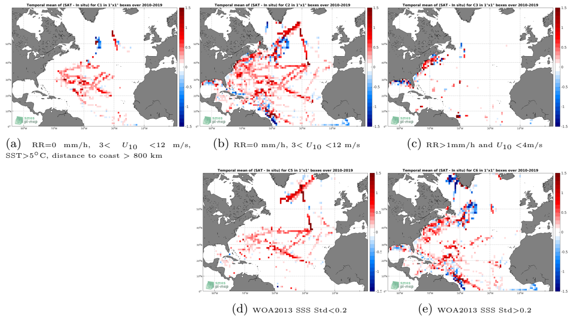
Figure 12: Temporal mean gridded over spatial boxes of size 1^\circ \times 1^\circ of \Delta SSS (CCI L4 Merged-OI v2.31 - 30-day running (ESA) - TSG (SAMOS)) for 5 different subdatasets corresponding to: RR=0 mm/h, 3 < U_{10} < 12 m/s, SST >5^\circ\text{C} , distance to coast > 800 km (a), RR=0 mm/h, 3 < U_{10} < 12 m/s (b), RR >1 mm/h and U_{10} < 4 m/s (c), WOA2013 SSS Std <0.2 (d), WOA2013 SSS Std >0.2 (e).
