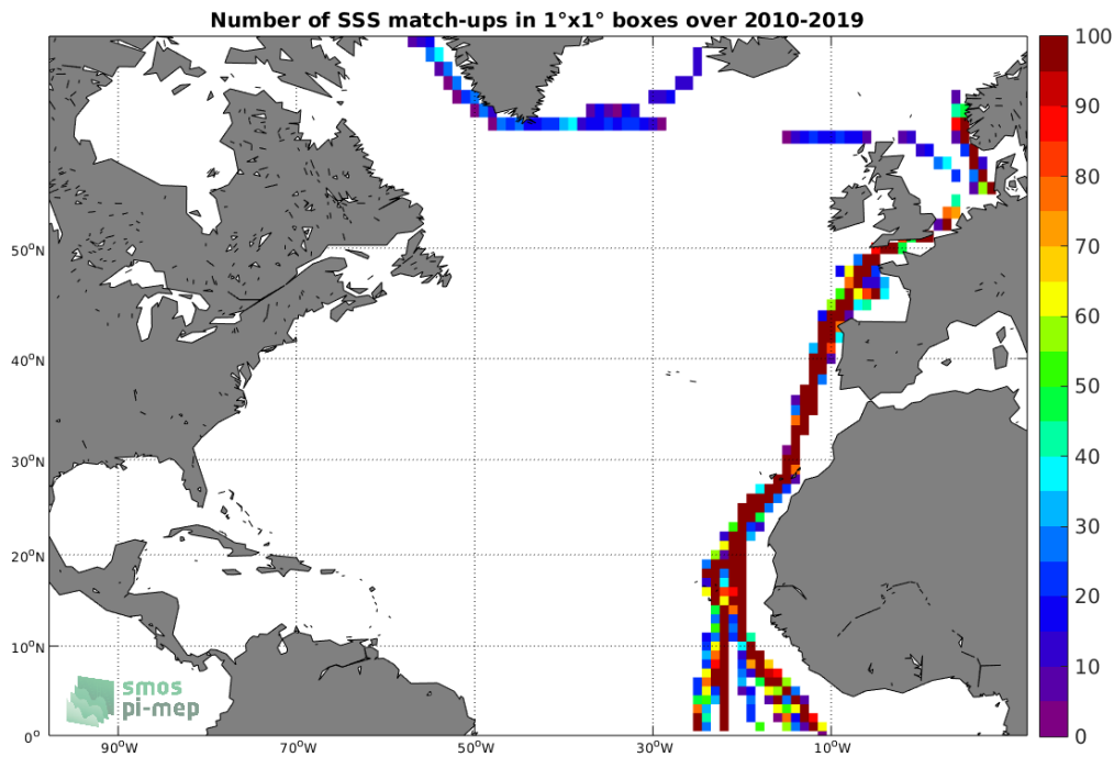
Figure 4: Number of SSS match-ups between TSG (Polarstern) SSS and the CCI L4 Merged-OI v2.31 - 30-day running (ESA) SSS product for the North Atlantic Ocean Pi-MEP region over 1°x1° boxes and for the full satellite product period.
