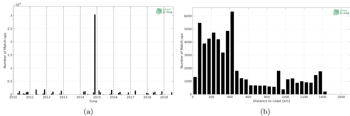
Figure 1: Number of match-ups between TSG (Polarstern) and CCI L4 Merged-OI v2.31 - 30-day running (ESA) SSS as a function of time (a) and as function of the distance to coast (b) over the North Atlantic Ocean Pi-MEP region and for the full satellite product period.
