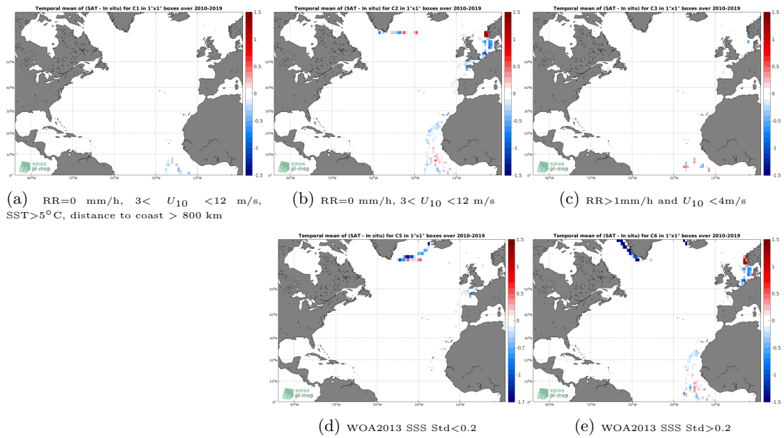
Figure 12: Temporal mean gridded over spatial boxes of size 1°x1° of \Delta SSS (CCI L4 Merged-OI v2.31 - 30-day running (ESA) - TSG (Polarstern)) for 5 different subdatasets corresponding to: RR=0 mm/h, 3 < U_{10} < 12 m/s, SST > 5°C, distance to coast > 800 km (a), RR=0 mm/h, 3 < U_{10} < 12 m/s (b), RR > 1mm/h and U_{10} < 4 m/s (c), WOA2013 SSS Std < 0.2 (d), WOA2013 SSS Std > 0.2 (e).
