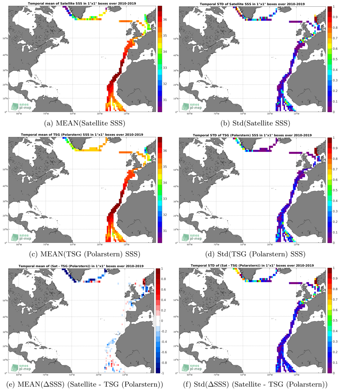
Figure 6: Temporal mean (left) and Std (right) of SSS from CCI L4 Merged-OI v2.31 - 30-day running (ESA) (top), TSG (Polarstern) (middle), and of \Delta SSS (Satellite - TSG (Polarstern)). Only match-up pairs are used to generate these maps.
