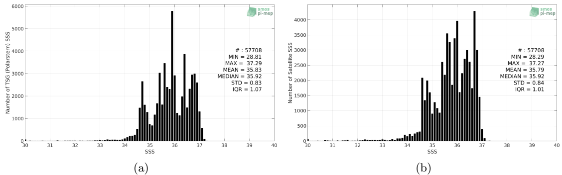
Figure 2: Histograms of SSS from TSG (Polarstern) (a) and CCI L4 Merged-OI v2.31 - 30-day running (ESA) (b) considering all match-up pairs per bins of 0.1 over the North Atlantic Ocean Pi-MEP region and for the full satellite product period.
