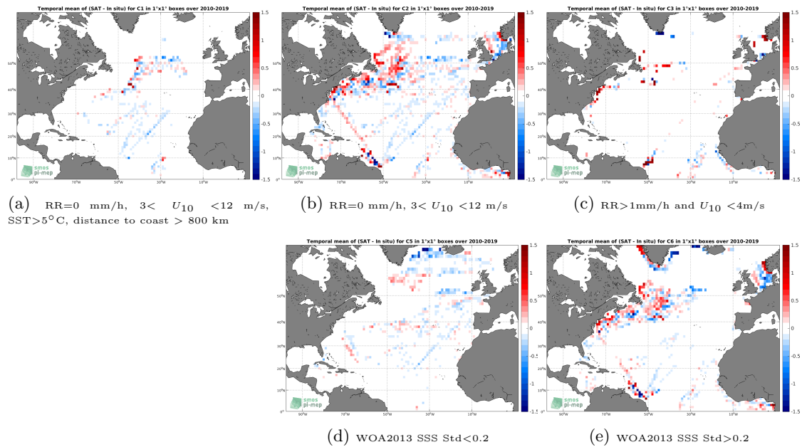
Figure 12: Temporal mean gridded over spatial boxes of size 1^\circ \times 1^\circ of \Delta\text{SSS} (CCI SSS L4 Merged-OI v2.31 - 30-day running (ESA) - TSG (LEGOS-DM)) for 5 different subdatasets corresponding to: RR=0 mm/h, 3 < U_{10} < 12 m/s, SST > 5^\circ\text{C} , distance to coast > 800 km (a), RR=0 mm/h, 3 < U_{10} < 12 m/s (b), RR > 1 mm/h and U_{10} < 4 m/s (c), WOA2013 SSS Std < 0.2 (d), WOA2013 SSS Std > 0.2 (e).
