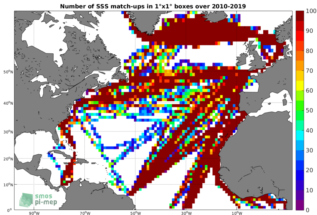
Figure 4: Number of SSS match-ups between TSG (LEGOS-DM) SSS and the CCI SSS L4 Merged-OI v2.31 - 30-day running (ESA) SSS product for the North Atlantic Ocean Pi-MEP region over 1^\circ \times 1^\circ boxes and for the full satellite product period.
