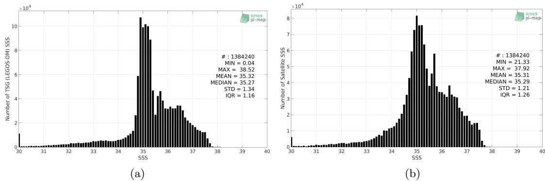
Figure 2: Histograms of SSS from TSG (LEGOS-DM) (a) and CCI SSS L4 Merged-OI v2.31 - 30-day running (ESA) (b) considering all match-up pairs per bins of 0.1 over the North Atlantic Ocean Pi-MEP region and for the full satellite product period.
