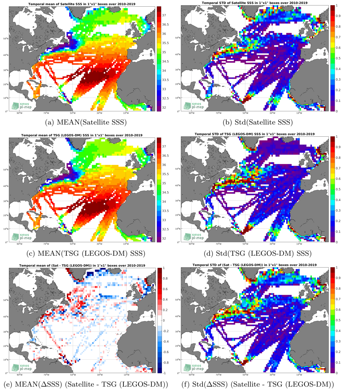
Figure 6: Temporal mean (left) and Std (right) of SSS from CCI SSS L4 Merged-OI v2.31 - 30-day running (ESA) (top), TSG (LEGOS-DM) (middle), and of \Delta SSS (Satellite - TSG (LEGOS-DM)). Only match-up pairs are used to generate these maps.
