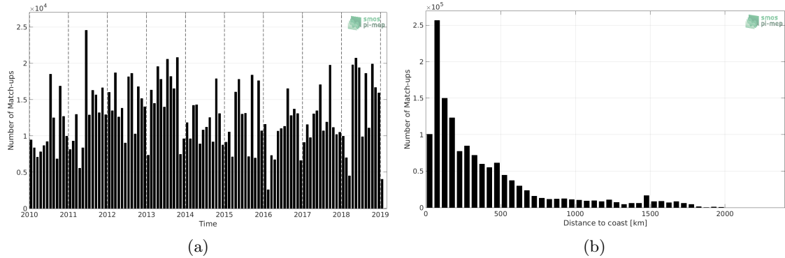
Figure 1: Number of match-ups between TSG (LEGOS-DM) and CCI SSS L4 Merged-OI v2.31 - 30-day running (ESA) SSS as a function of time (a) and as function of the distance to coast (b) over the North Atlantic Ocean Pi-MEP region and for the full satellite product period.
