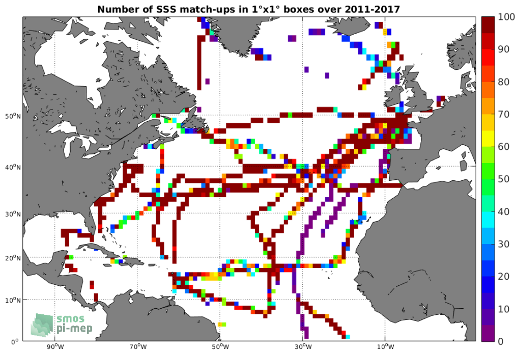
Figure 4: Number of SSS match-ups between TSG (GOSUD-Sailing-ship) SSS and the CCI L4 Merged-OI v2.31 - 30-day running (ESA) SSS product for the North Atlantic Ocean Pi-MEP region over 1^\circ \times 1^\circ boxes and for the full satellite product period.
