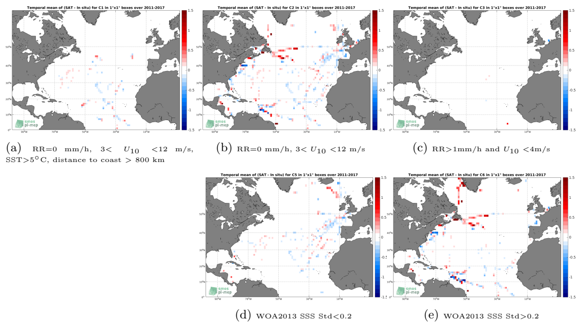
Figure 12: Temporal mean gridded over spatial boxes of size 1^\circ \times 1^\circ of \Delta SSS (CCI L4 Merged-OI v2.31 - 30-day running (ESA) - TSG (GOSUD-Sailing-ship)) for 5 different subdatasets corresponding to:RR=0 mm/h, 3 < U_{10} < 12 m/s, SST>5°C, distance to coast > 800 km (a), RR=0 mm/h, 3 < U_{10} < 12 m/s (b), RR>1mm/h and U_{10} < 4 m/s (c), WOA2013 SSS Std<0.2 (d), WOA2013 SSS Std>0.2 (e).
