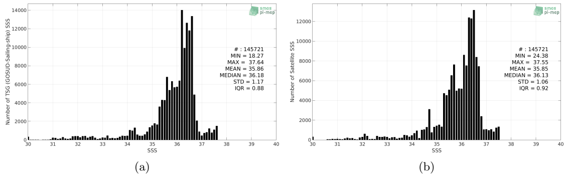
Figure 2: Histograms of SSS from TSG (GOSUD-Sailing-ship) (a) and CCI L4 Merged-OI v2.31 - 30-day running (ESA) (b) considering all match-up pairs per bins of 0.1 over the North Atlantic Ocean Pi-MEP region and for the full satellite product period.
