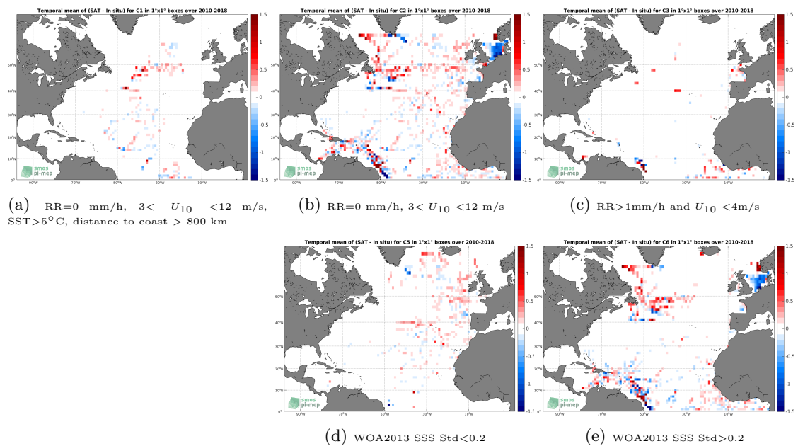
Figure 12: Temporal mean gridded over spatial boxes of size 1^\circ \times 1^\circ of \Delta\text{SSS} (CCI SSS L4 Merged-OI v2.31 - 30-day running (ESA) - TSG (GOSUD-Research-vessel)) for 5 different subdatasets corresponding to:RR=0 mm/h, 3 < U_{10} < 12 m/s, SST>5°C, distance to coast > 800 km (a), RR=0 mm/h, 3 < U_{10} < 12 m/s (b), RR>1mm/h and U_{10} < 4 m/s (c), WOA2013 SSS Std<0.2 (d), WOA2013 SSS Std>0.2 (e).
