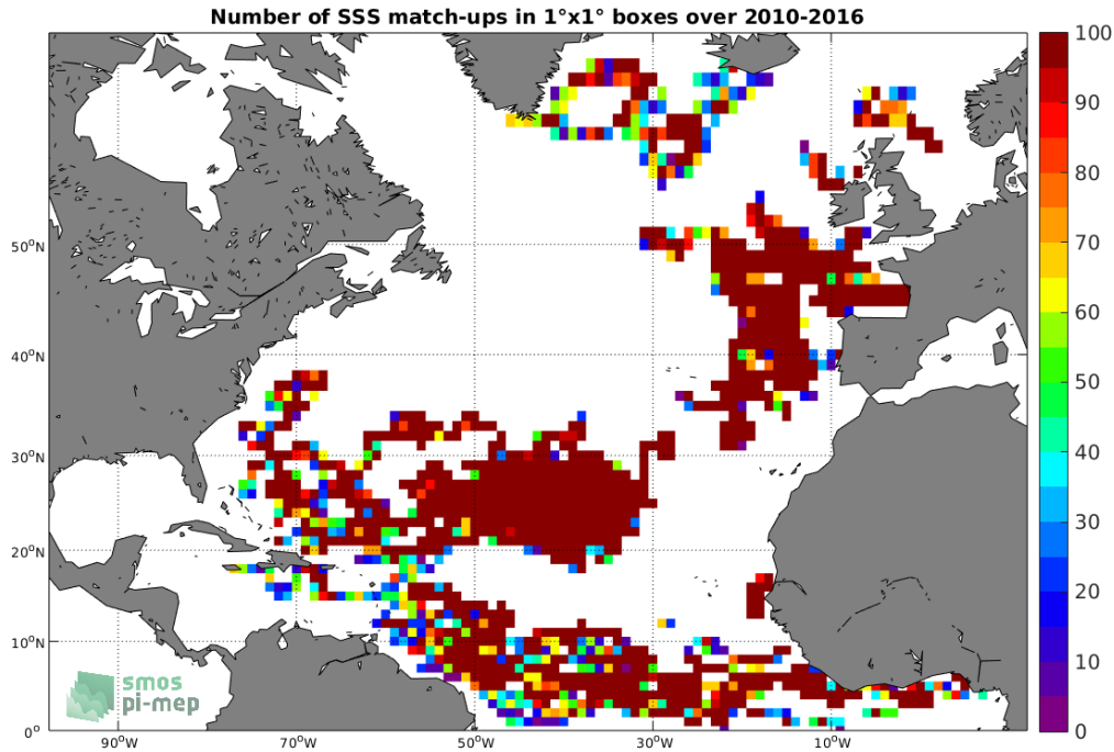
Figure 3: Number of SSS match-ups between Surface drifters SSS and the CCI SSS L4 Merged-OI v2.31 - 30-day running (ESA) SSS product for the North Atlantic Ocean Pi-MEP region over 1°x1° boxes and for the full satellite product period.
