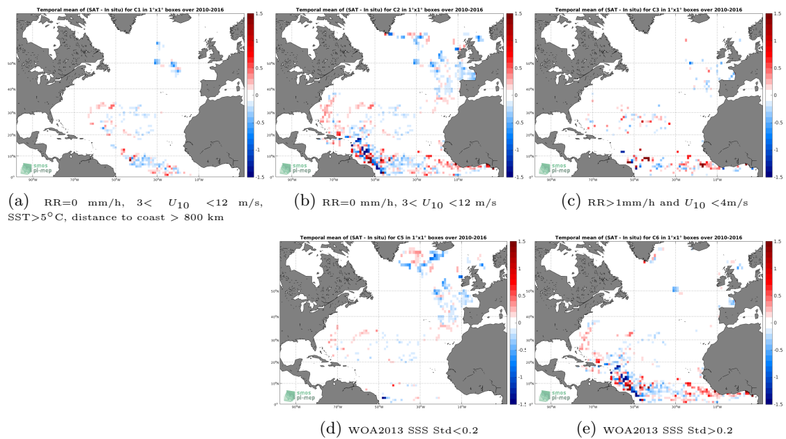
Figure 11: Temporal mean gridded over spatial boxes of size 1^\circ \times 1^\circ of \Delta\text{SSS} (CCI SSS L4 Merged-OI v2.31 - 30-day running (ESA) - Surface drifters) for 5 different subdatasets corresponding to:RR=0 mm/h, 3 < U_{10} < 12 m/s, SST > 5^\circ\text{C} , distance to coast > 800 km (a), RR=0 mm/h, 3 < U_{10} < 12 m/s (b), RR > 1 mm/h and U_{10} < 4 m/s (c), WOA2013 SSS Std < 0.2 (d), WOA2013 SSS Std > 0.2 (e).
