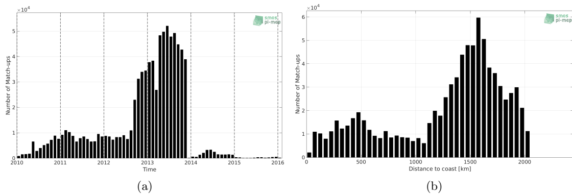
Figure 1: Number of match-ups between Surface drifters and CCI SSS L4 Merged-OI v2.31 - 30-day running (ESA) SSS as a function of time (a) and as function of the distance to coast (b) over the North Atlantic Ocean Pi-MEP region and for the full satellite product period.
