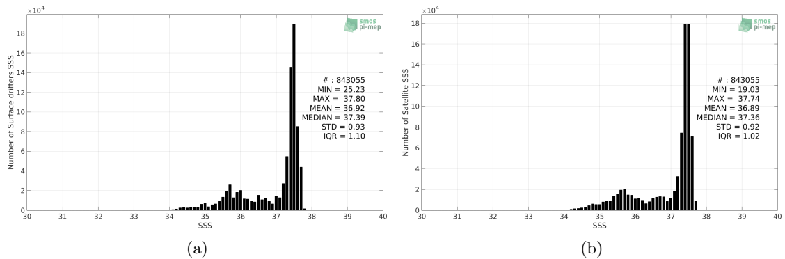
Figure 2: Histograms of SSS from Surface drifters (a) and CCI SSS L4 Merged-OI v2.31 - 30-day running (ESA) (b) considering all match-up pairs per bins of 0.1 over the North Atlantic Ocean Pi-MEP region and for the full satellite product period.
