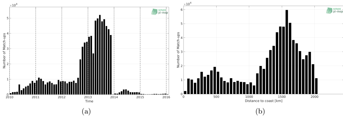
Figure 1: Number of match-ups between Surface drifters and CCI L4 Merged-OI v2.31 - 30-day running (ESA) SSS as a function of time (a) and as function of the distance to coast (b) over the North Atlantic Ocean Pi-MEP region and for the full satellite product period.
