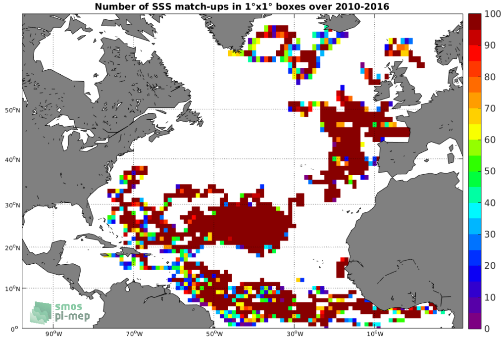
Figure 3: Number of SSS match-ups between Surface drifters SSS and the CCI L4 Merged-OI v2.31 - 30-day running (ESA) SSS product for the North Atlantic Ocean Pi-MEP region over 1°x1° boxes and for the full satellite product period.
