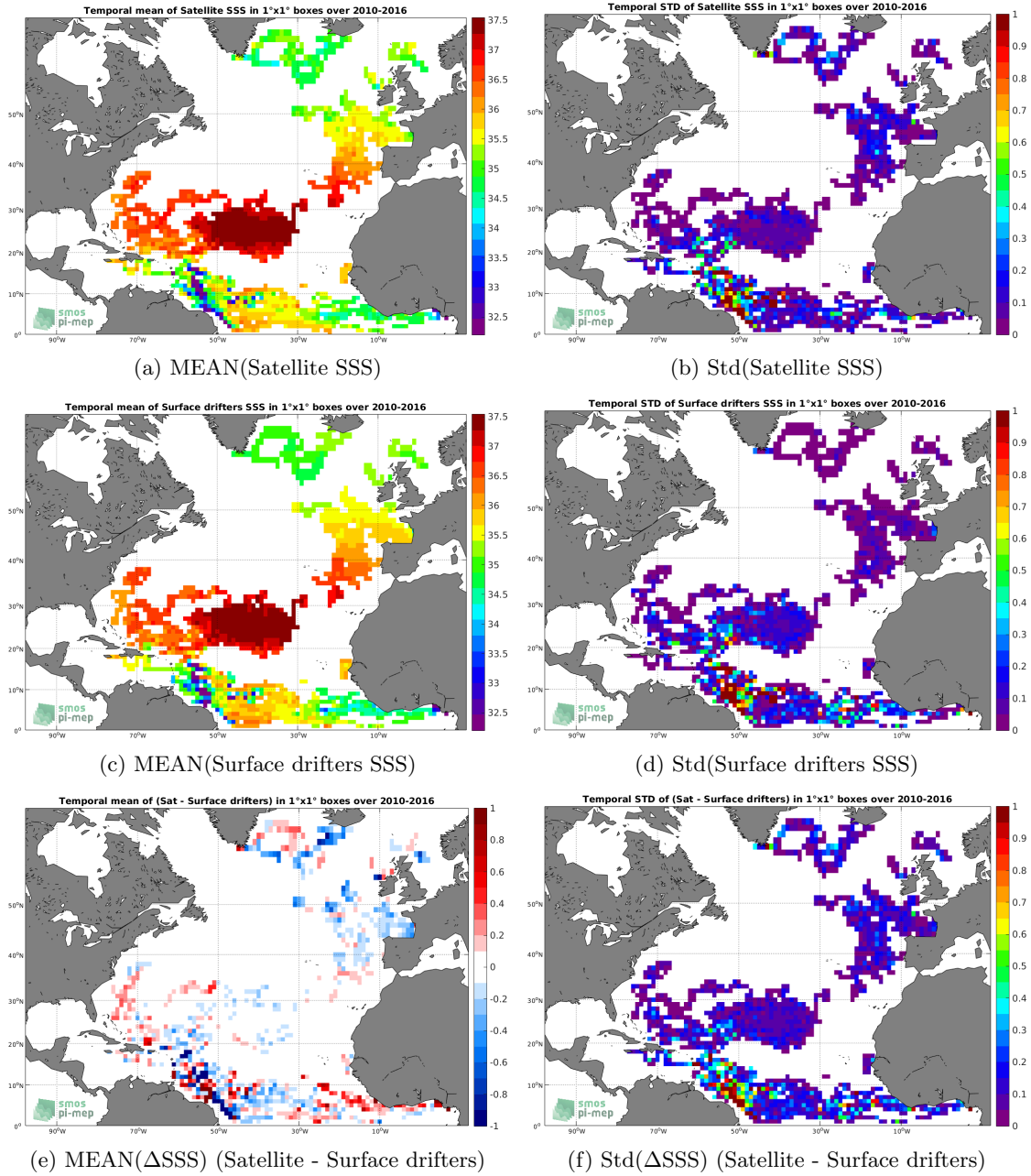
Figure 5: Temporal mean (left) and Std (right) of SSS from CCI L4 Merged-OI v2.31 - 30-day running (ESA) (top), Surface drifters (middle), and of \Delta SSS (Satellite - Surface drifters). Only match-up pairs are used to generate these maps.
