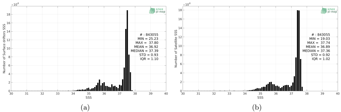
Figure 2: Histograms of SSS from Surface drifters (a) and CCI L4 Merged-OI v2.31 - 30-day running (ESA) (b) considering all match-up pairs per bins of 0.1 over the North Atlantic Ocean Pi-MEP region and for the full satellite product period.
