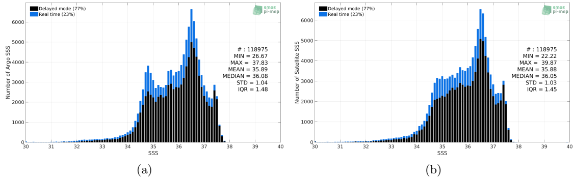
Figure 2: Histograms of SSS from Argo (a) and CCI SSS L4 Merged-OI v2.31 - 30-day running (ESA) (b) considering all match-up pairs per bins of 0.1 over the North Atlantic Ocean Pi-MEP region and for the full satellite product period.
