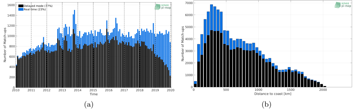
Figure 1: Number of match-ups between Argo and CCI SSS L4 Merged-OI v2.31 - 30-day running (ESA) SSS as a function of time (a) and as function of the distance to coast (b) over the North Atlantic Ocean Pi-MEP region and for the full satellite product period.
