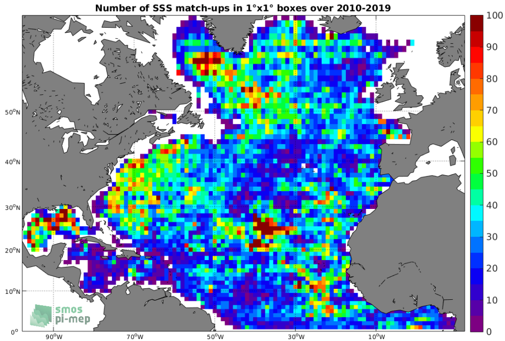
Figure 4: Number of SSS match-ups between Argo SSS and the CCI SSS L4 Merged-OI v2.31 - 30-day running (ESA) SSS product for the North Atlantic Ocean Pi-MEP region over 1^\circ \times 1^\circ boxes and for the full satellite product period.
