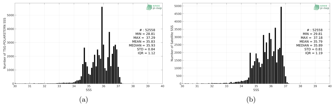
Figure 2: Histograms of SSS from TSG-POLARSTERN (a) and CCI L4 Merged-OI v1.8 - 7-day running (ESA) (b) considering all match-up pairs per bins of 0.1 over the North Atlantic Ocean Pi-MEP region and for the full satellite product period.
