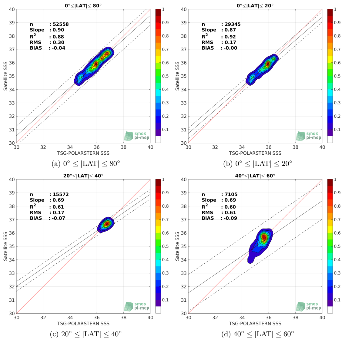
Figure 9: Contour maps of the concentration of CCI L4 Merged-OI v1.8 - 7-day running (ESA) SSS (y-axis) versus TSG-POLARSTERN SSS (x-axis) at match-up pairs for different latitude bands. For each plot, the red line shows x=y . The black thin and dashed lines indicate a linear fit through the data cloud and the \pm 95\% confidence levels, respectively. The number match-up pairs n , the slope and R^2 coefficient of the linear fit, the root mean square (RMS) and the mean bias between satellite and in situ data are indicated for each latitude band in each plots.
