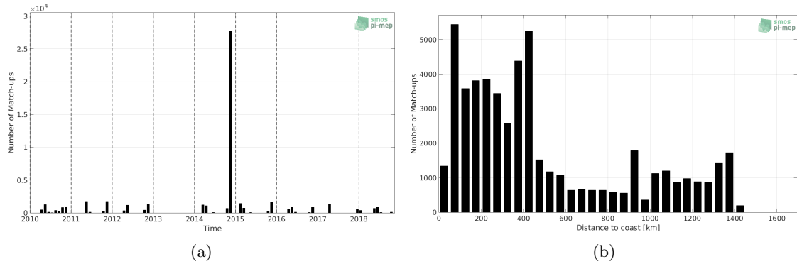
Figure 1: Number of match-ups between TSG-POLARSTERN and CCI L4 Merged-OI v1.8 - 7-day running (ESA) SSS as a function of time (a) and as function of the distance to coast (b) over the North Atlantic Ocean Pi-MEP region and for the full satellite product period.
