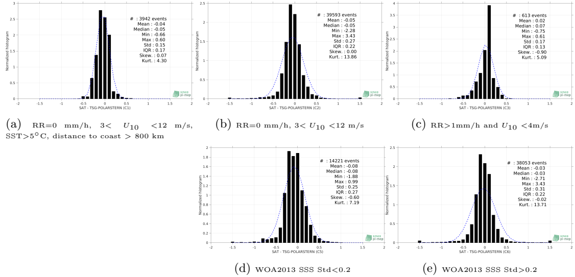
Figure 13: Normalized histogram of \Delta SSS (CCI L4 Merged-OI v1.8 - 7-day running (ESA) - TSG-POLARSTERN) for 5 different subdatasets corresponding to: RR=0 mm/h, 3 < U_{10} < 12 m/s, SST > 5°C, distance to coast > 800 km (a), RR=0 mm/h, 3 < U_{10} < 12 m/s (b), RR > 1mm/h and U_{10} < 4 m/s (c), WOA2013 SSS Std < 0.2 (d), WOA2013 SSS Std > 0.2 (e).
