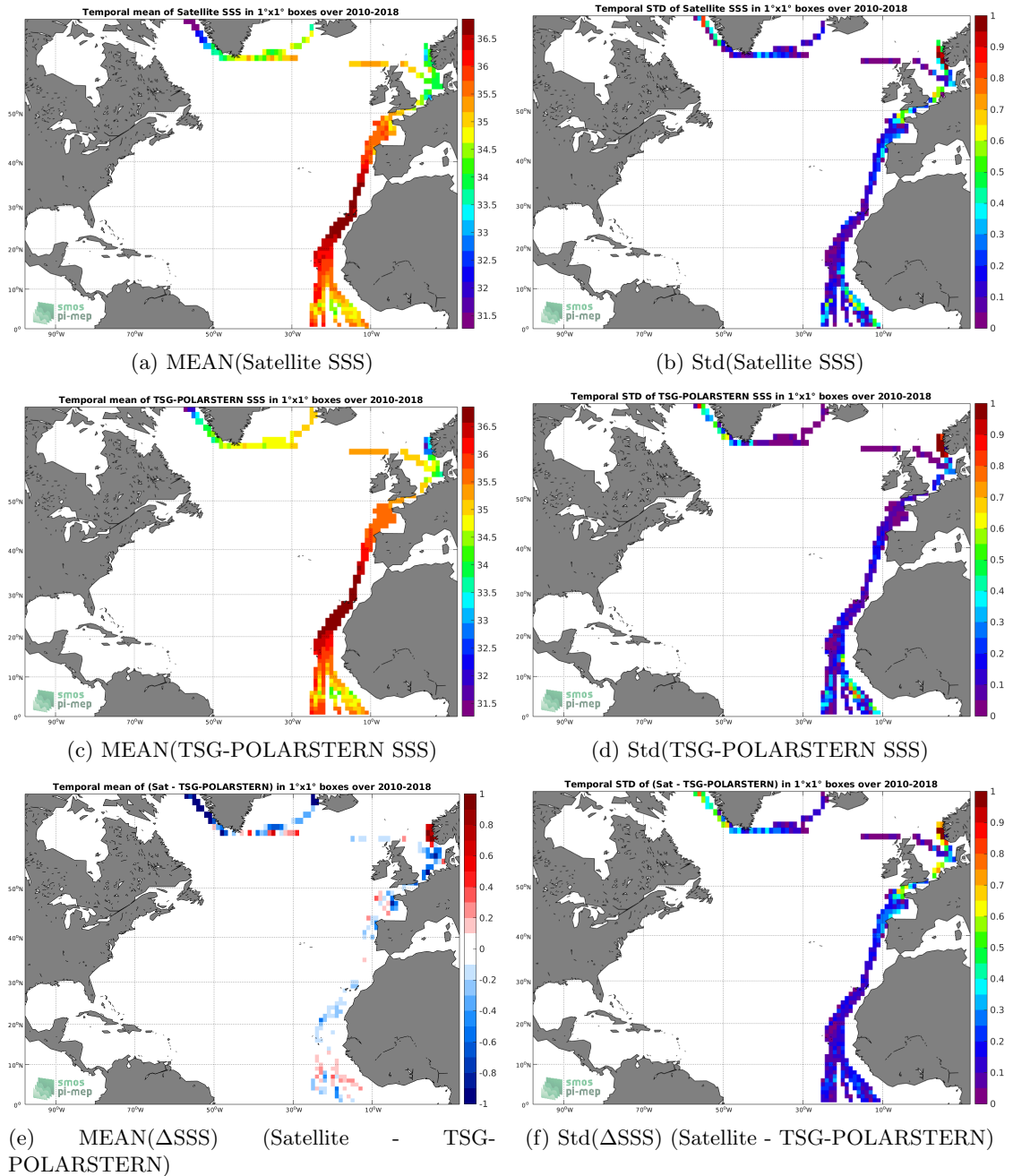
Figure 6: Temporal mean (left) and Std (right) of SSS from CCI L4 Merged-OI v1.8 - 7-day running (ESA) (top), TSG-POLARSTERN (middle), and of \Delta SSS (Satellite - TSG-POLARSTERN). Only match-up pairs are used to generate these maps.
