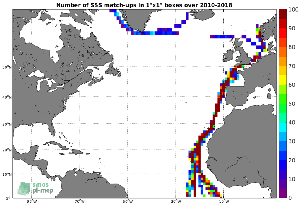
Figure 4: Number of SSS match-ups between TSG-POLARSTERN SSS and the CCI L4 Merged-OI v1.8 - 7-day running (ESA) SSS product for the North Atlantic Ocean Pi-MEP region over 1°x1° boxes and for the full satellite product period.
