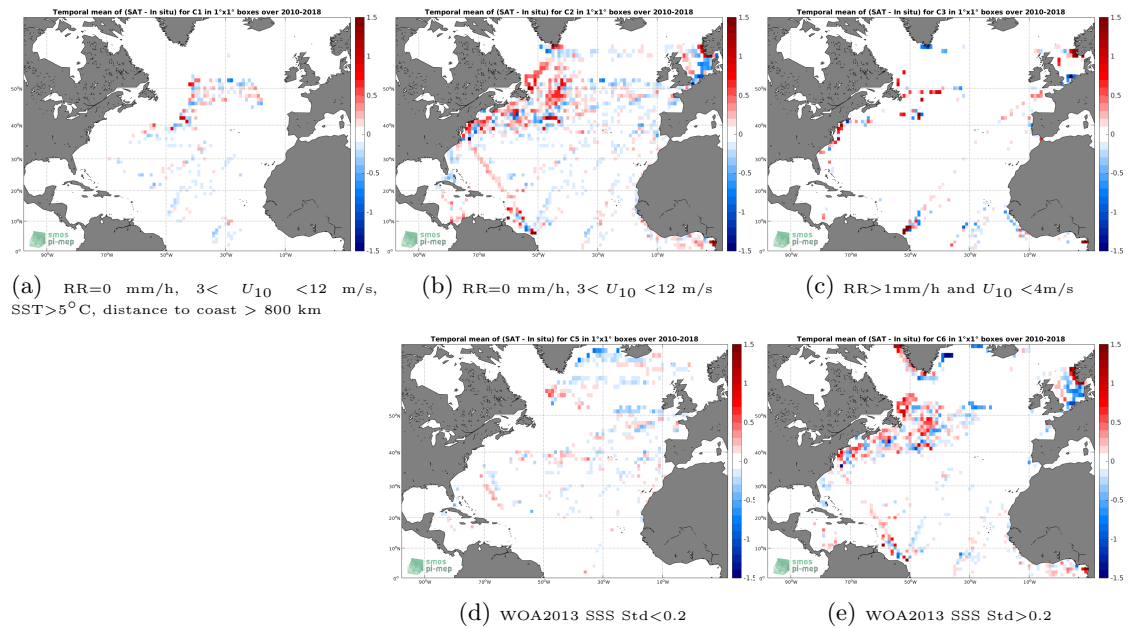
Figure 12: Temporal mean gridded over spatial boxes of size 1^\circ \times 1^\circ of \Delta SSS (CCI L4 Merged-OI v1.8 - 7-day running (ESA) - TSG-LEGOS-DM) for 5 different subdatasets corresponding to:RR=0 mm/h, 3 < U_{10} < 12 m/s, SST >5^\circ C, distance to coast > 800 km (a), RR=0 mm/h, 3 < U_{10} < 12 m/s (b), RR >1 mm/h and U_{10} < 4 m/s (c), WOA2013 SSS Std <0.2 (d), WOA2013 SSS Std >0.2 (e).
