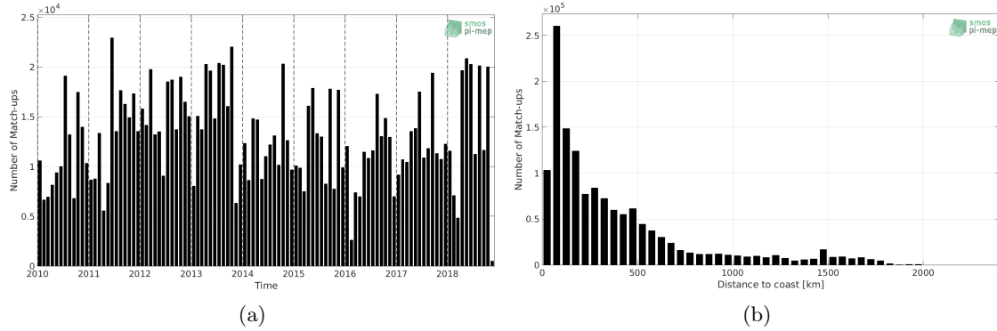
Figure 1: Number of match-ups between TSG-LEGOS-DM and CCI L4 Merged-OI v1.8 - 7-day running (ESA) SSS as a function of time (a) and as function of the distance to coast (b) over the North Atlantic Ocean Pi-MEP region and for the full satellite product period.
