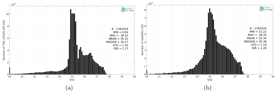
Figure 2: Histograms of SSS from TSG-LEGOS-DM (a) and CCI L4 Merged-OI v1.8 - 7-day running (ESA) (b) considering all match-up pairs per bins of 0.1 over the North Atlantic Ocean Pi-MEP region and for the full satellite product period.
