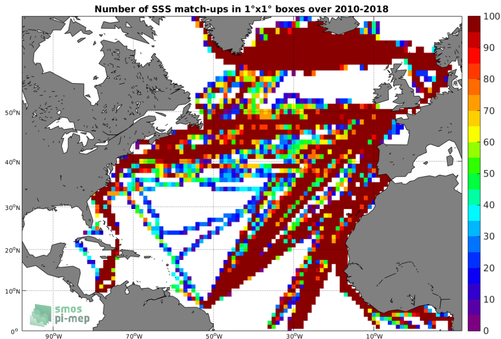
Figure 4: Number of SSS match-ups between TSG-LEGOS-DM SSS and the CCI L4 Merged-OI v1.8 - 7-day running (ESA) SSS product for the North Atlantic Ocean Pi-MEP region over 1^\circ \times 1^\circ boxes and for the full satellite product period.
