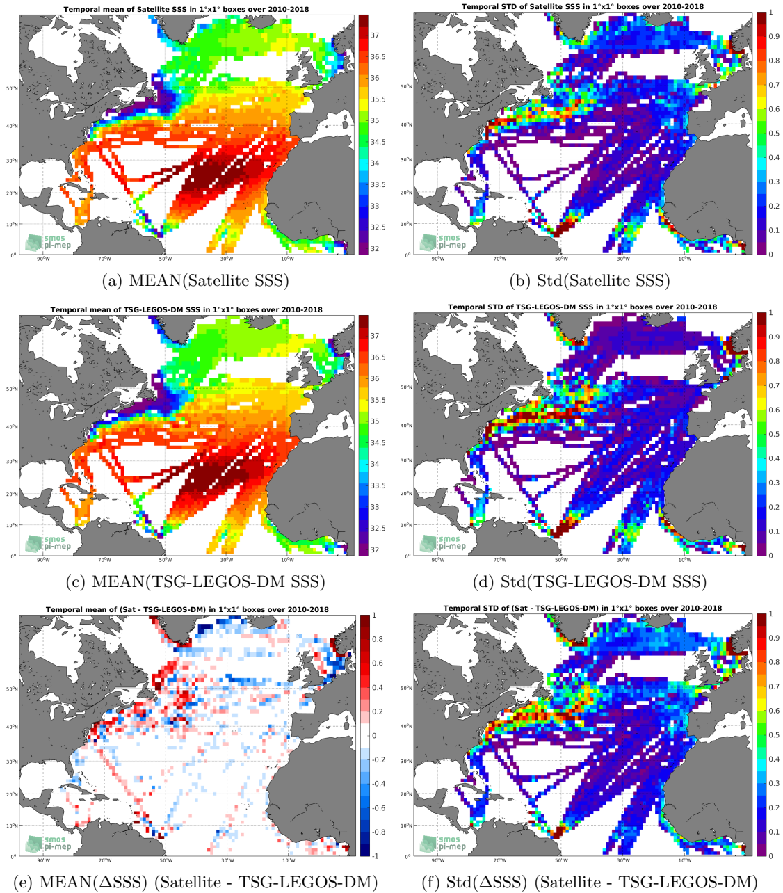
Figure 6: Temporal mean (left) and Std (right) of SSS from CCI L4 Merged-OI v1.8 - 7-day running (ESA) (top), TSG-LEGOS-DM (middle), and of \Delta SSS (Satellite - TSG-LEGOS-DM). Only match-up pairs are used to generate these maps.
