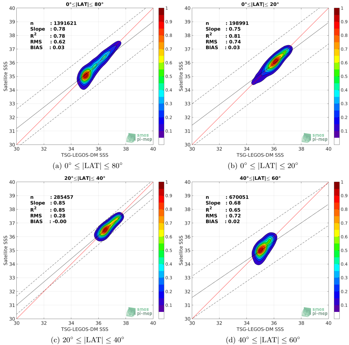
Figure 9: Contour maps of the concentration of CCI L4 Merged-OI v1.8 - 7-day running (ESA) SSS (y-axis) versus TSG-LEGOS-DM SSS (x-axis) at match-up pairs for different latitude bands. For each plot, the red line shows x=y . The black thin and dashed lines indicate a linear fit through the data cloud and the \pm 95\% confidence levels, respectively. The number match-up pairs n , the slope and R^2 coefficient of the linear fit, the root mean square (RMS) and the mean bias between satellite and in situ data are indicated for each latitude band in each plots.
