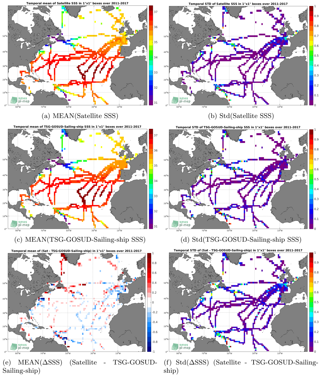
Figure 6: Temporal mean (left) and Std (right) of SSS from CCI L4 Merged-OI v1.8 - 7-day running (ESA) (top), TSG-GOSUD-Sailing-ship (middle), and of \Delta SSS (Satellite - TSG-GOSUD-Sailing-ship). Only match-up pairs are used to generate these maps.
