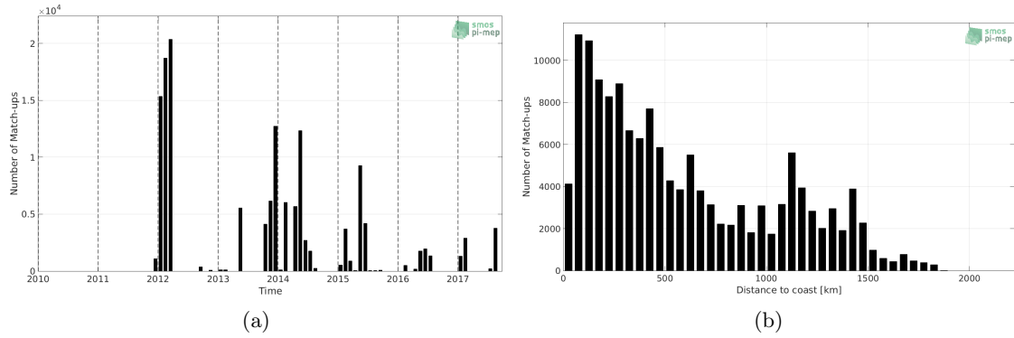
Figure 1: Number of match-ups between TSG-GOSUD-Sailing-ship and CCI L4 Merged-OI v1.8 - 7-day running (ESA) SSS as a function of time (a) and as function of the distance to coast (b) over the North Atlantic Ocean Pi-MEP region and for the full satellite product period.
