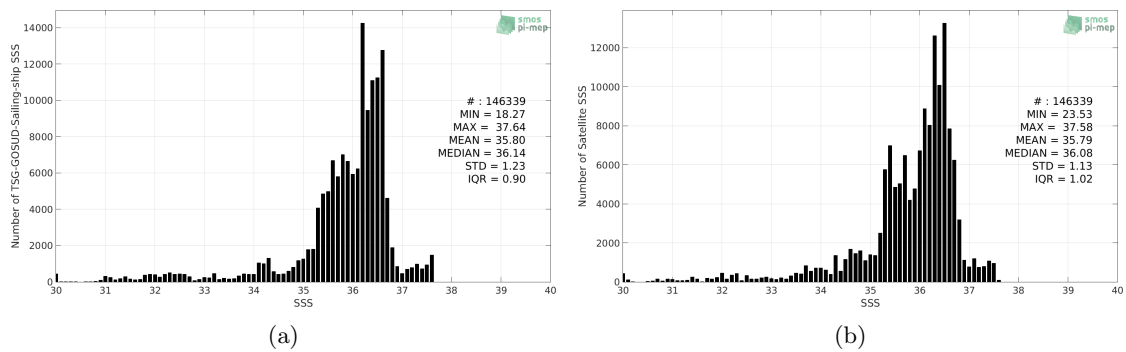
Figure 2: Histograms of SSS from TSG-GOSUD-Sailing-ship (a) and CCI L4 Merged-OI v1.8 - 7-day running (ESA) (b) considering all match-up pairs per bins of 0.1 over the North Atlantic Ocean Pi-MEP region and for the full satellite product period.
