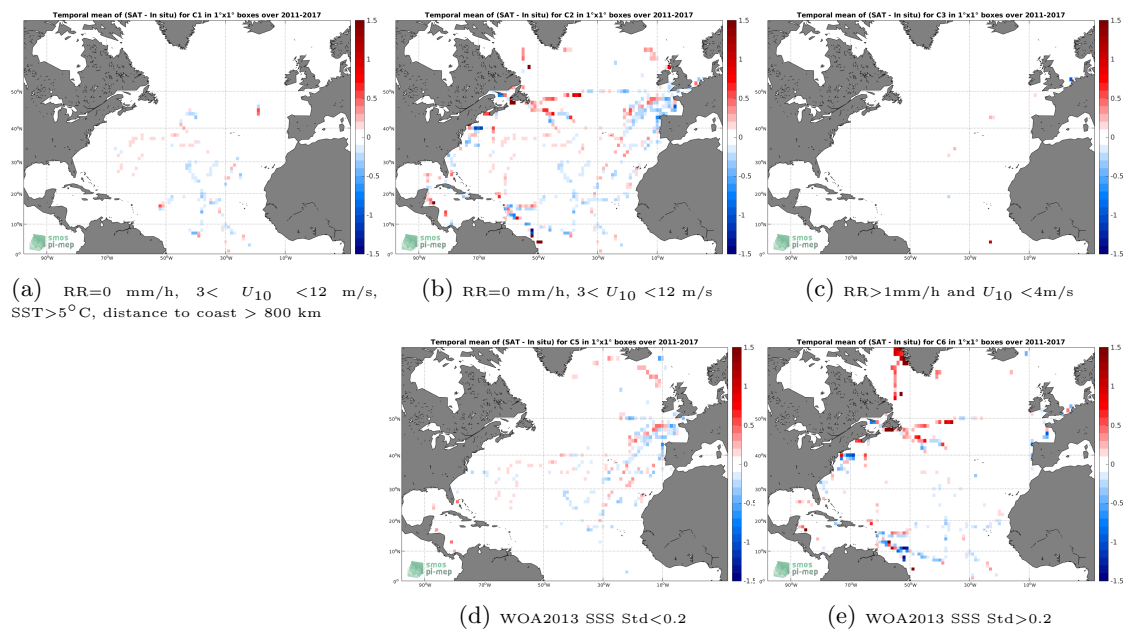
Figure 12: Temporal mean gridded over spatial boxes of size 1^\circ \times 1^\circ of \Delta SSS (CCI L4 Merged-OI v1.8 - 7-day running (ESA) - TSG-GOSUD-Sailing-ship) for 5 different subdatasets corresponding to:RR=0 mm/h, 3 < U_{10} < 12 m/s, SST >5^\circ\text{C} , distance to coast > 800 km (a), RR=0 mm/h, 3 < U_{10} < 12 m/s (b), RR >1 mm/h and U_{10} < 4 m/s (c), WOA2013 SSS Std <0.2 (d), WOA2013 SSS Std >0.2 (e).
