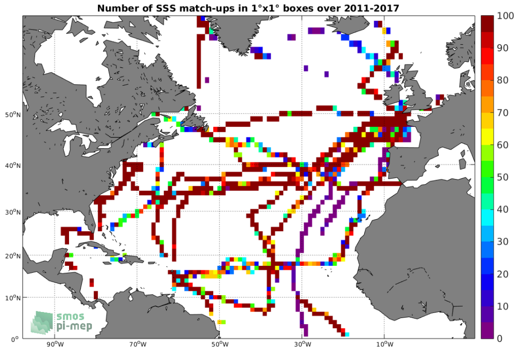
Figure 4: Number of SSS match-ups between TSG-GOSUD-Sailing-ship SSS and the CCI L4 Merged-OI v1.8 - 7-day running (ESA) SSS product for the North Atlantic Ocean Pi-MEP region over 1^\circ \times 1^\circ boxes and for the full satellite product period.
