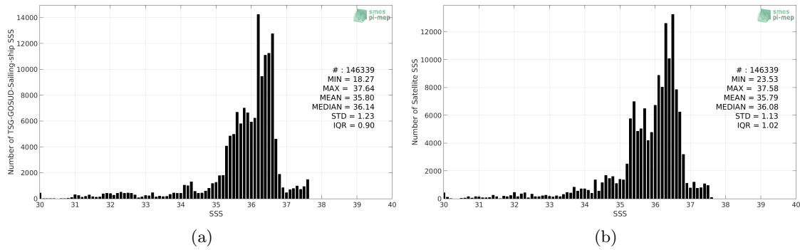
Figure 2: Histograms of SSS from TSG-GOSUD-Sailing-ship (a) and CCI-L4-ESA-MERGED-OI-V1.8-7DAY-RUNNING (b) considering all match-up pairs per bins of 0.1 over the North Atlantic Ocean Pi-MEP region and for the full satellite product period.
