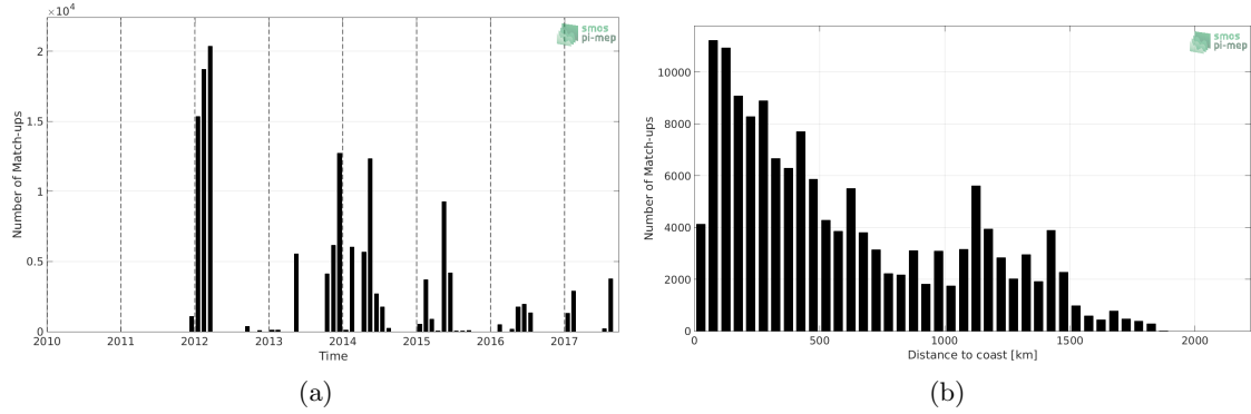
Figure 1: Number of match-ups between TSG-GOSUD-Sailing-ship and CCI-L4-ESA-MERGED-OI-V1.8-7DAY-RUNNING SSS as a function of time (a) and as function of the distance to coast (b) over the North Atlantic Ocean Pi-MEP region and for the full satellite product period.
