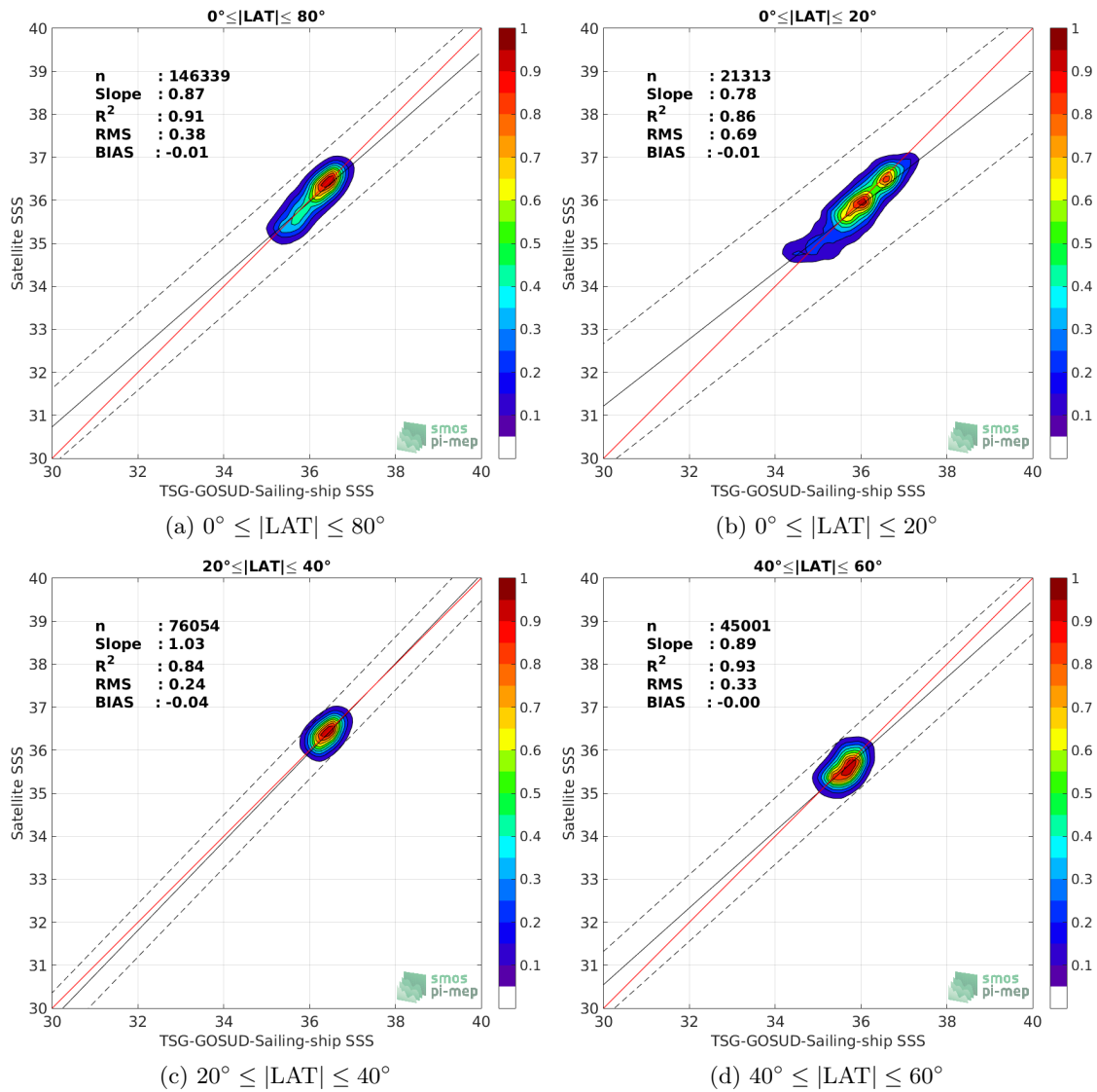
Figure 9: Contour maps of the concentration of CCI-L4-ESA-MERGED-OI-V1.8-7DAY-RUNNING SSS (y-axis) versus TSG-GOSUD-Sailing-ship SSS (x-axis) at match-up pairs for different latitude bands. For each plot, the red line shows x=y . The black thin and dashed lines indicate a linear fit through the data cloud and the \pm 95\% confidence levels, respectively. The number match-up pairs n , the slope and R^2 coefficient of the linear fit, the root mean square (RMS) and the mean bias between satellite and in situ data are indicated for each latitude band in each plots.
