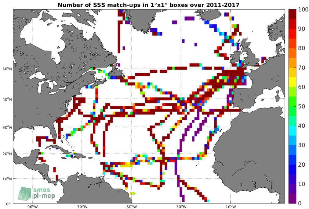
Figure 4: Number of SSS match-ups between TSG-GOSUD-Sailing-ship SSS and the CCI-L4-ESA-MERGED-OI-V1.8-7DAY-RUNNING SSS product for the North Atlantic Ocean Pi-MEP region over 1°x1° boxes and for the full satellite product period.
