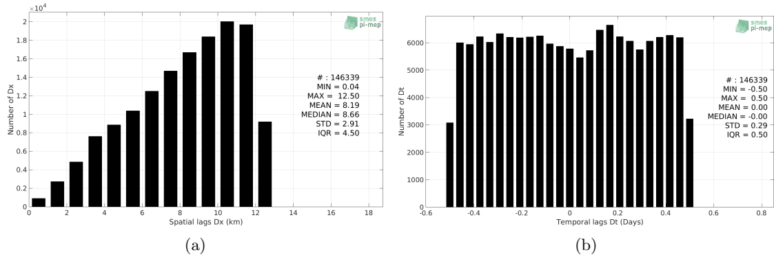
Figure 5: Histograms of the spatial (a) and temporal (b) lags between the time of the TSG-GOSUD-Sailing-ship measurements and the date of the corresponding CCI-L4-ESA-MERGED-OI-V1.8-7DAY-RUNNING SSS product.
