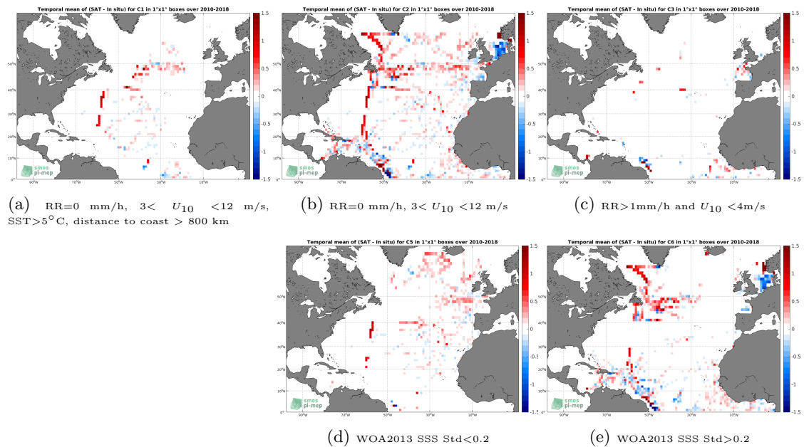
Figure 12: Temporal mean gridded over spatial boxes of size 1^\circ \times 1^\circ of \Delta SSS (CCI L4 Merged-OI v1.8 - 7-day running (ESA) - TSG-GOSUD-Research-vessel) for 5 different subdatasets corresponding to: RR=0 mm/h, 3 < U_{10} < 12 m/s, SST > 5°C, distance to coast > 800 km (a), RR=0 mm/h, 3 < U_{10} < 12 m/s (b), RR > 1mm/h and U_{10} < 4 m/s (c), WOA2013 SSS Std < 0.2 (d), WOA2013 SSS Std > 0.2 (e).
