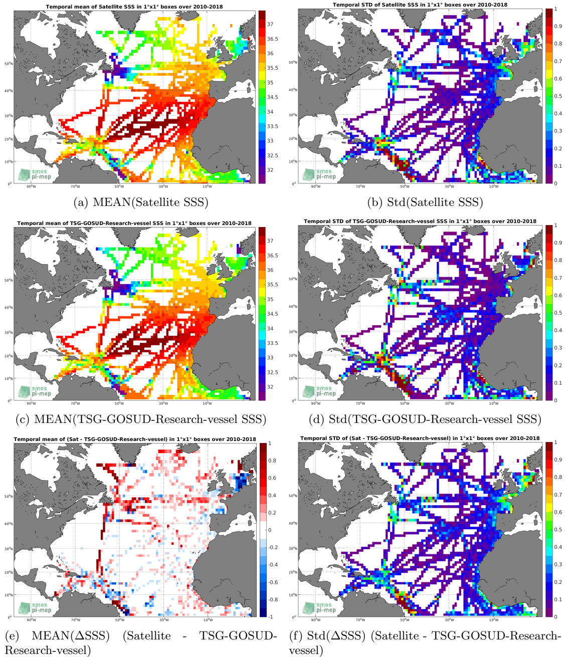
Figure 6: Temporal mean (left) and Std (right) of SSS from CCI L4 Merged-OI v1.8 - 7-day running (ESA) (top), TSG-GOSUD-Research-vessel (middle), and of \Delta SSS (Satellite - TSG-GOSUD-Research-vessel). Only match-up pairs are used to generate these maps.
