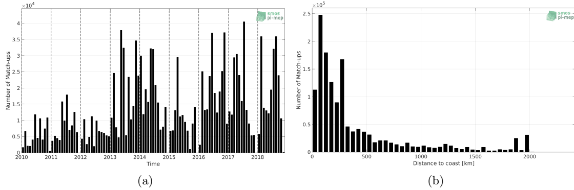
Figure 1: Number of match-ups between TSG-GOSUD-Research-vessel and CCI L4 Merged-OI v1.8 - 7-day running (ESA) SSS as a function of time (a) and as function of the distance to coast (b) over the North Atlantic Ocean Pi-MEP region and for the full satellite product period.
