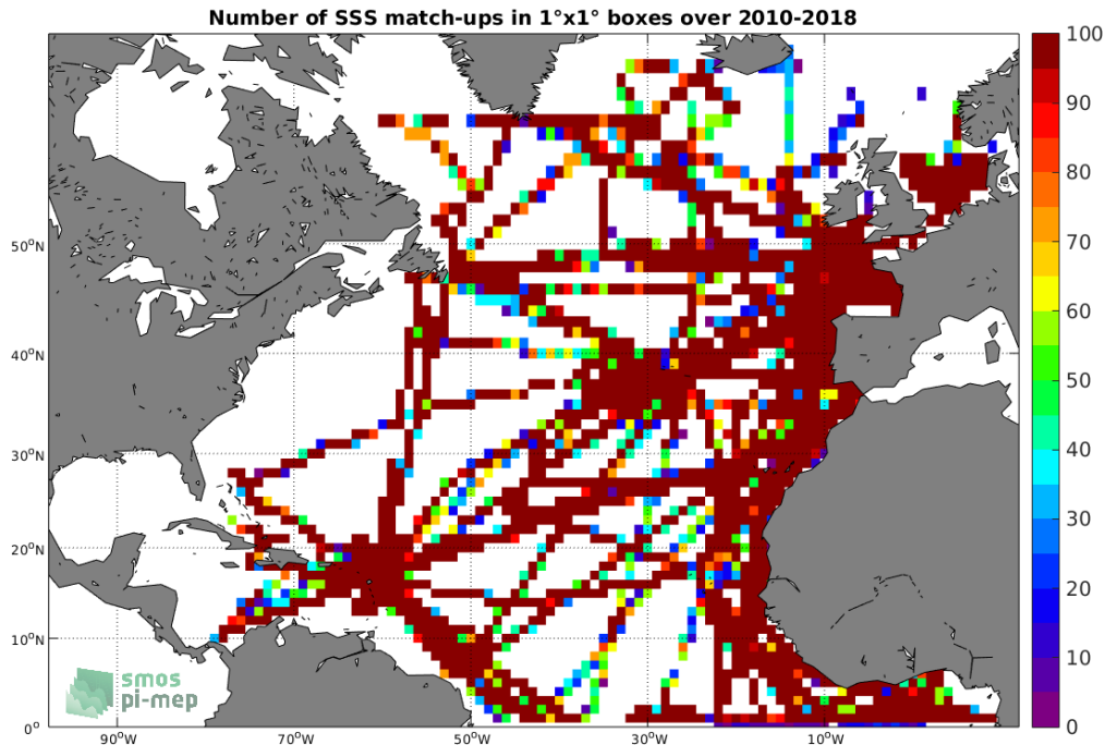
Figure 4: Number of SSS match-ups between TSG-GOSUD-Research-vessel SSS and the CCI L4 Merged-OI v1.8 - 7-day running (ESA) SSS product for the North Atlantic Ocean Pi-MEP region over 1°x1° boxes and for the full satellite product period.
