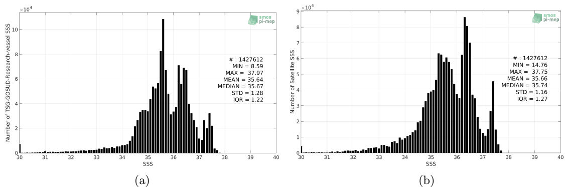
Figure 2: Histograms of SSS from TSG-GOSUD-Research-vessel (a) and CCI L4 Merged-OI v1.8 - 7-day running (ESA) (b) considering all match-up pairs per bins of 0.1 over the North Atlantic Ocean Pi-MEP region and for the full satellite product period.
