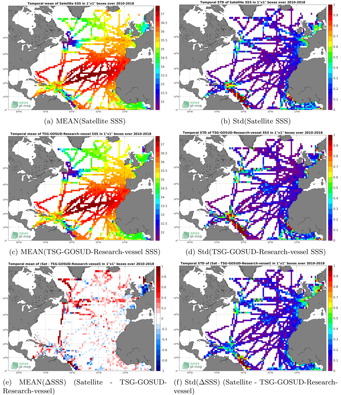
Figure 6: Temporal mean (left) and Std (right) of SSS from CCI-L4-ESA-MERGED-OI-V1.8-7DAY-RUNNING (top), TSG-GOSUD-Research-vessel (middle), and of \Delta SSS (Satellite - TSG-GOSUD-Research-vessel). Only match-up pairs are used to generate these maps.
