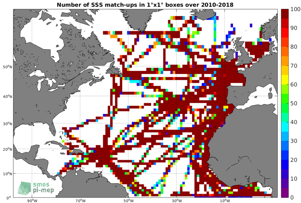
Figure 4: Number of SSS match-ups between TSG-GOSUD-Research-vessel SSS and the CCI-L4-ESA-MERGED-OI-V1.8-7DAY-RUNNING SSS product for the North Atlantic Ocean Pi-MEP region over 1^\circ \times 1^\circ boxes and for the full satellite product period.
