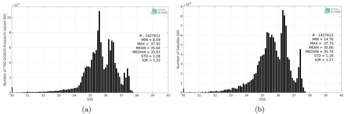
Figure 2: Histograms of SSS from TSG-GOSUD-Research-vessel (a) and CCI-L4-ESA-MERGED-OI-V1.8-7DAY-RUNNING (b) considering all match-up pairs per bins of 0.1 over the North Atlantic Ocean Pi-MEP region and for the full satellite product period.
