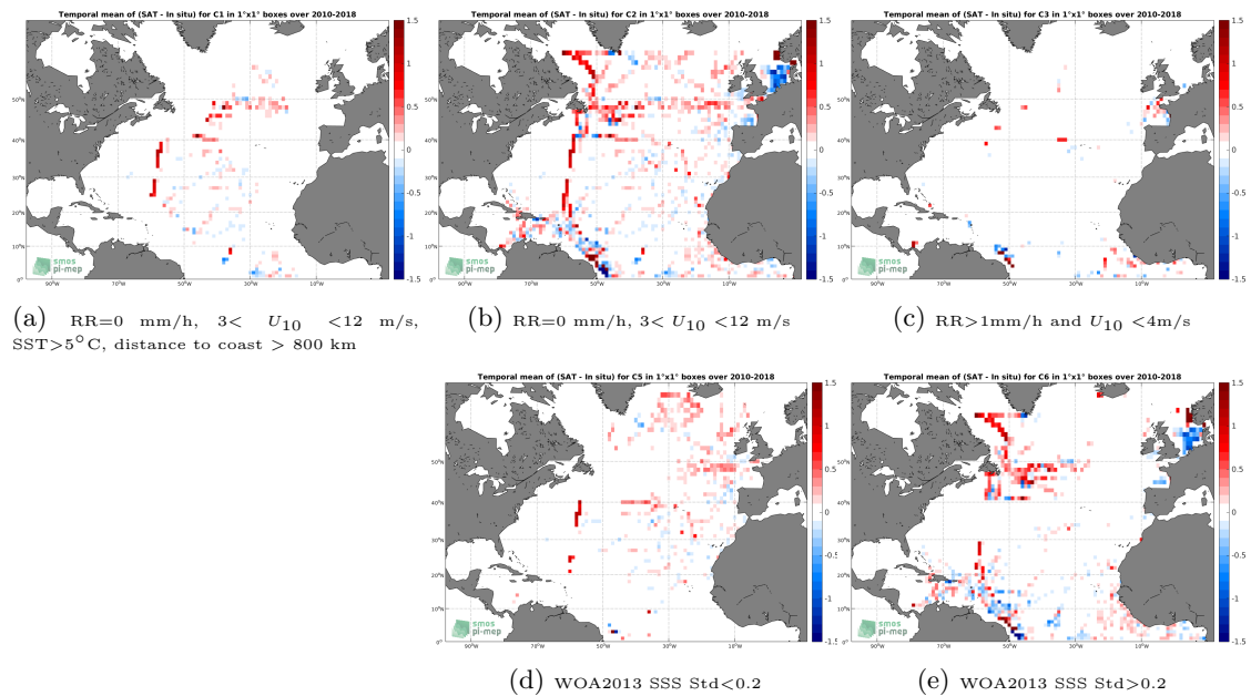
Figure 12: Temporal mean gridded over spatial boxes of size 1^\circ \times 1^\circ of \Delta SSS (CCI-L4-ESA-MERGED-OI-V1.8-7DAY-RUNNING - TSG-GOSUD-Research-vessel) for 5 different sub-datasets corresponding to:RR=0 mm/h, 3 < U_{10} < 12 m/s, SST >5^\circ\text{C} , distance to coast > 800 km (a), RR=0 mm/h, 3 < U_{10} < 12 m/s (b), RR >1 mm/h and U_{10} < 4 m/s (c), WOA2013 SSS Std <0.2 (d), WOA2013 SSS Std >0.2 (e).
