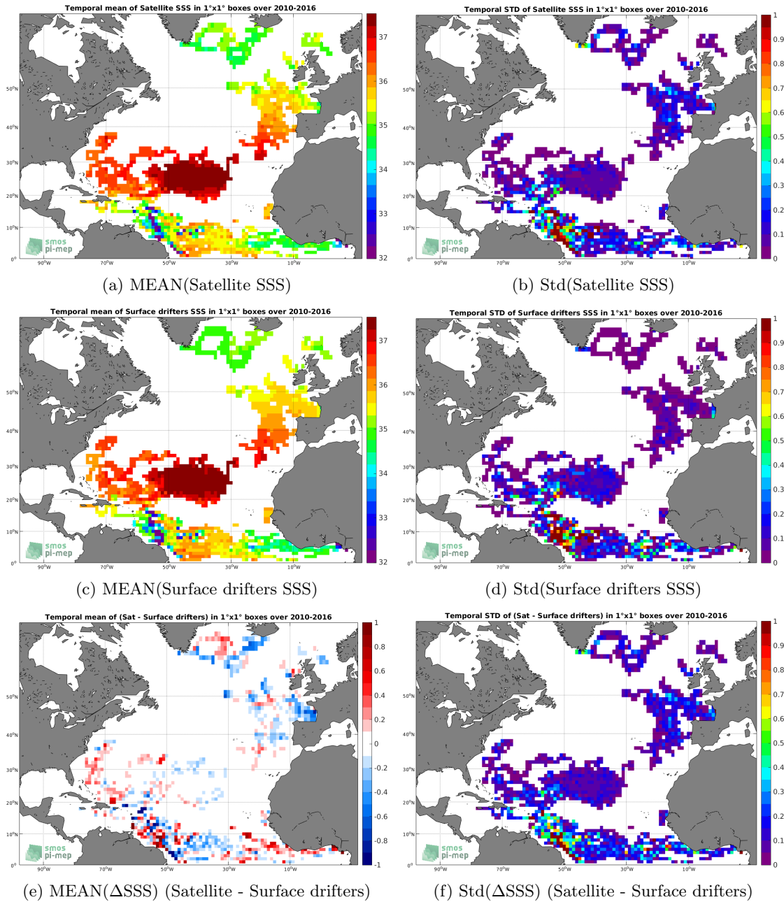
Figure 5: Temporal mean (left) and Std (right) of SSS from CCI L4 Merged-OI v1.8 - 7-day running (ESA) (top), Surface drifters (middle), and of \Delta SSS (Satellite - Surface drifters). Only match-up pairs are used to generate these maps.
