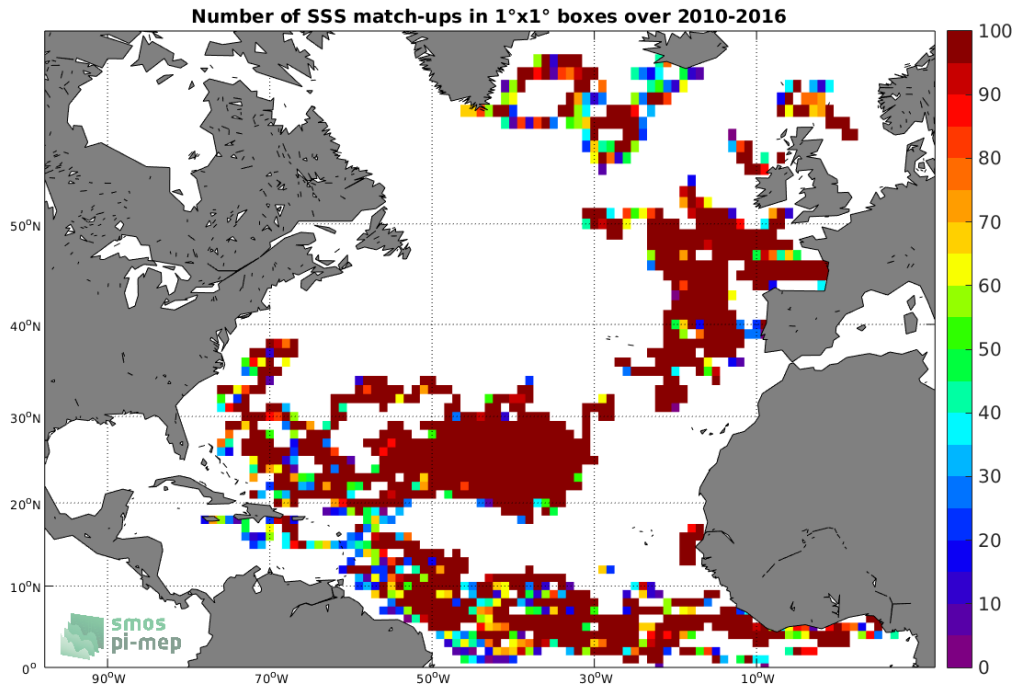
Figure 3: Number of SSS match-ups between Surface drifters SSS and the CCI L4 Merged-OI v1.8 - 7-day running (ESA) SSS product for the North Atlantic Ocean Pi-MEP region over 1^{\circ} \times 1^{\circ} boxes and for the full satellite product period.
