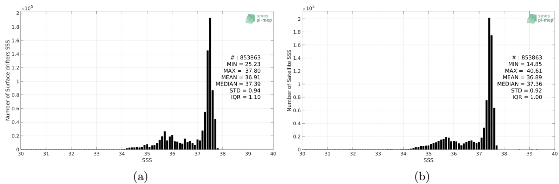
Figure 2: Histograms of SSS from Surface drifters (a) and CCI L4 Merged-OI v1.8 - 7-day running (ESA) (b) considering all match-up pairs per bins of 0.1 over the North Atlantic Ocean Pi-MEP region and for the full satellite product period.
