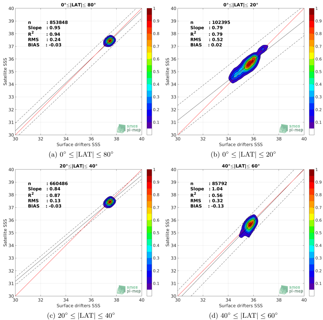
Figure 8: Contour maps of the concentration of CCI-L4-ESA-MERGED-OI-V1.8-7DAY-RUNNING SSS (y-axis) versus Surface drifters SSS (x-axis) at match-up pairs for different latitude bands. For each plot, the red line shows x=y . The black thin and dashed lines indicate a linear fit through the data cloud and the \pm 95\% confidence levels, respectively. The number of match-up pairs n , the slope and R^2 coefficient of the linear fit, the root mean square (RMS) and the mean bias between satellite and in situ data are indicated for each latitude band in each plot.
