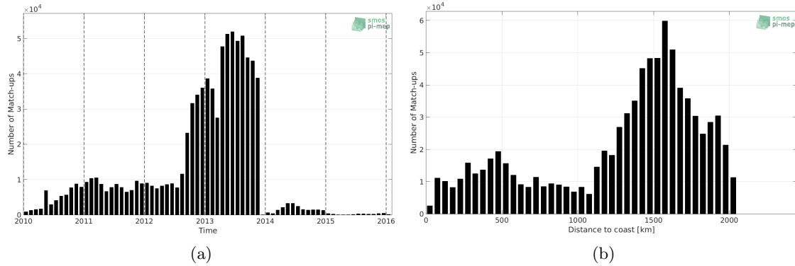
Figure 1: Number of match-ups between Surface drifters and CCI-L4-ESA-MERGED-OI-V1.8-7DAY-RUNNING SSS as a function of time (a) and as function of the distance to coast (b) over the North Atlantic Ocean Pi-MEP region and for the full satellite product period.
