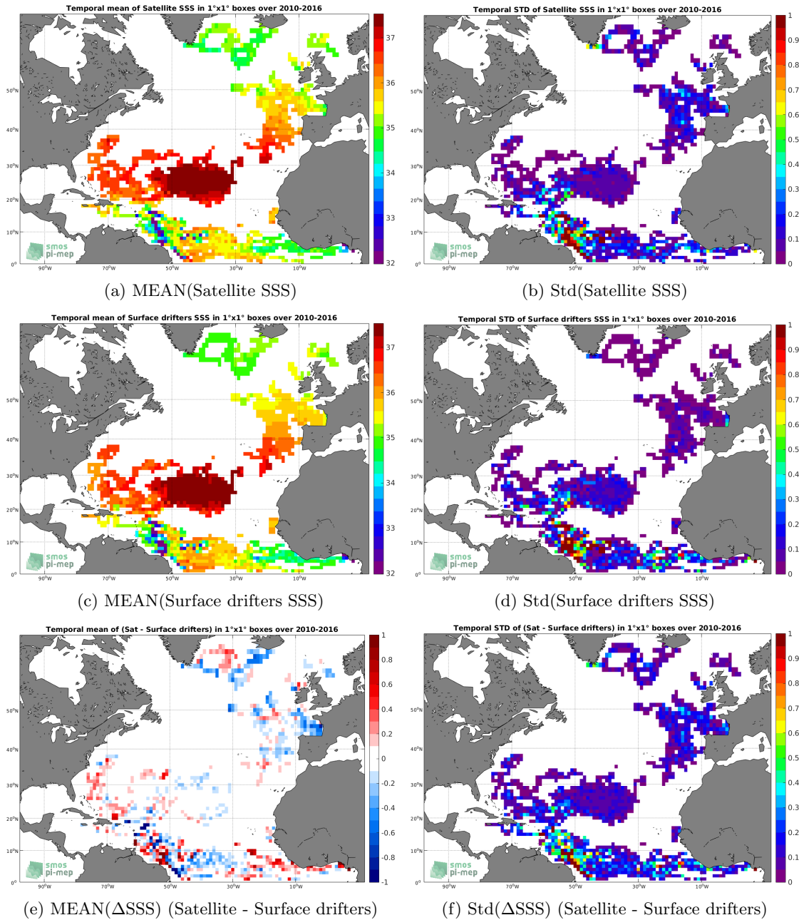
Figure 5: Temporal mean (left) and Std (right) of SSS from CCI-L4-ESA-MERGED-OI-V1.8-7DAY-RUNNING (top), Surface drifters (middle), and of \Delta SSS (Satellite - Surface drifters). Only match-up pairs are used to generate these maps.
