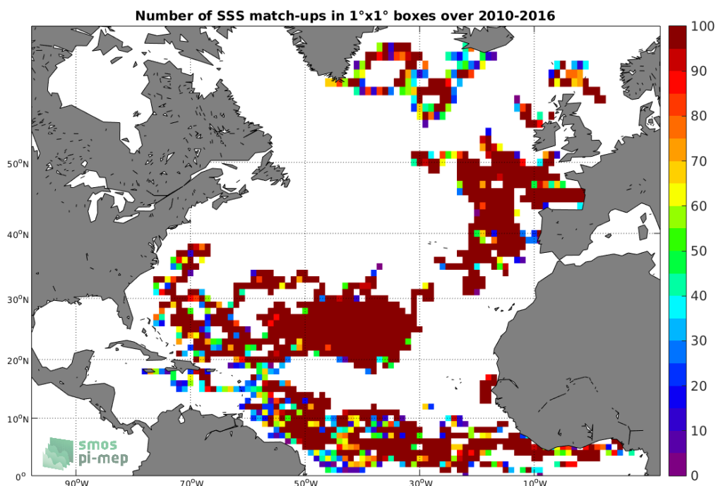
Figure 3: Number of SSS match-ups between Surface drifters SSS and the CCI-L4-ESA-MERGED-OI-V1.8-7DAY-RUNNING SSS product for the North Atlantic Ocean Pi-MEP region over 1°x1° boxes and for the full satellite product period.
