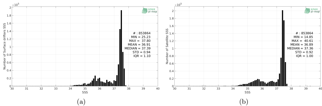
Figure 2: Histograms of SSS from Surface drifters (a) and CCI-L4-ESA-MERGED-OI-V1.8-7DAY-RUNNING (b) considering all match-up pairs per bins of 0.1 over the North Atlantic Ocean Pi-MEP region and for the full satellite product period.
