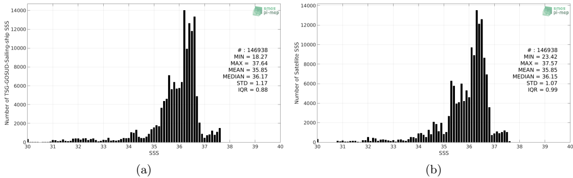
Figure 2: Histograms of SSS from TSG-GOSUD-Sailing-ship (a) and CCI-L4-ESA-MERGED-OI-V1.8-30DAY-RUNNING (b) considering all match-up pairs per bins of 0.1 over the North Atlantic Ocean Pi-MEP region and for the full satellite product period.
