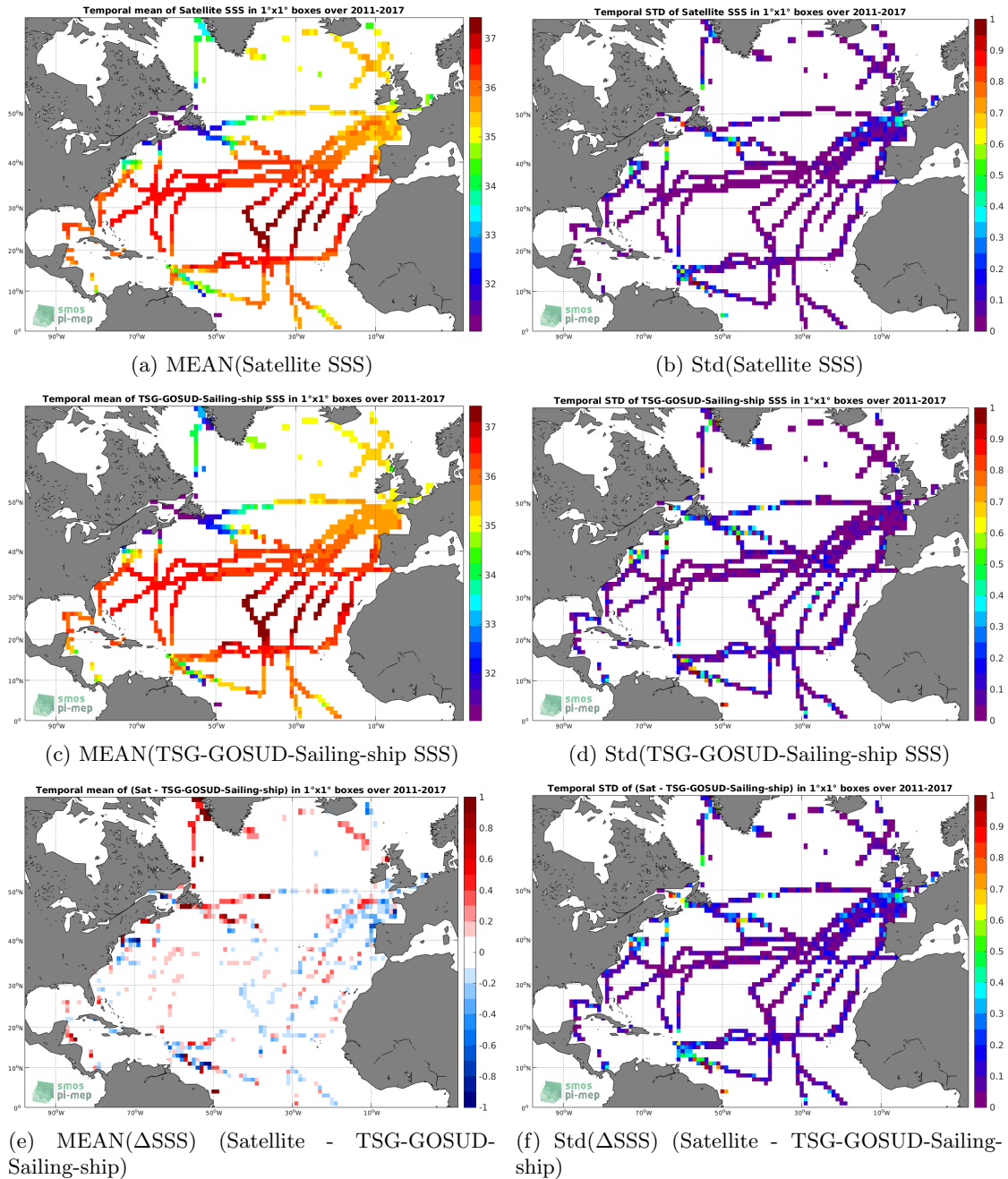
Figure 6: Temporal mean (left) and Std (right) of SSS from CCI-L4-ESA-MERGED-OI-V1.8-30DAY-RUNNING (top), TSG-GOSUD-Sailing-ship (middle), and of \Delta SSS (Satellite - TSG-GOSUD-Sailing-ship). Only match-up pairs are used to generate these maps.
