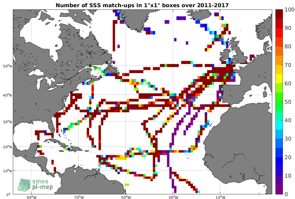
Figure 4: Number of SSS match-ups between TSG-GOSUD-Sailing-ship SSS and the CCI-L4-ESA-MERGED-OI-V1.8-30DAY-RUNNING SSS product for the North Atlantic Ocean Pi-MEP region over 1^\circ \times 1^\circ boxes and for the full satellite product period.
