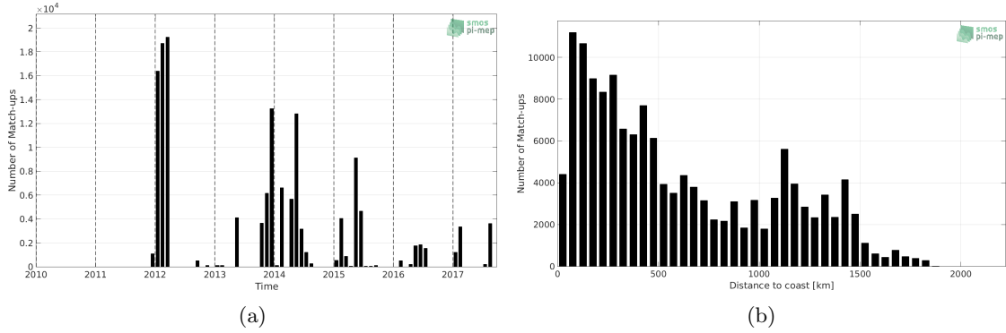
Figure 1: Number of match-ups between TSG-GOSUD-Sailing-ship and CCI-L4-ESA-MERGED-OI-V1.8-30DAY-RUNNING SSS as a function of time (a) and as function of the distance to coast (b) over the North Atlantic Ocean Pi-MEP region and for the full satellite product period.
