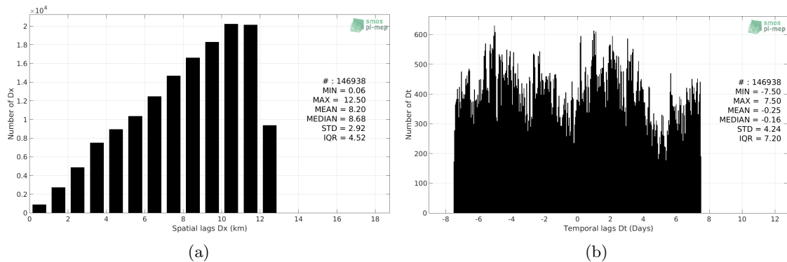
Figure 5: Histograms of the spatial (a) and temporal (b) lags between the time of the TSG-GOSUD-Sailing-ship measurements and the date of the corresponding CCI-L4-ESA-MERGED-OI-V1.8-30DAY-RUNNING SSS product.
