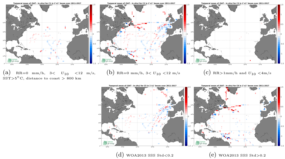
Figure 12: Temporal mean gridded over spatial boxes of size 1^\circ \times 1^\circ of \Delta SSS (CCI-L4-ESAMERGED-OI-V1.8-30DAY-RUNNING - TSG-GOSUD-Sailing-ship) for 5 different subdatasets corresponding to:RR=0 mm/h, 3 < U_{10} < 12 m/s, SST >5^\circ\text{C} , distance to coast > 800 km (a), RR=0 mm/h, 3 < U_{10} < 12 m/s (b), RR >1 mm/h and U_{10} < 4 m/s (c), WOA2013 SSS Std <0.2 (d), WOA2013 SSS Std >0.2 (e).
