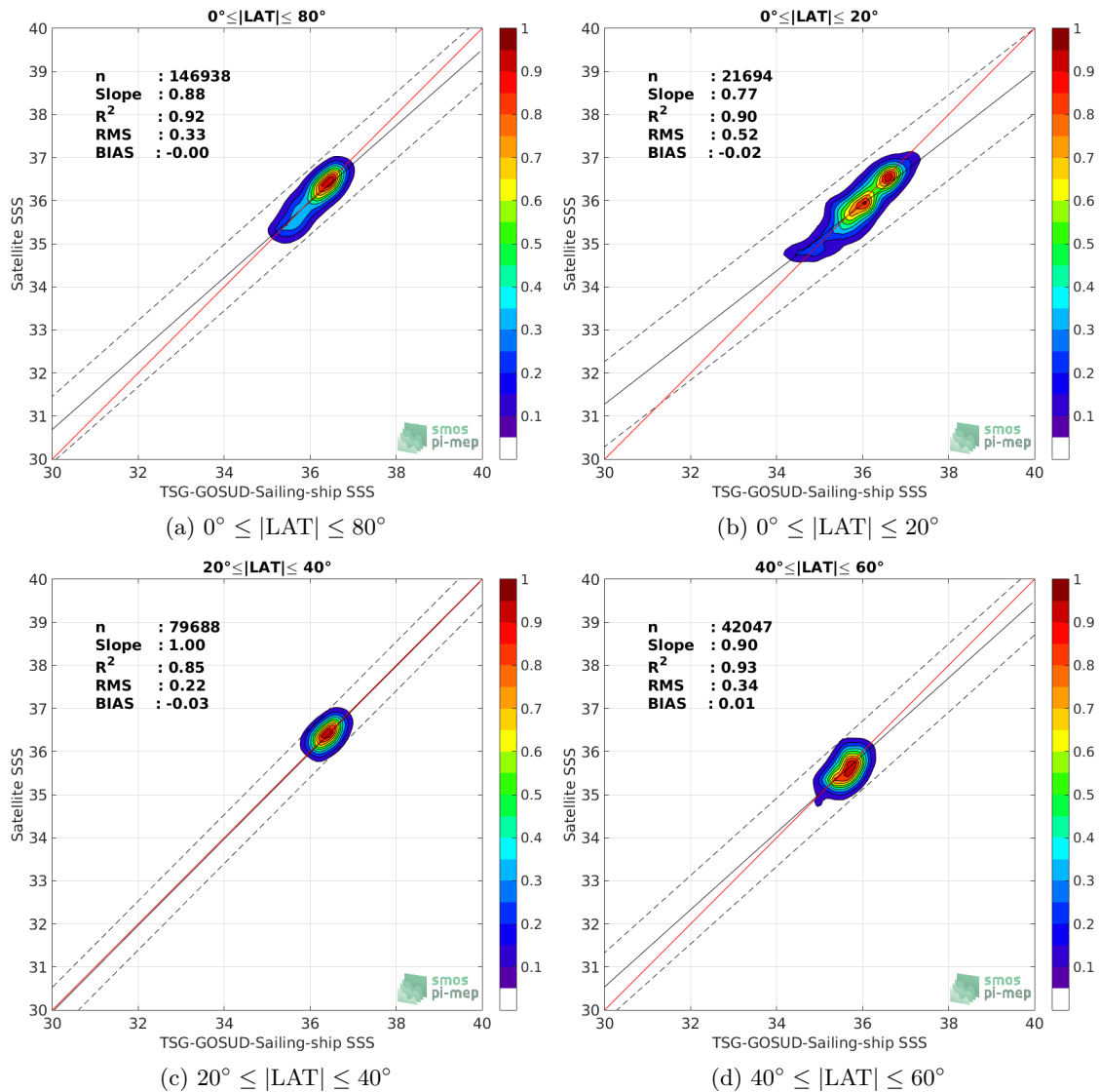
Figure 9: Contour maps of the concentration of CCI-L4-ESA-MERGED-OI-V1.8-30DAY-RUNNING SSS (y-axis) versus TSG-GOSUD-Sailing-ship SSS (x-axis) at match-up pairs for different latitude bands. For each plot, the red line shows x=y . The black thin and dashed lines indicate a linear fit through the data cloud and the \pm 95\% confidence levels, respectively. The number match-up pairs n , the slope and R^2 coefficient of the linear fit, the root mean square (RMS) and the mean bias between satellite and in situ data are indicated for each latitude band in each plots.
