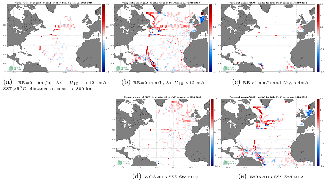
Figure 12: Temporal mean gridded over spatial boxes of size 1^\circ \times 1^\circ of \Delta SSS (CCI-L4-ESA-MERGED-OI-V1.8-30DAY-RUNNING - TSG-GOSUD-Research-vessel) for 5 different sub-datasets corresponding to:RR=0 mm/h, 3 < U_{10} < 12 m/s, SST >5^\circ C, distance to coast > 800 km (a), RR=0 mm/h, 3 < U_{10} < 12 m/s (b), RR >1 mm/h and U_{10} < 4 m/s (c), WOA2013 SSS Std <0.2 (d), WOA2013 SSS Std >0.2 (e).
