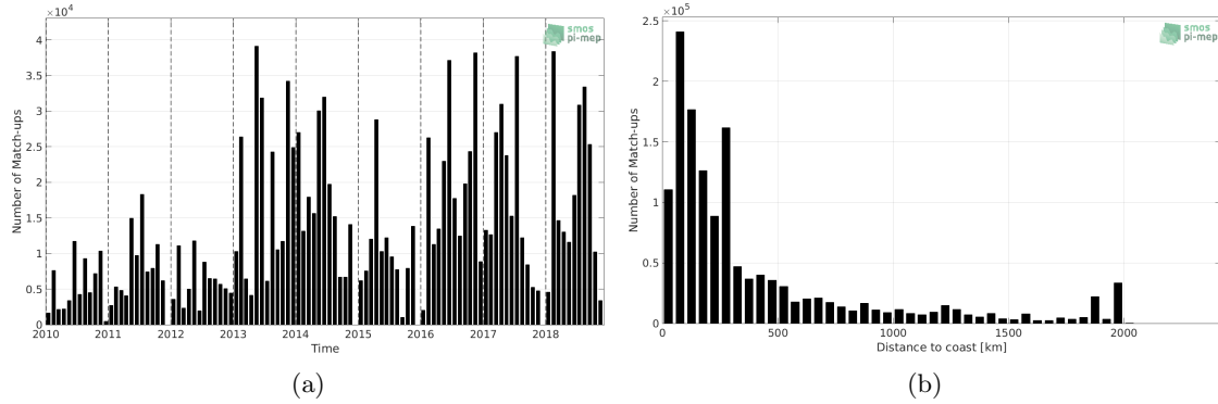
Figure 1: Number of match-ups between TSG-GOSUD-Research-vessel and CCI-L4-ESA-MERGED-OI-V1.8-30DAY-RUNNING SSS as a function of time (a) and as function of the distance to coast (b) over the North Atlantic Ocean Pi-MEP region and for the full satellite product period.
