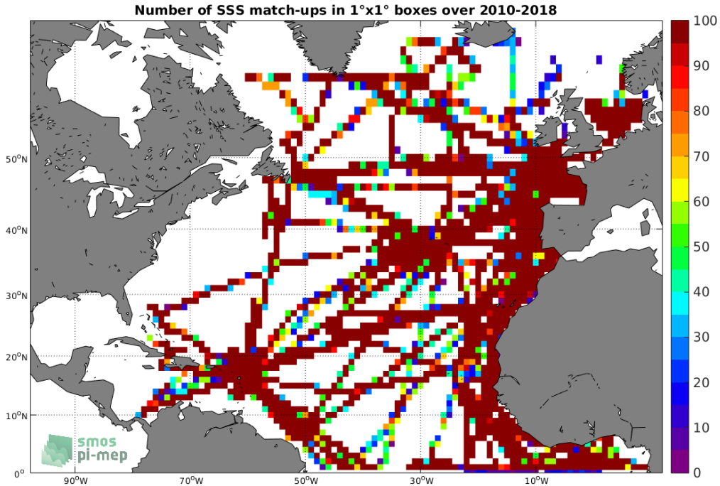
Figure 4: Number of SSS match-ups between TSG-GOSUD-Research-vessel SSS and the CCI-L4-ESA-MERGED-OI-V1.8-30DAY-RUNNING SSS product for the North Atlantic Ocean Pi-MEP region over 1^\circ \times 1^\circ boxes and for the full satellite product period.
