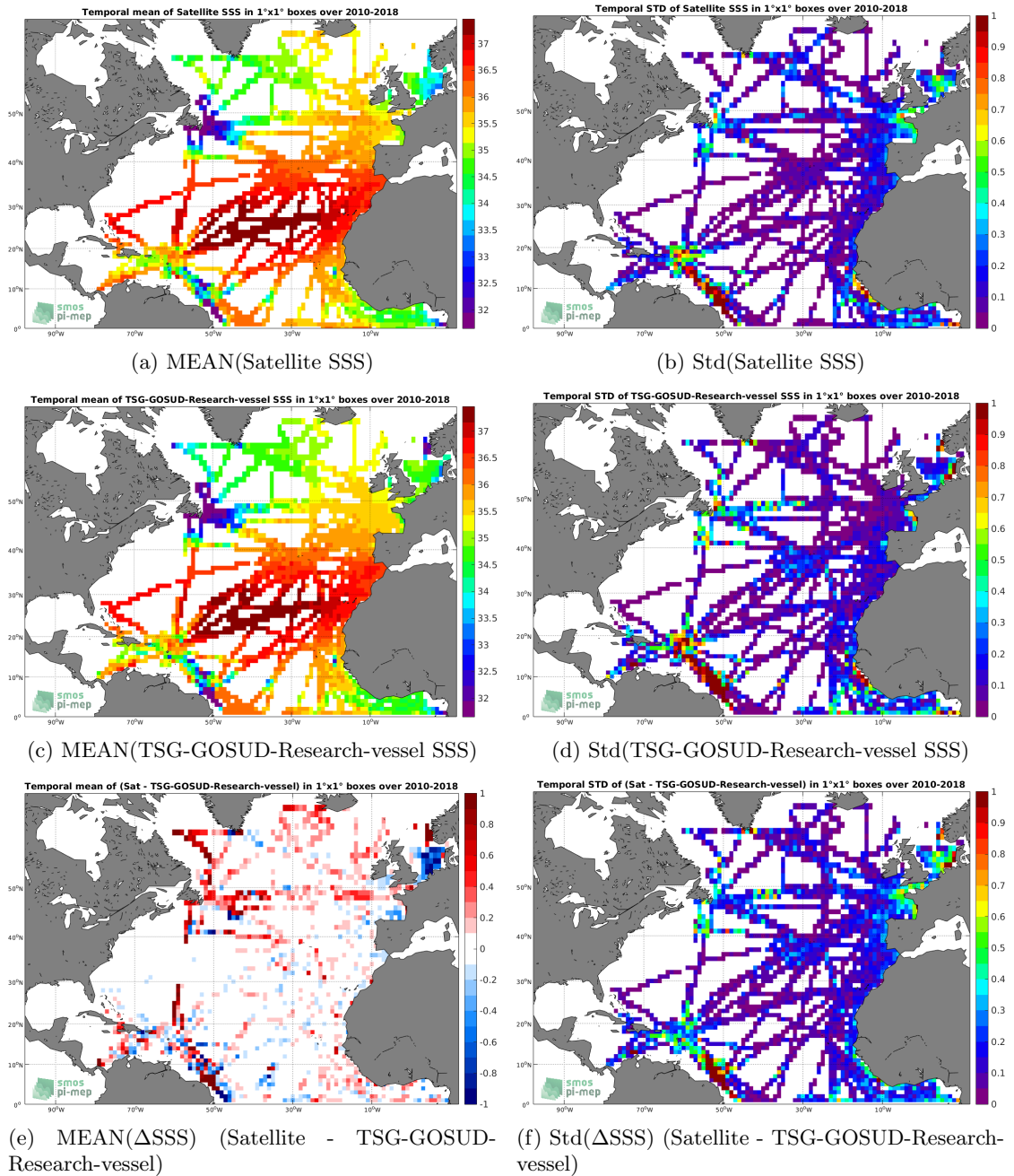
Figure 6: Temporal mean (left) and Std (right) of SSS from CCI-L4-ESA-MERGED-OI-V1.8-30DAY-RUNNING (top), TSG-GOSUD-Research-vessel (middle), and of \Delta SSS (Satellite - TSG-GOSUD-Research-vessel). Only match-up pairs are used to generate these maps.
