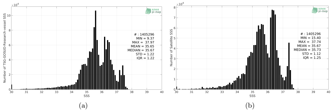
Figure 2: Histograms of SSS from TSG-GOSUD-Research-vessel (a) and CCI-L4-ESA-MERGED-OI-V1.8-30DAY-RUNNING (b) considering all match-up pairs per bins of 0.1 over the North Atlantic Ocean Pi-MEP region and for the full satellite product period.
