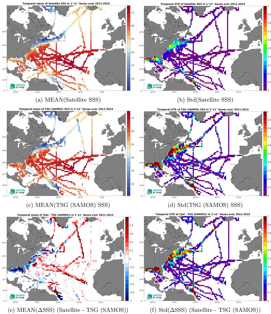
Figure 7: Temporal mean (left) and Std (right) of SSS from Aquarius SSS L4 OI v5 - Weekly (IPRC) (top), TSG (SAMOS) (middle), and of \Delta SSS (Satellite - TSG (SAMOS)). Only match-up pairs are used to generate these maps.
