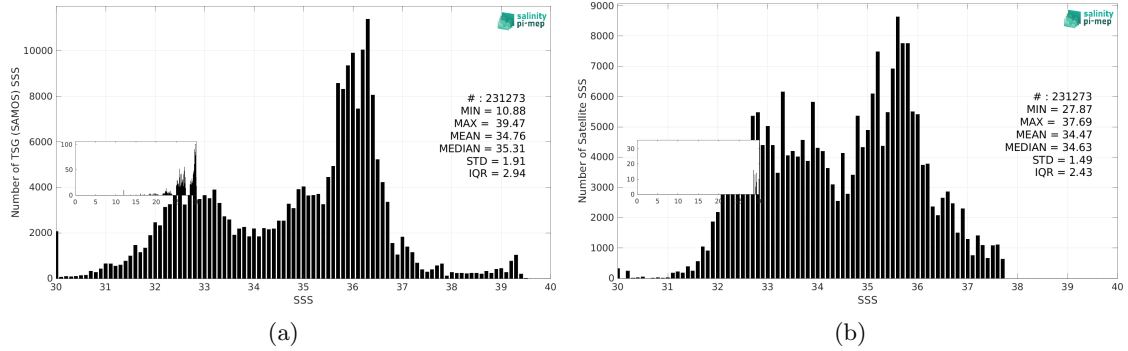
Figure 3: Histograms of SSS from TSG (SAMOS) (a) and Aquarius SSS L4 OI v5 - Weekly (IPRC) (b) considering all match-up pairs per bins of 0.1 over the North Atlantic Ocean Pi-MEP region and for the full satellite product period.
