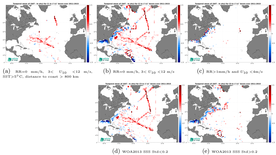
Figure 14: Temporal mean gridded over spatial boxes of size 1^\circ \times 1^\circ of \Delta\text{SSS} (Aquarius SSS L4 OI v5 - Weekly (IPRC) - TSG (SAMOS)) for 5 different subdatasets corresponding to:RR=0 mm/h, 3 < U_{10} < 12 m/s, SST>5°C, distance to coast > 800 km (a), RR=0 mm/h, 3 < U_{10} < 12 m/s (b), RR>1mm/h and U_{10} < 4 m/s (c), WOA2013 SSS Std<0.2 (d), WOA2013 SSS Std>0.2 (e).
