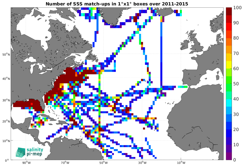
Figure 5: Number of SSS match-ups between TSG (SAMOS) SSS and the Aquarius SSS L4 OI v5 - Weekly (IPRC) SSS product for the North Atlantic Ocean Pi-MEP region over 1^\circ \times 1^\circ boxes and for the full satellite product period.
