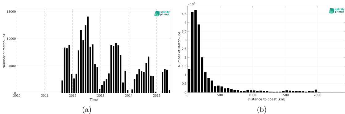
Figure 2: Number of match-ups between TSG (SAMOS) and Aquarius SSS L4 OI v5 - Weekly (IPRC) SSS as a function of time (a) and as function of the distance to coast (b) over the North Atlantic Ocean Pi-MEP region and for the full satellite product period.
